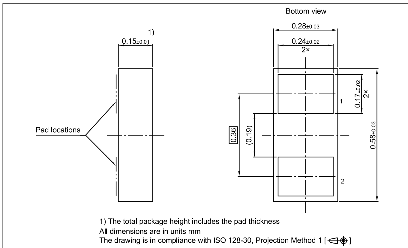
Figure 14 WLL-2-3 package
