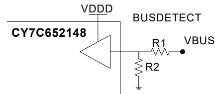
Figure 11. GPIO VBUS Detection, VBUS > VDDD
