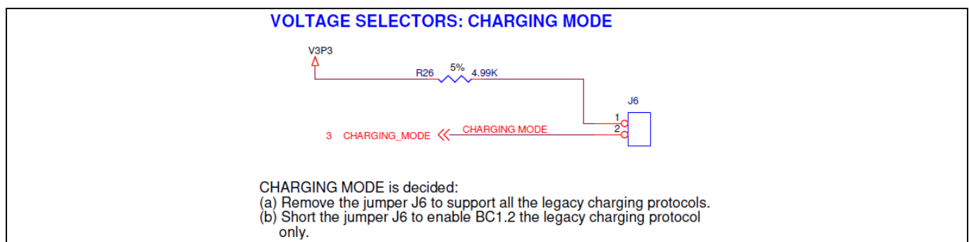
Figure 11 Legacy charging mode selection jumper circuit
