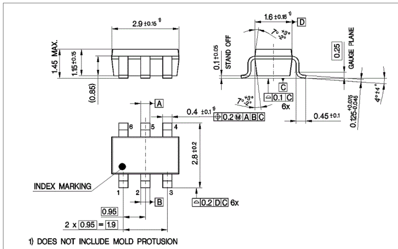
Figure 5 Package Drawings
