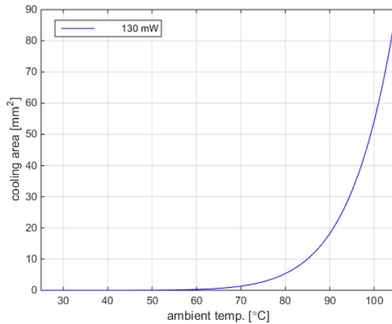
Figure 3 Cooling area over ambient temperature CDM10V-4
