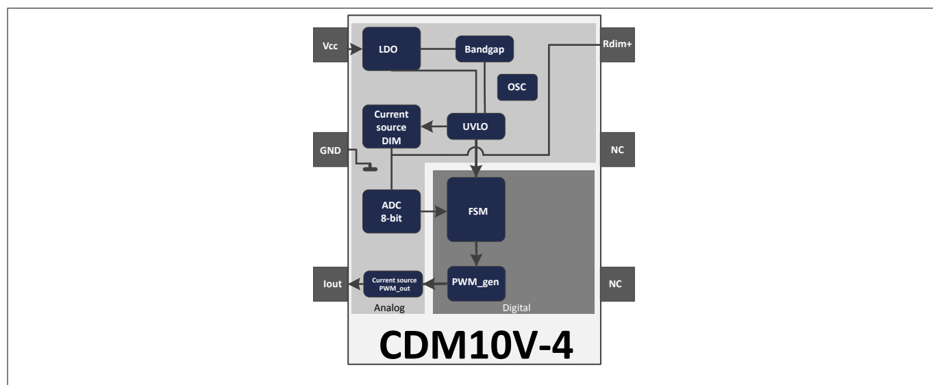
Figure 1 Block Diagram of the CDM10V-4
