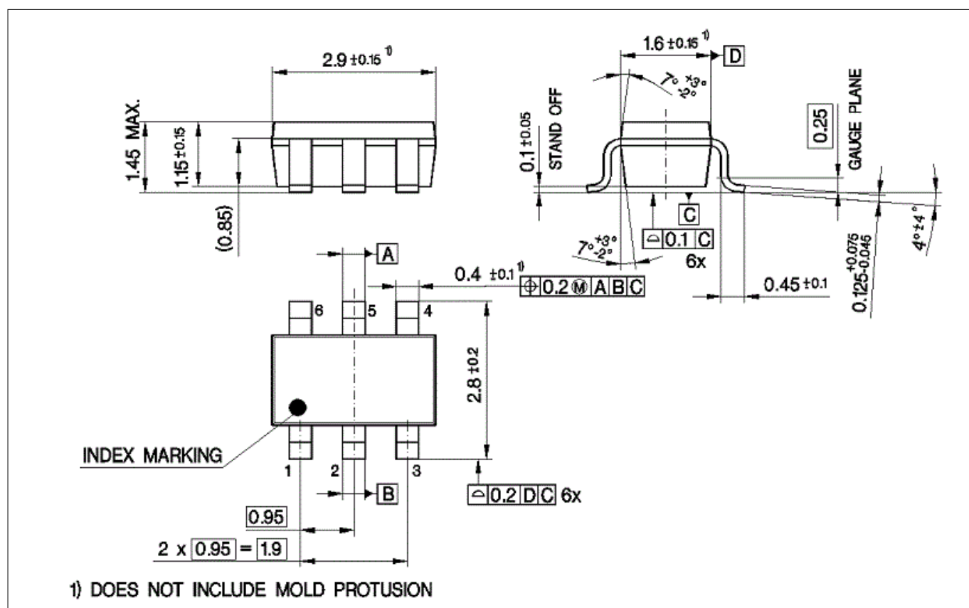
Figure 5 Package Drawings
