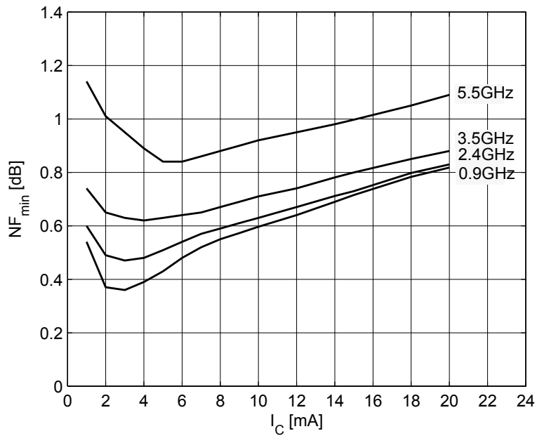
Figure 20 Noise figure NF_{min} = f(I_C) , V_{CE} = 2.5 \text{ V} , Z_S = Z_{S,opt} , f = \text{parameter}
