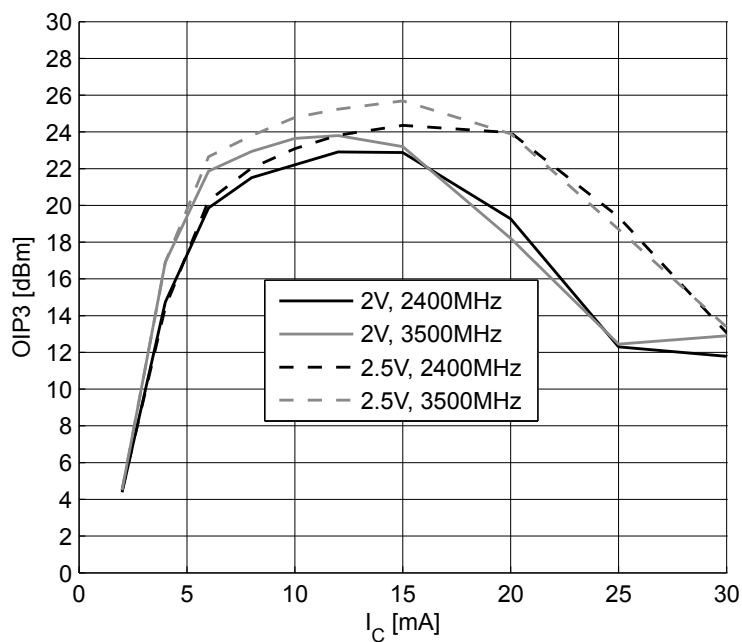
Figure 13 3rd order intercept point at output OIP_3 = f(I_C) , Z_S = Z_L = 50 \Omega , V_{CE} , f = parameter
