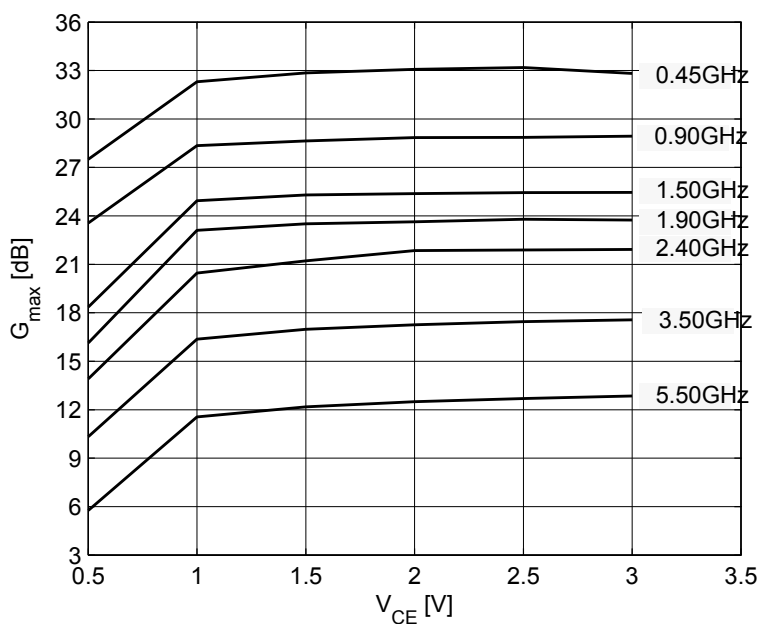
Figure 12 Maximum power gain G_{max} = f(V_{CE}) , I_C = 15 mA, f = parameter
