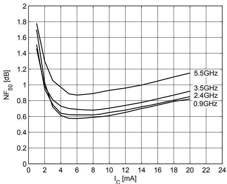
Figure 21 Noise figure NF_{50} = f(I_C) , V_{CE} = 2.5 \text{ V} , Z_S = 50 \Omega , f = \text{parameter}
