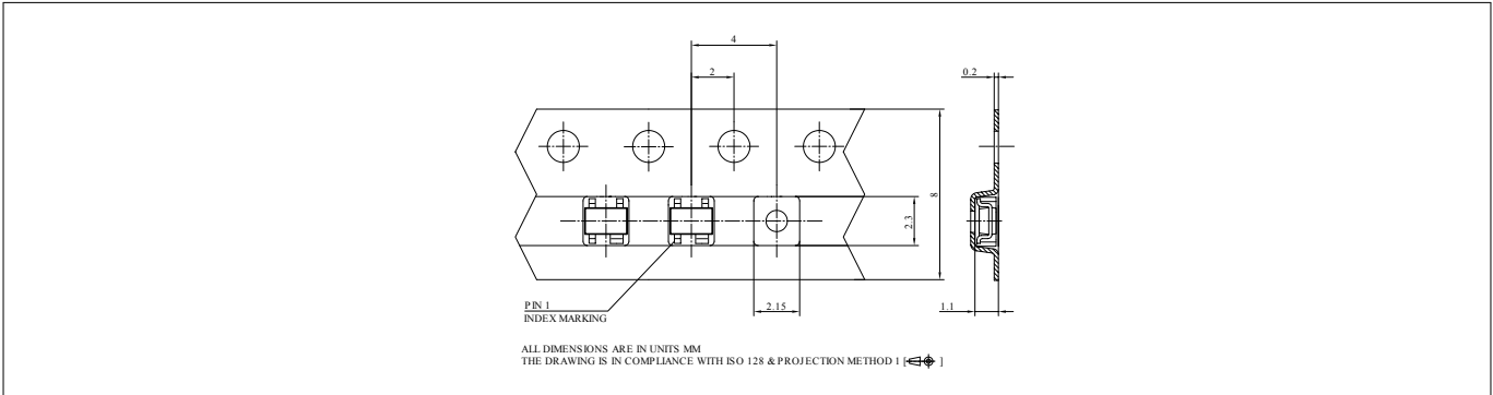
Figure 25 Tape dimensions
