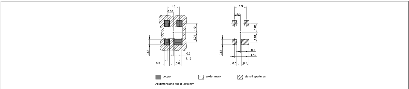
Figure 23 Foot print
