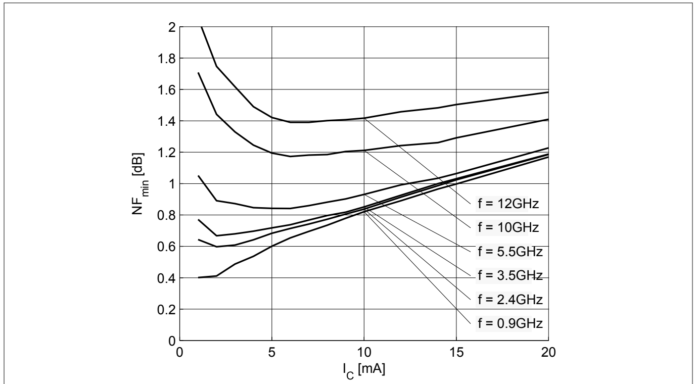
Figure 20 Noise figure NF_{min} = f(I_C) , V_{CE} = 1.8 \text{ V} , Z_S = Z_{opt} , f = \text{parameter in GHz}
