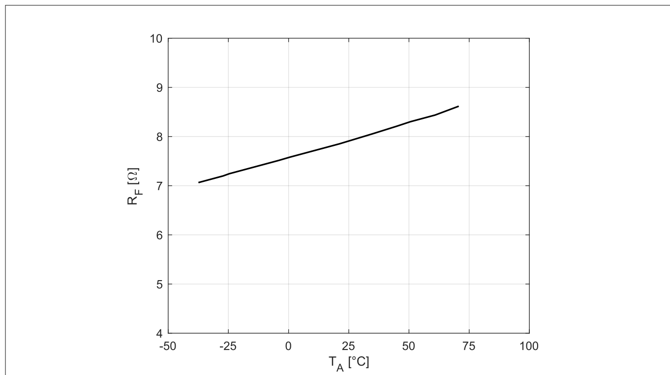
Figure 5 Differential forward resistance R_F vs. ambient temperature T_A between forward currents I_F = 10 \text{ mA} and 50 \text{ mA}
