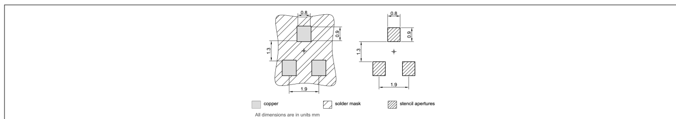
Figure 11 Foot print
