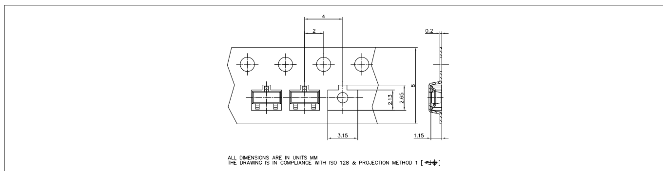
Figure 13 Tape dimensions
