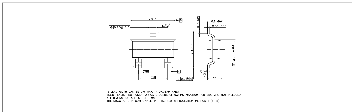
Figure 10 Package outline
