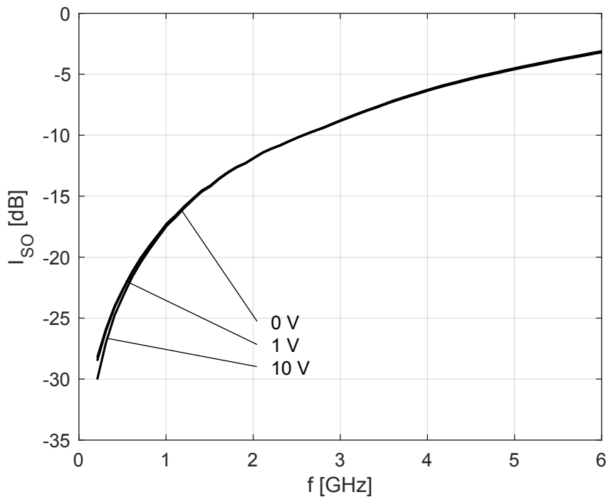
Figure 6 Isolation I_{50} vs. frequency f at different reverse voltages
