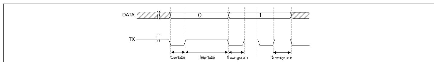
Figure 18 10BASE-T1S Signal Timing
