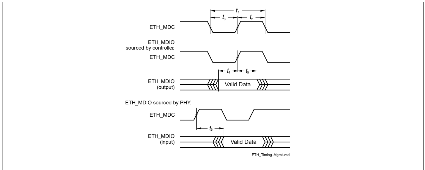
Figure 17 ETH management signal timing
