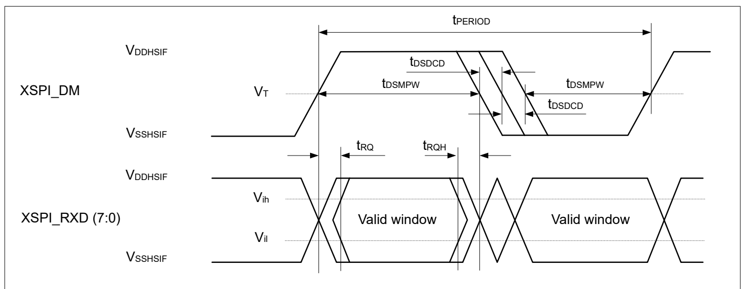
Figure 31 Data Strobe to Data Input Timing
