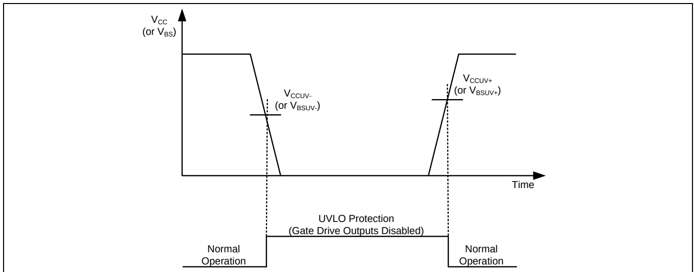
Figure 16 UVLO protection
