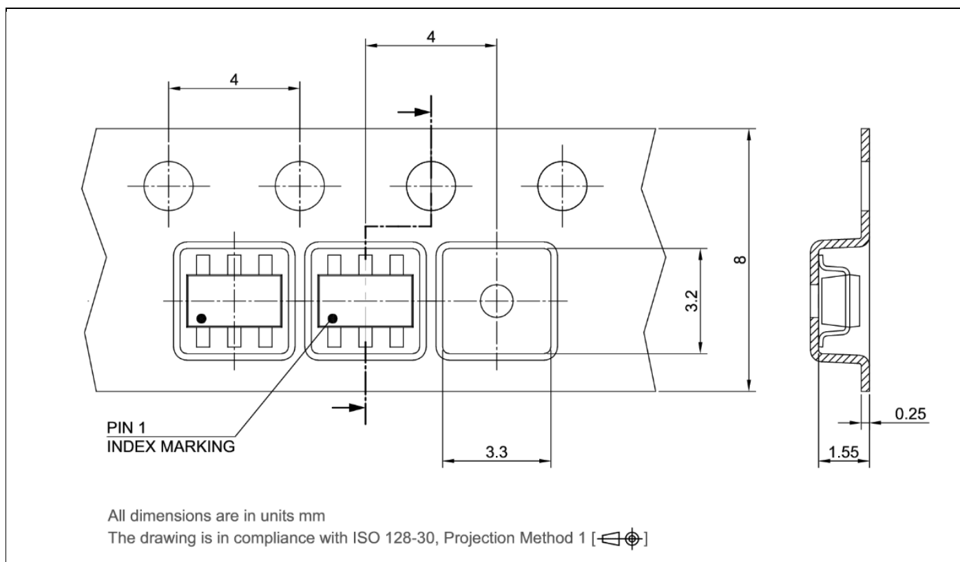
Figure 15 Tape and reel dimensions
