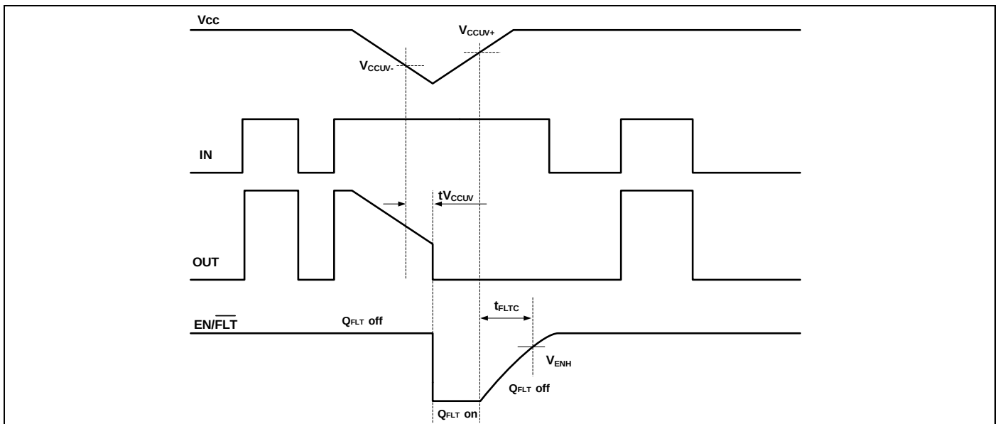
Figure 8 V_{CC} under voltage protection waveform definitions
