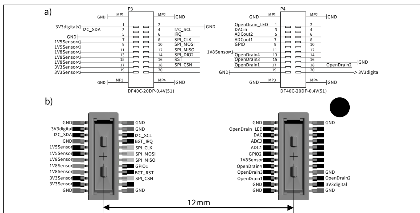
Figure 9 Pinout (a) and pad layout (b) of the sensor connectors on the BGT60TR13C shield
