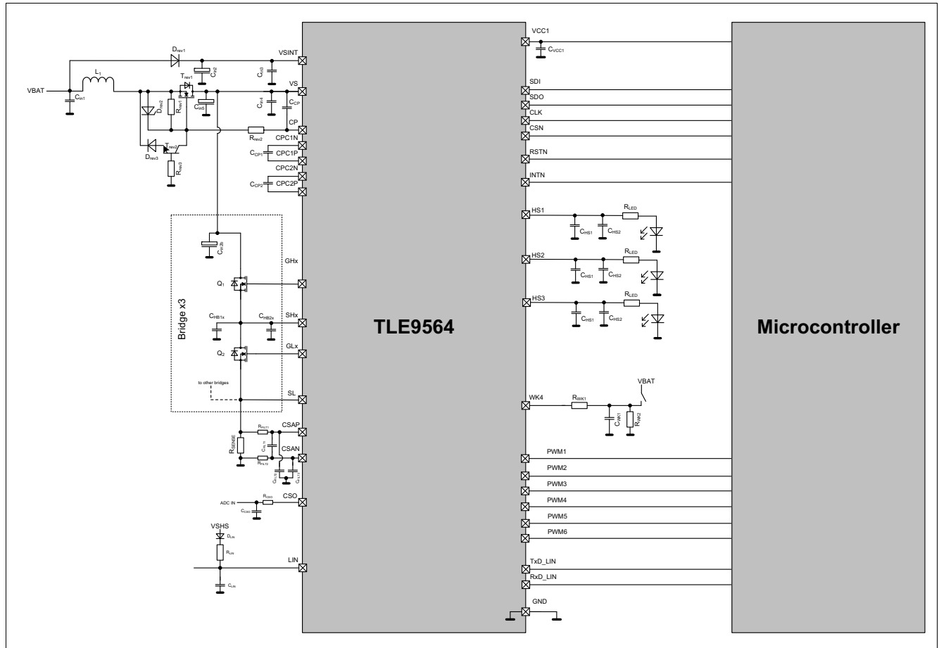
Figure 75 TLE9564QXW Application Diagram
