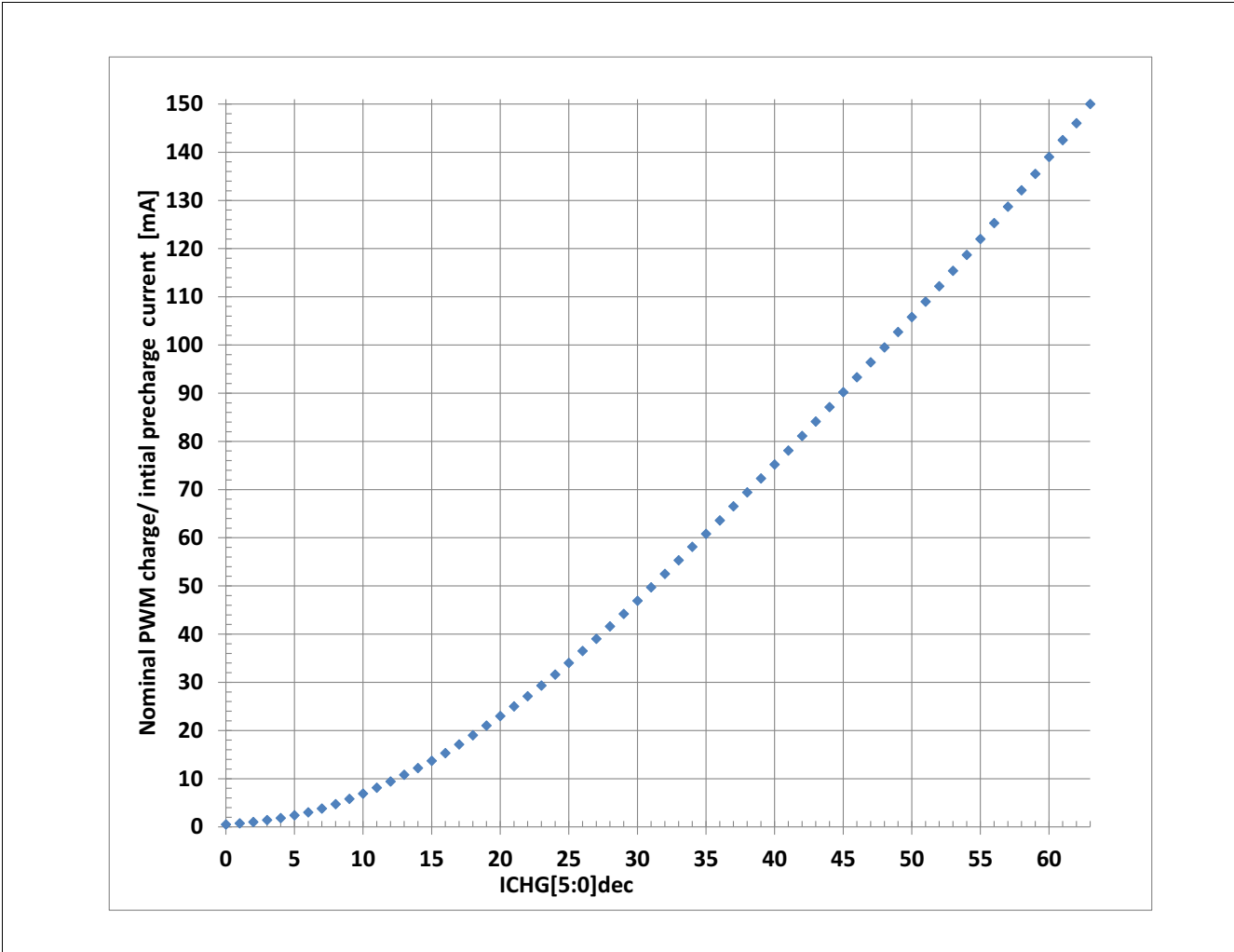
Figure 55 Configurable charge currents in PWM operation
