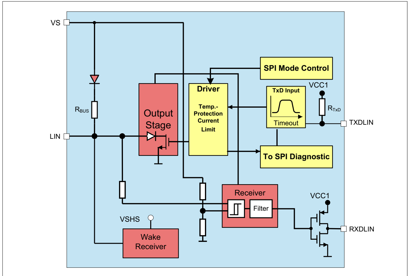
Figure 24 Block Diagram
