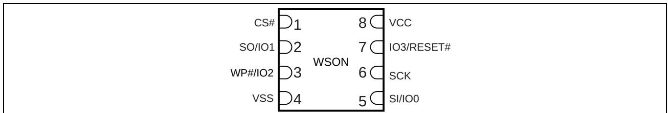
Figure 39 8-connector package (WSO6), top view [33]
