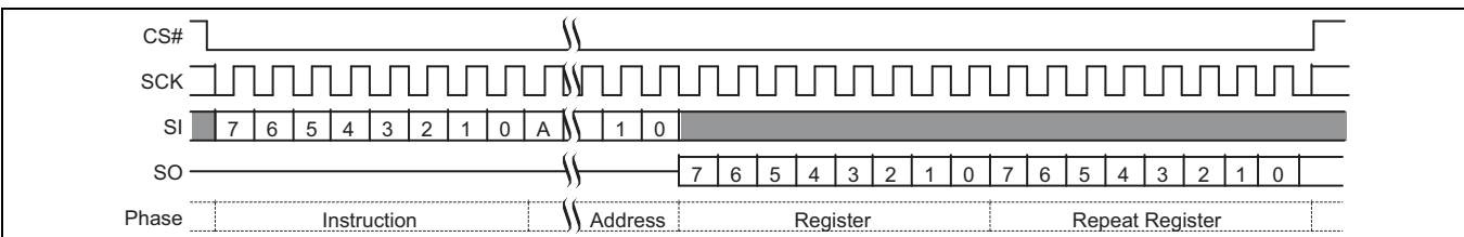
Figure 104 DYBRD command sequence [68, 69]
