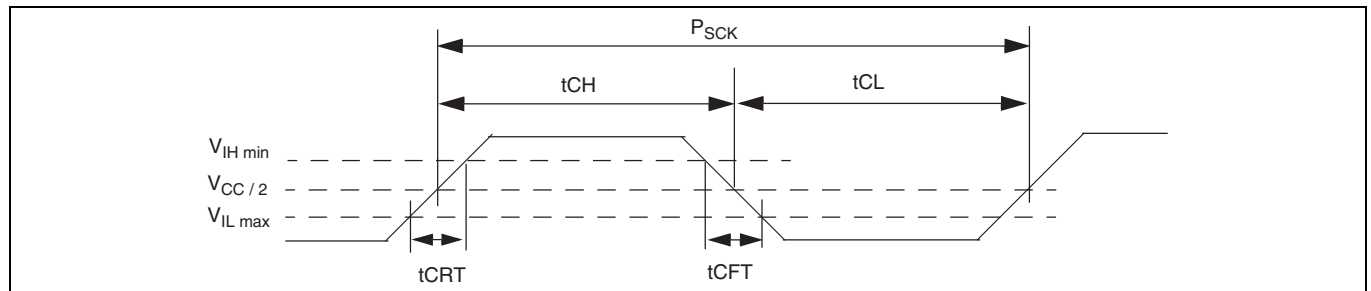
Figure 28 Clock timing
