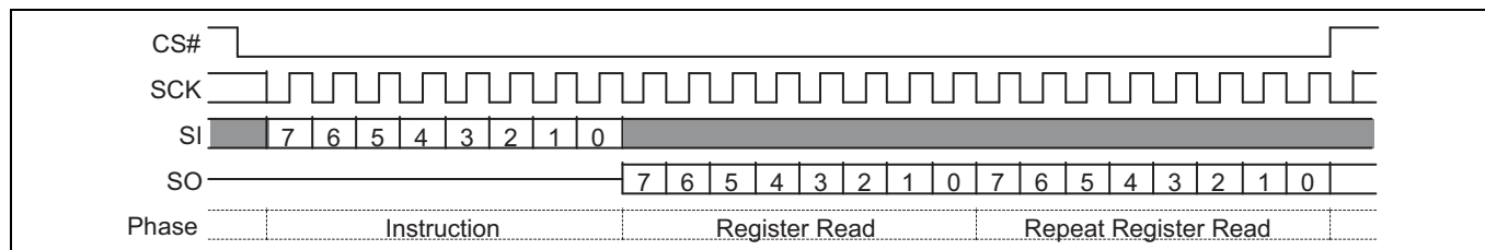
Figure 72 DLPRD (DLPRD) command sequence
