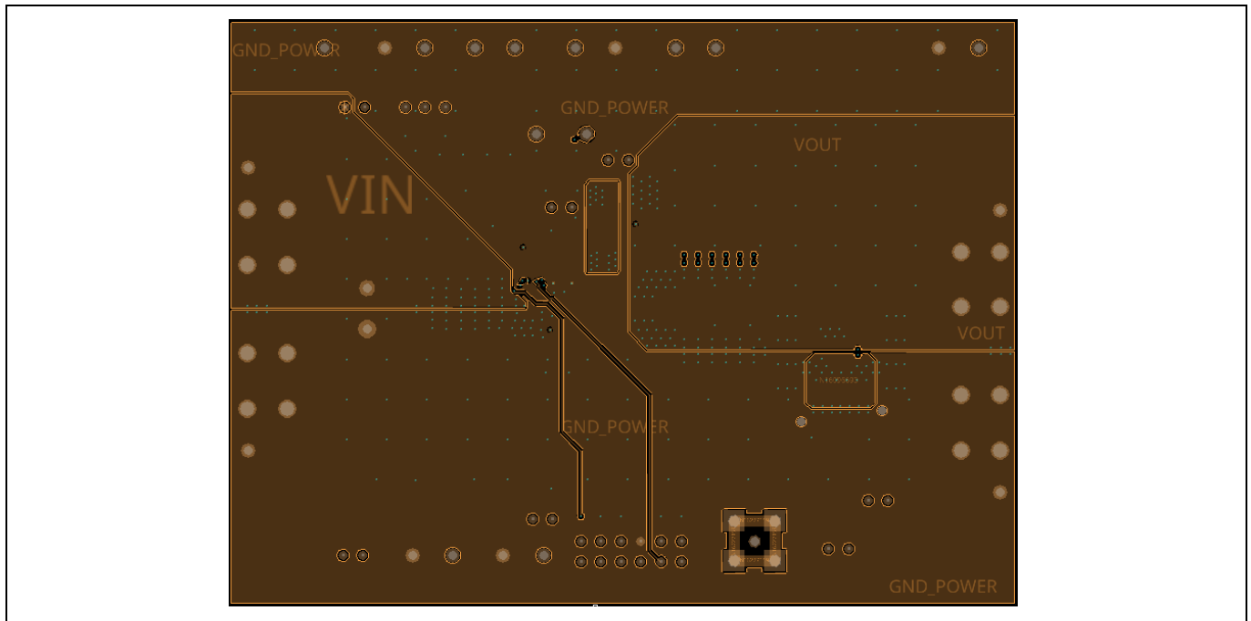
Figure 6 Inner layer 3
