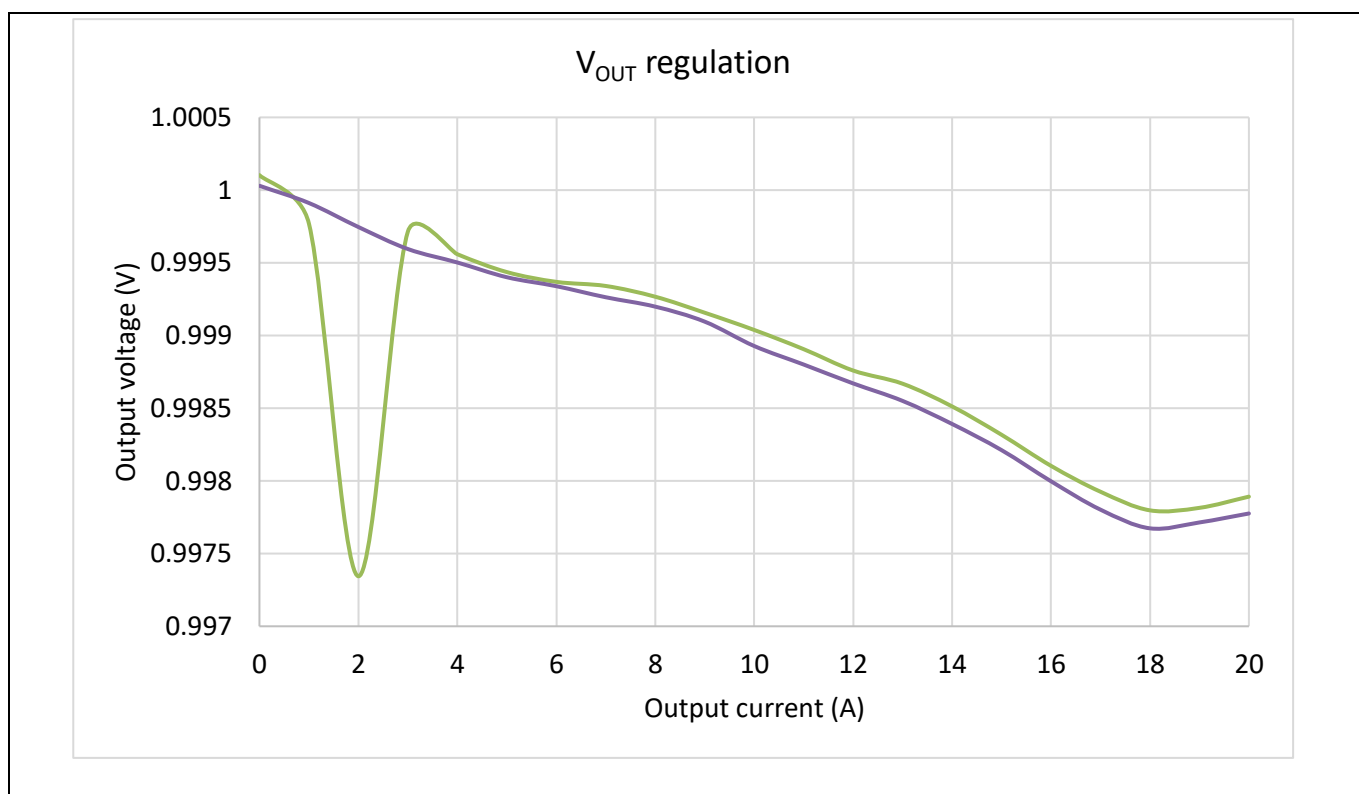
Figure 10 Output voltage regulation
