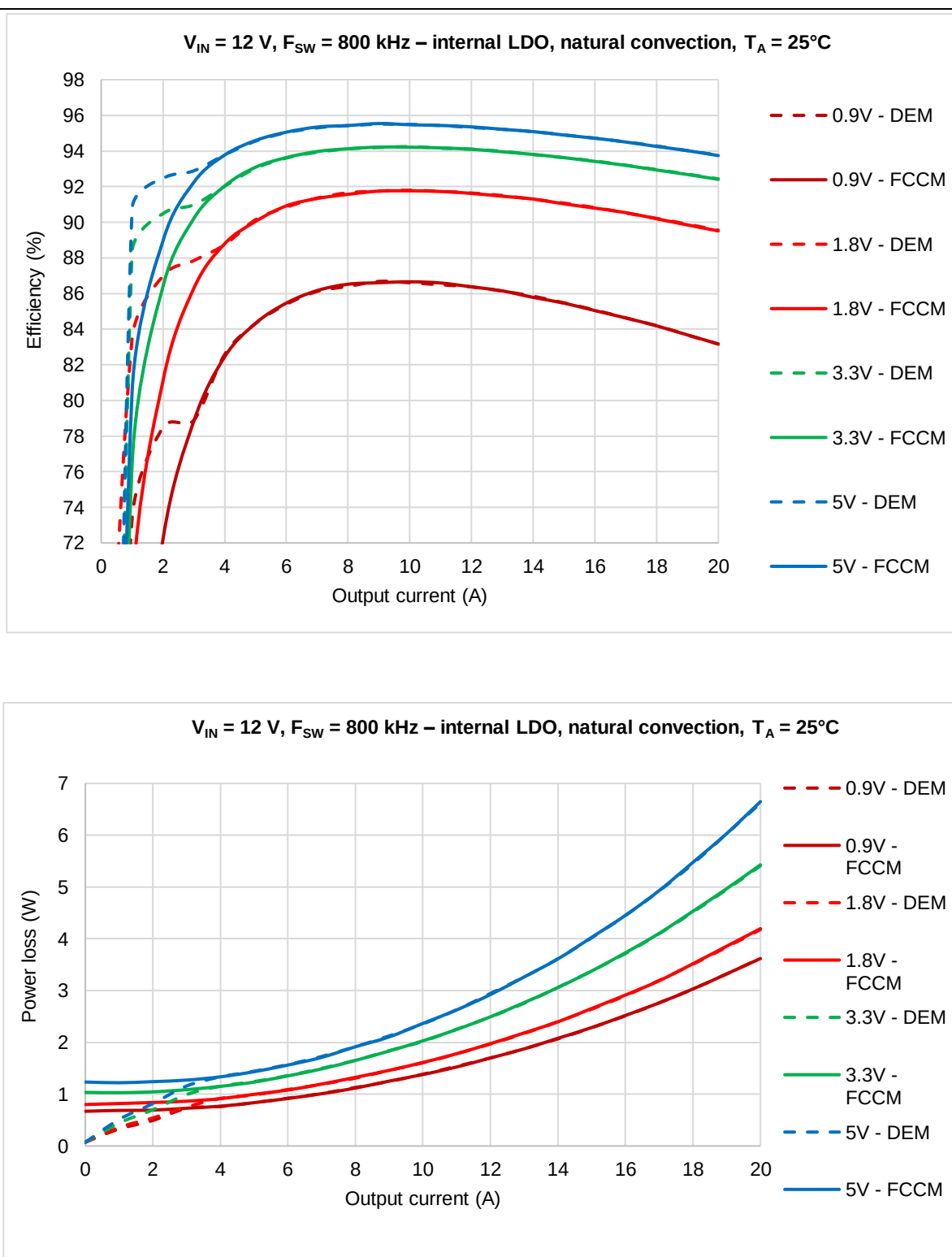
Figure 9 Efficiency and power loss
