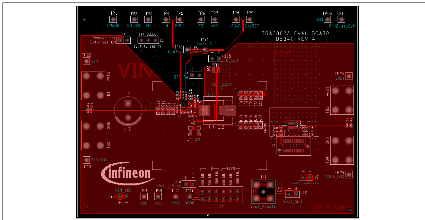
Figure 2 Top layer
