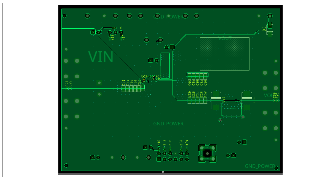
Figure 3 Bottom layer
