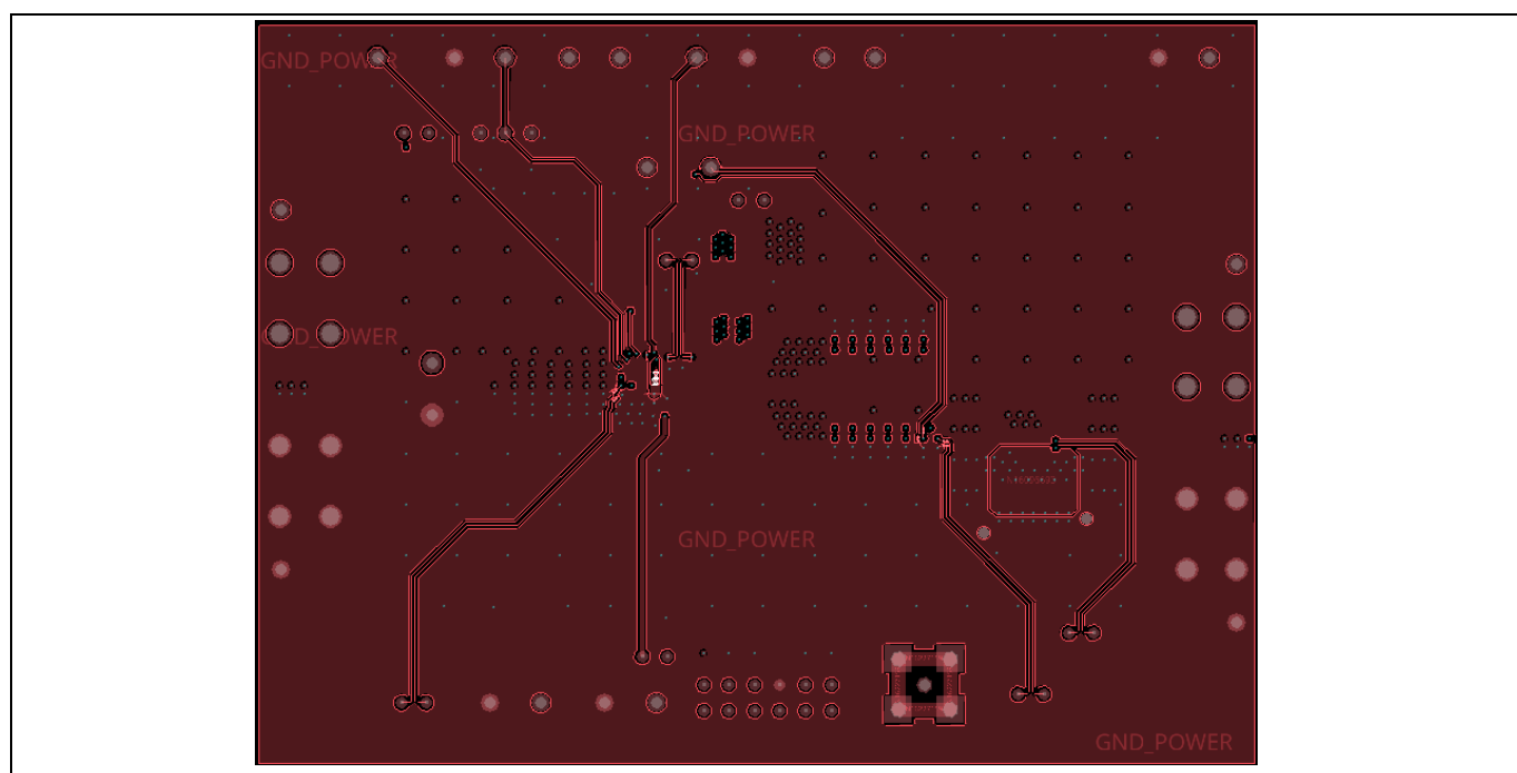
Figure 5 Inner layer 2
