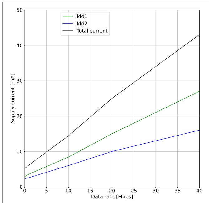
Figure 19 Supply current vs. data rate ( V_{\text{DD1}} = V_{\text{DD2}} = 6.5\text{ V} )
