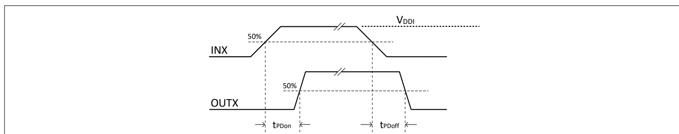
Figure 12 Propagation delays
