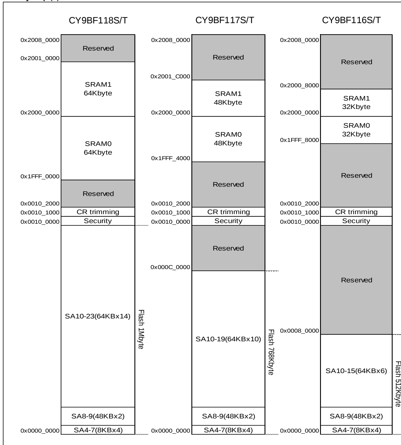
Memory Map (2)
