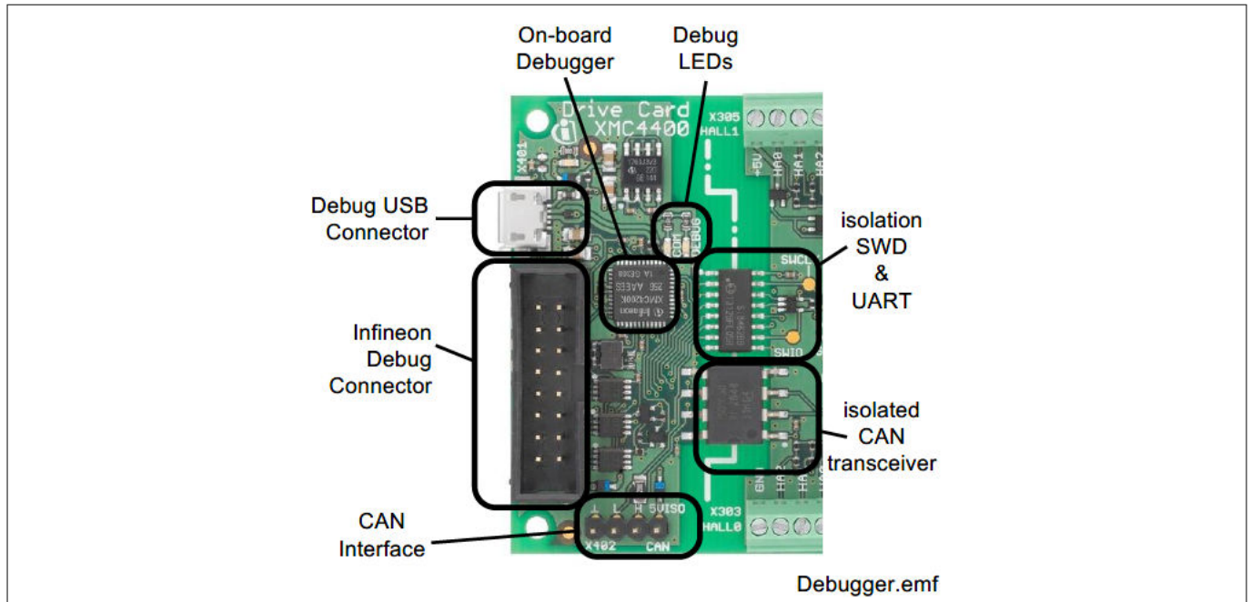
Figure 8 On-Board USB Debugger
