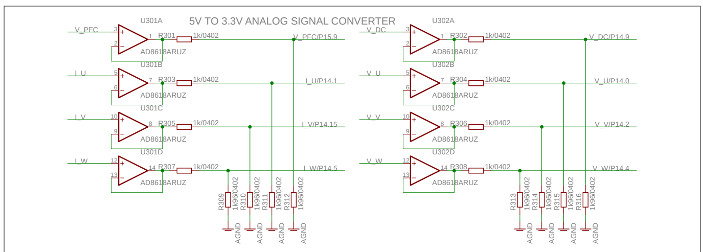
Figure 16 Buffered Level Shifter for High Impedance Analog Signals
