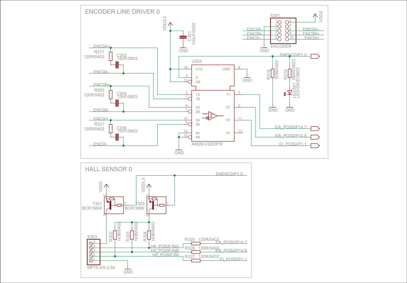
Figure 14 Hall Sensor and Encoder Interface Circuitry
