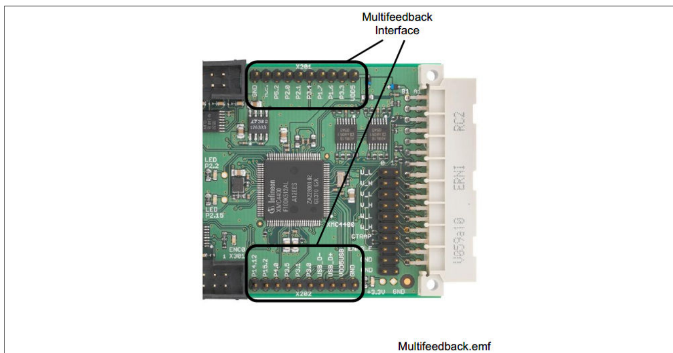
Figure 12 Multifeedback Interface Connectors
