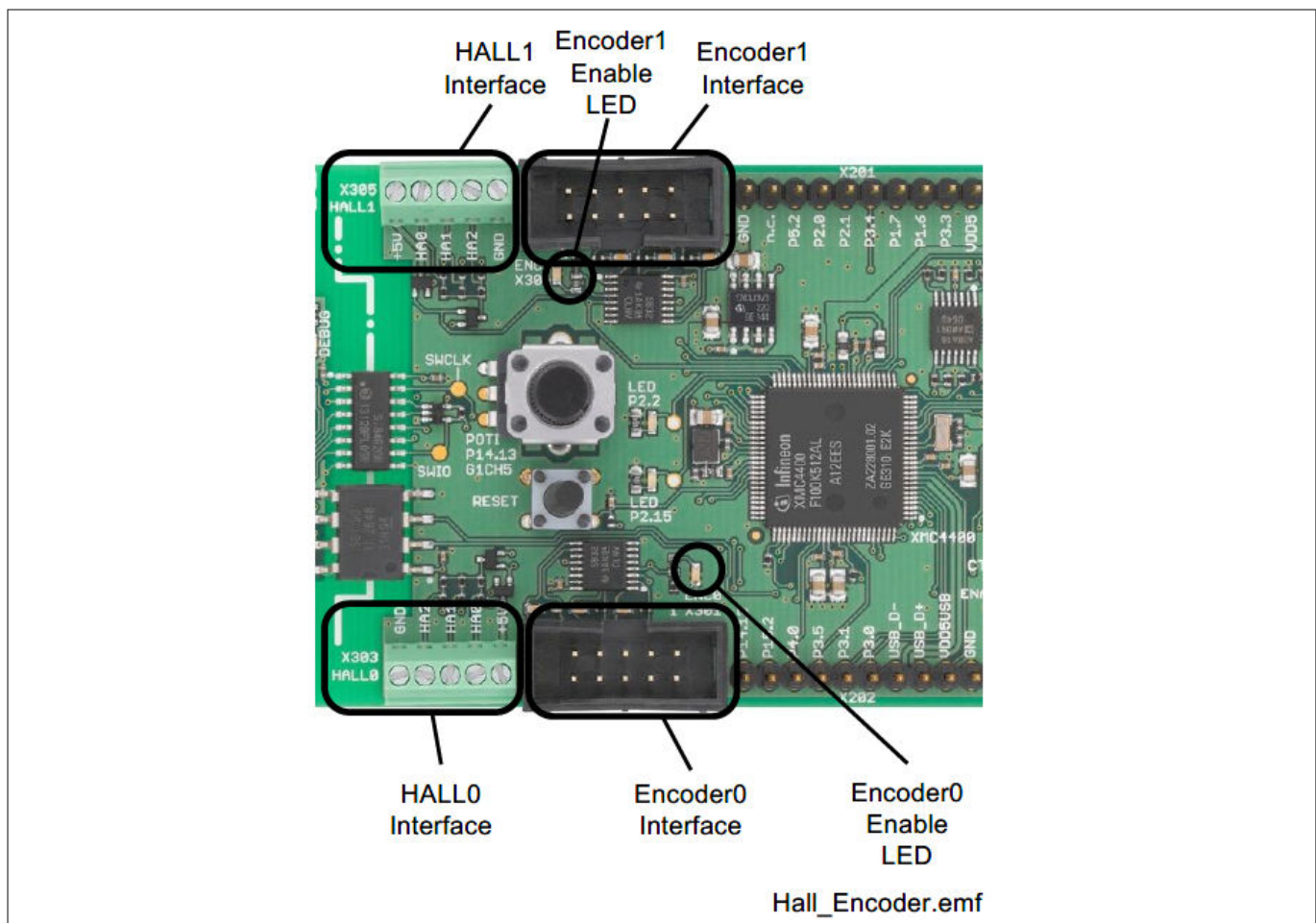
Figure 13 Hall Sensor and Encoder Connectors
