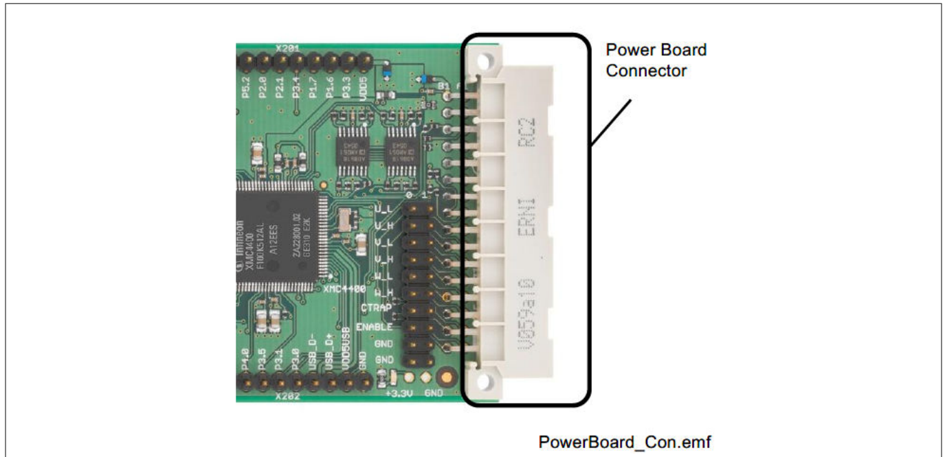
Figure 15 Power Board Connector
