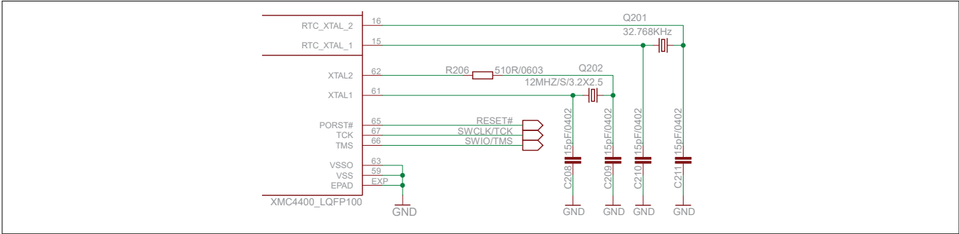
Figure 6 Clock Generation
