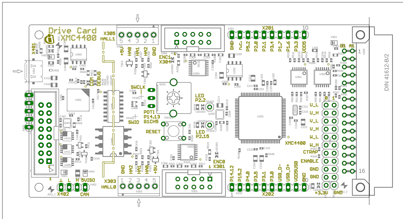
Figure 20 Component Placement
