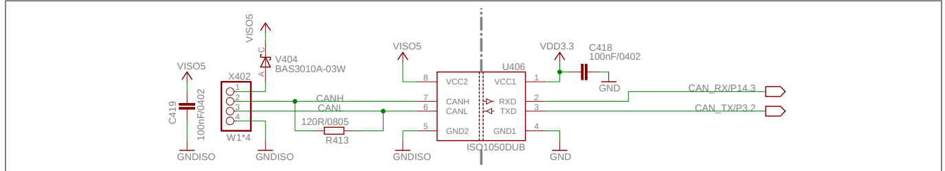
Figure 10 Isolated CAN Interface with Termination
