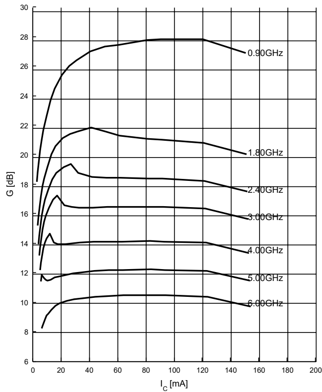
Figure 6 Maximum power gain G_{max} = f(I_C) , V_{CE} = 3\text{ V} , f = \text{parameter in GHz}
