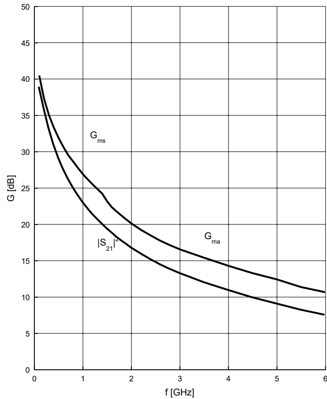
Figure 5 Gain G_{ma} , G_{ms} , |S_{21}|^2 = f(f) , V_{CE} = 3\text{ V} , I_C = 80\text{ mA}
