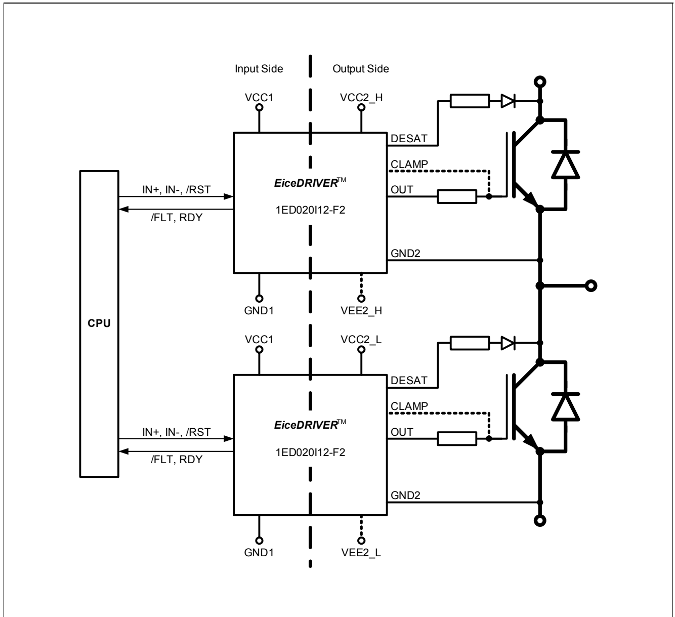
Figure 1 Typical Application
