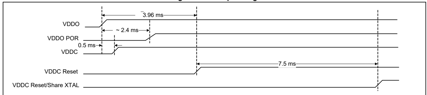
Figure 9. Startup Timing
