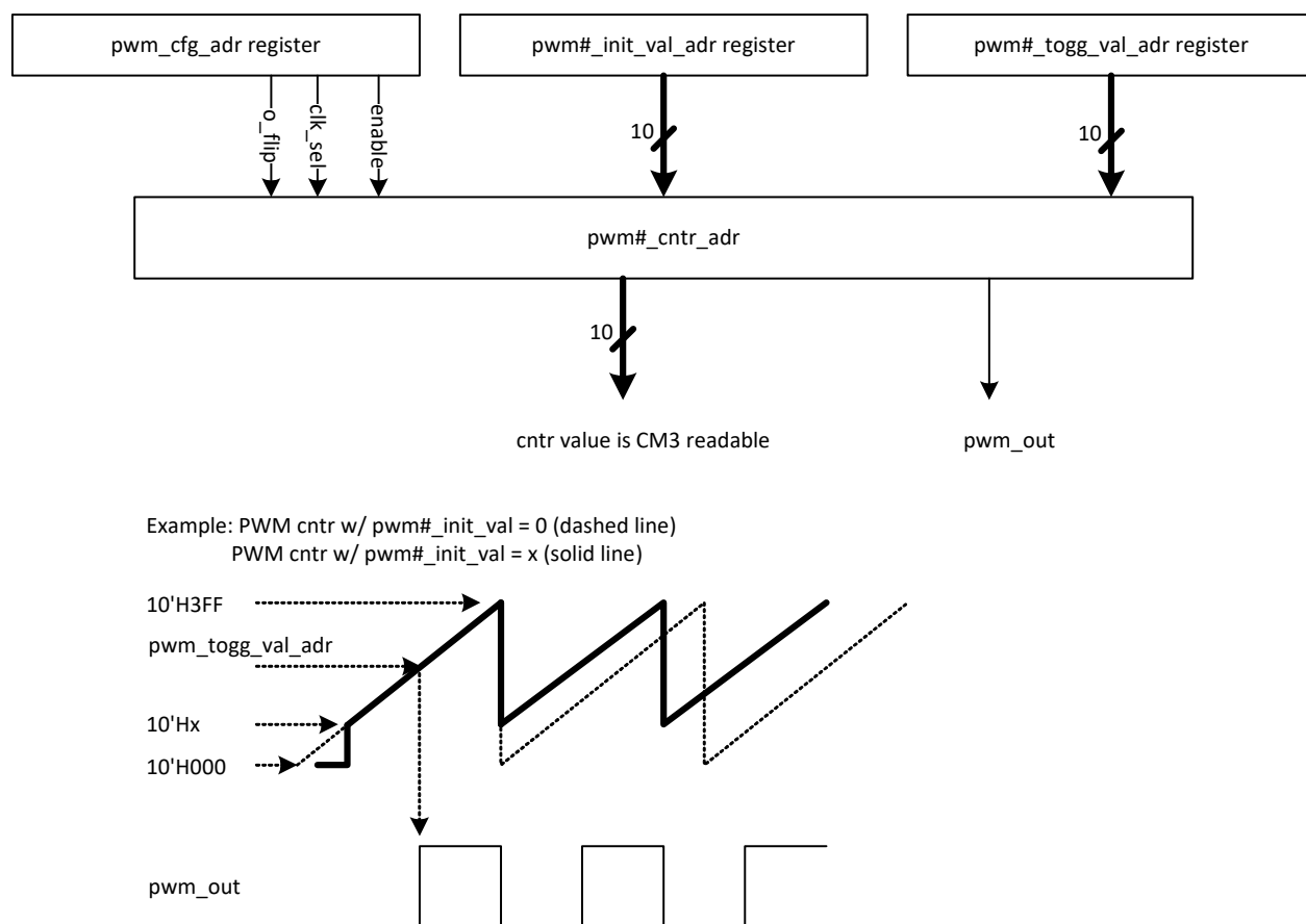
Figure 7. PWM Channel Block Diagram
