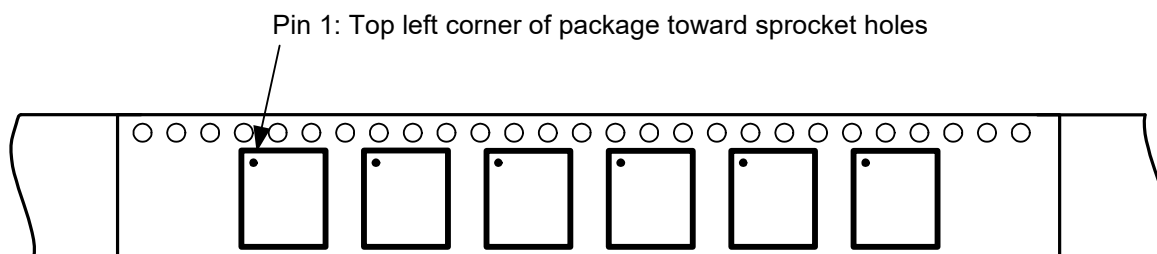
Figure 17. Pin 1 Orientation
