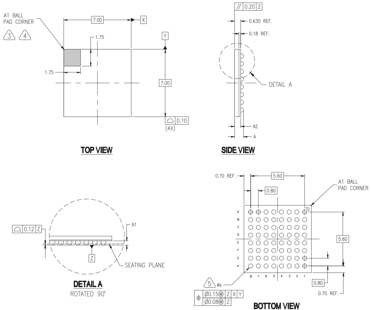
Figure 16. 64-pin FBGA Package
