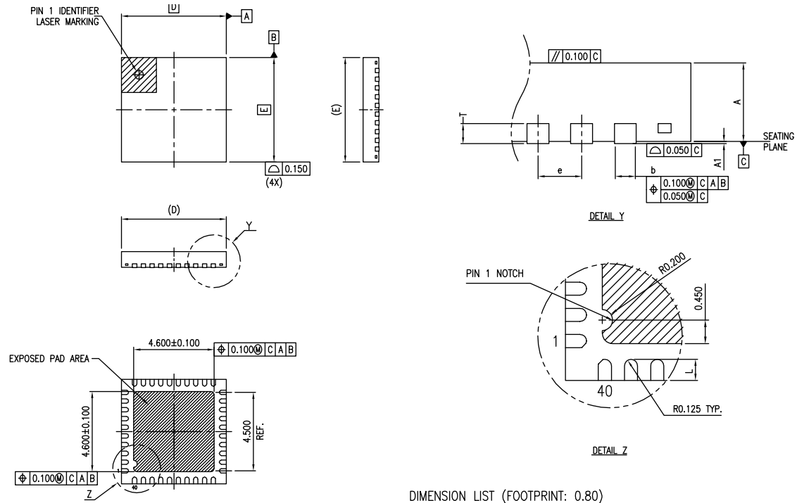
Figure 15. 40-pin QFN Package
