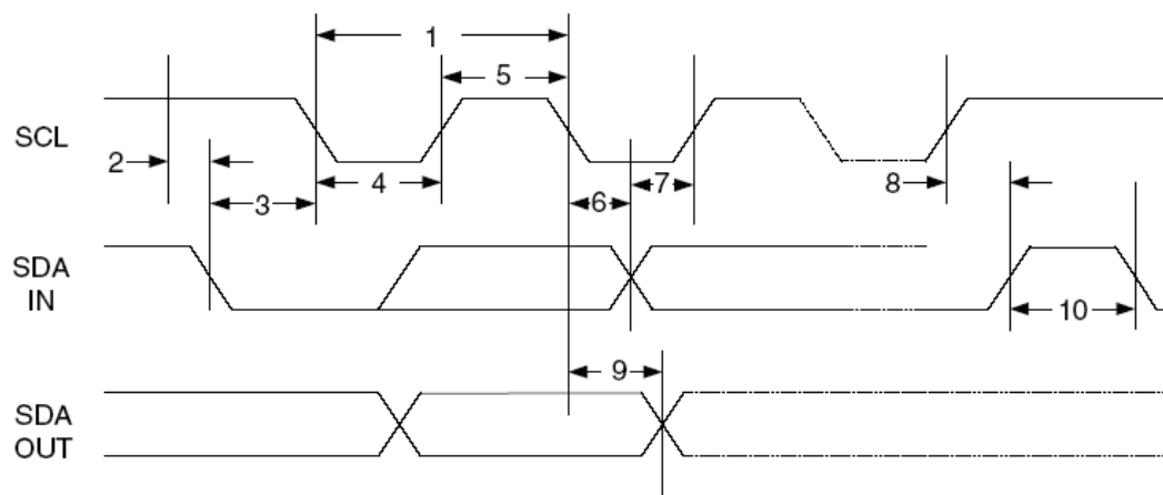
Figure 13. Interface Timing Diagram
