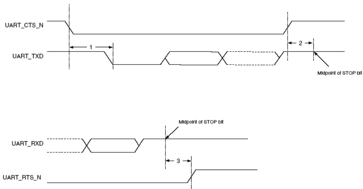
Figure 11. UART Timing
