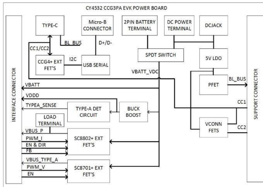
Figure 3-2. CY4532 Power Board Block Diagram
