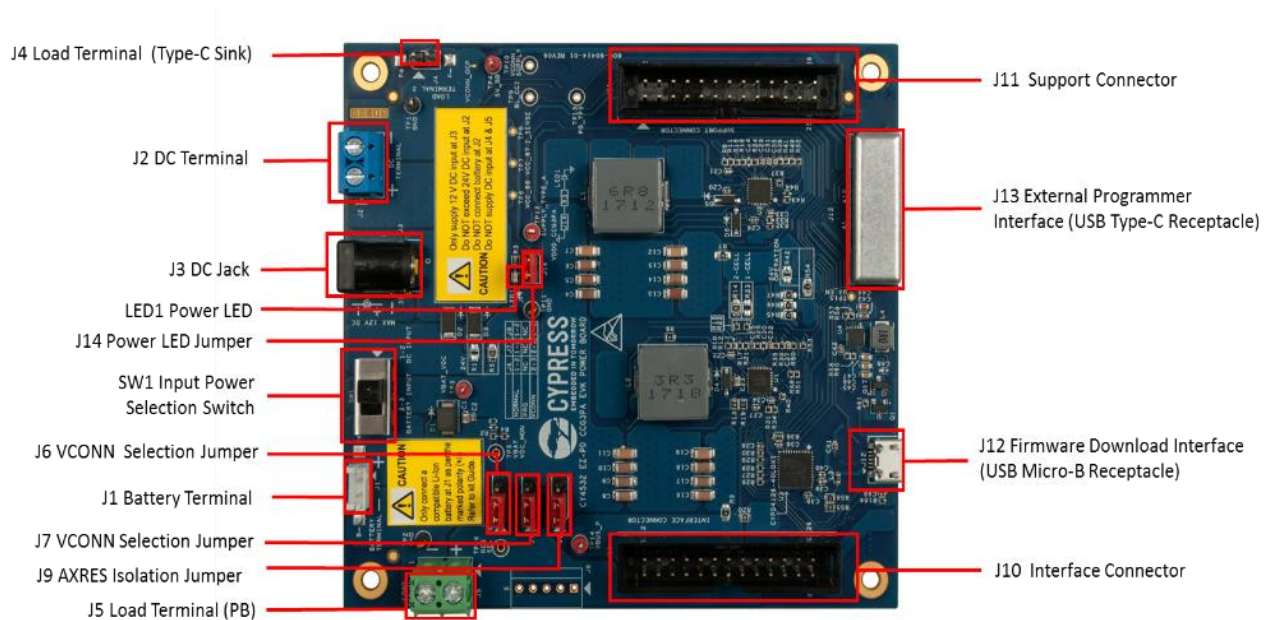
Figure 3-3. CY4532 Power Board Connectors
