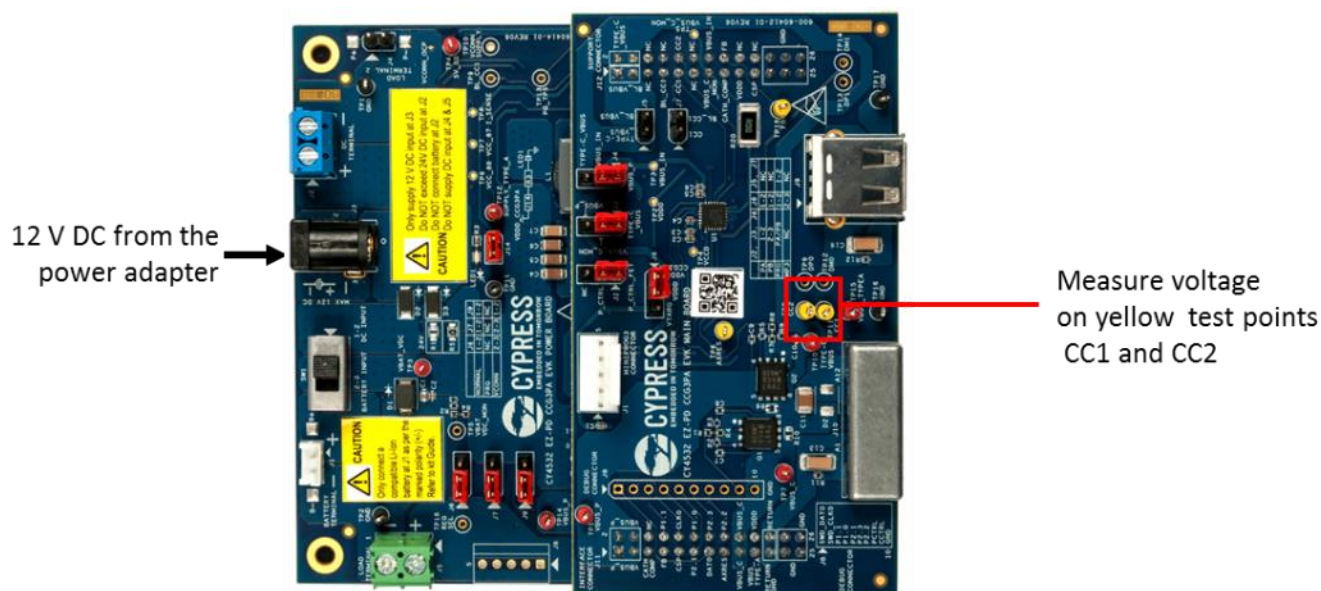
Figure C-1. Setup to Identify the Application Firmware Type
