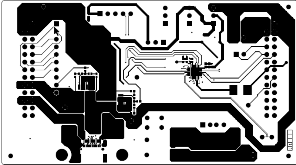
600-60412-01 REV06 PRIMARY SIDE
