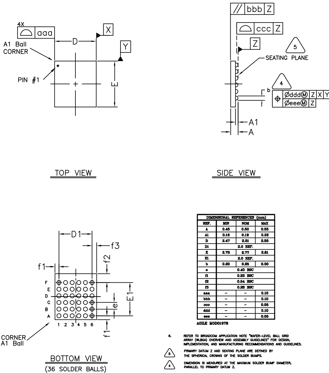
Figure 21. CYW20707 36-pin WLPGA Package (2.8 mm x 2.5 mm)
