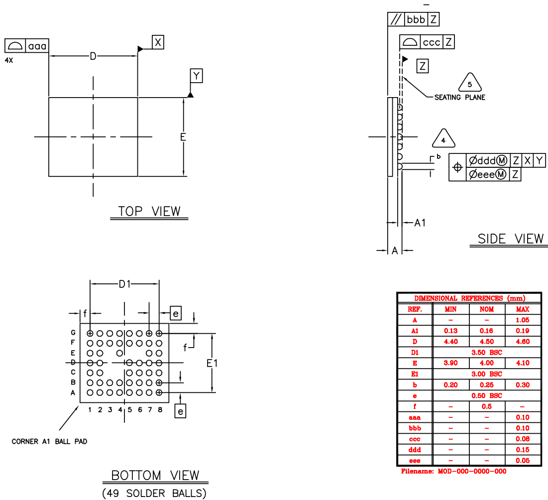
Figure 20. CYW20707 49-pin FBGA Package (4.5 mm x 4.0 mm)
