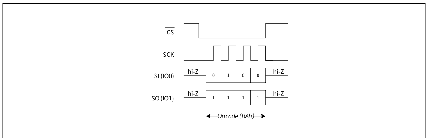
Figure 106 Hibernate mode operation in DPI mode
