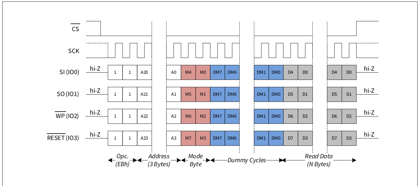
Figure 65 Quad I/O read (QIOR) in QPI mode
