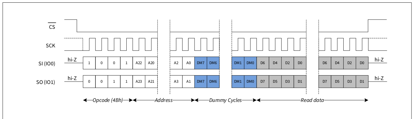
Figure 72 Special sector read (SSRD) in DPI mode
