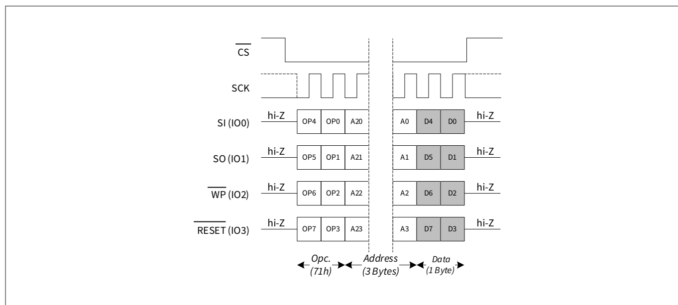
Figure 37 Write any register (WRAR) in QPI mode
