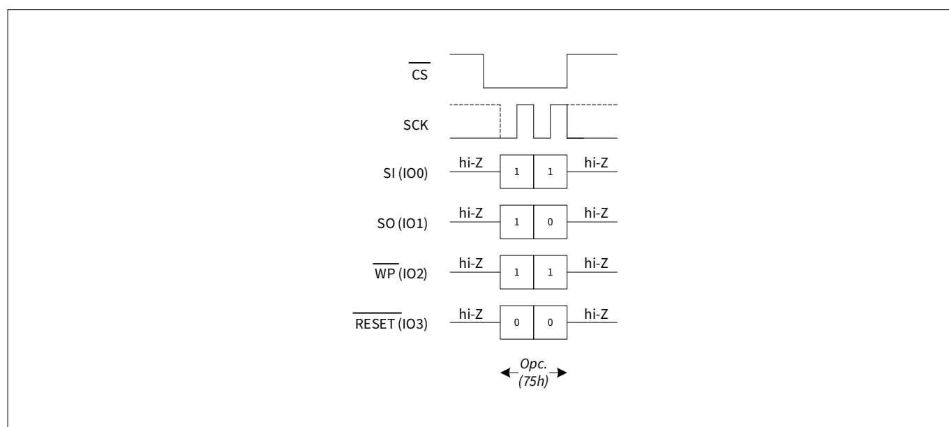
Figure 85 Suspend (EPCS) in QPI mode
