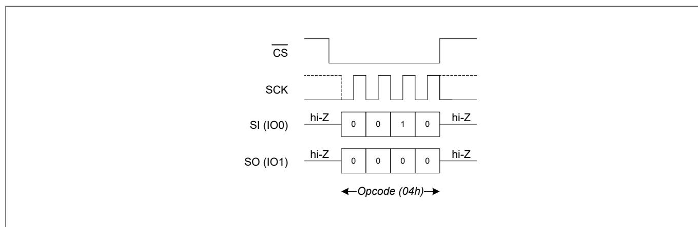
Figure 12 WRDI bus configuration in DPI mode
