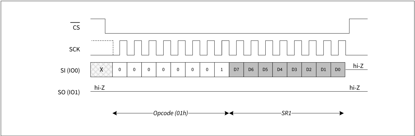
Figure 14 WRSR in SPI mode (WREN not shown)
