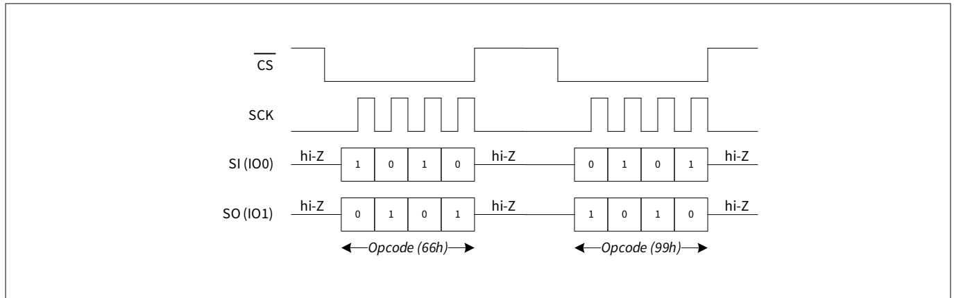
Figure 109 Software reset timing in DPI mode
