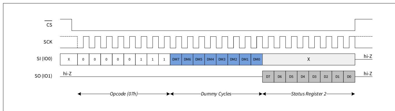
Figure 26 Read CR2 (RDCR2) in SPI mode
