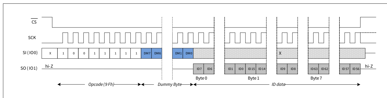
Figure 89 Read device ID (RDID) in SPI mode
