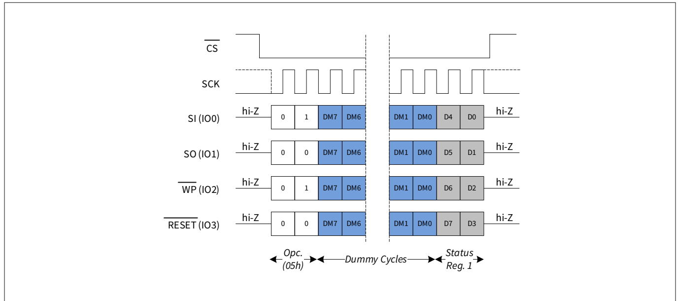
Figure 19 Read SR1 (RDSR1) in QPI mode
