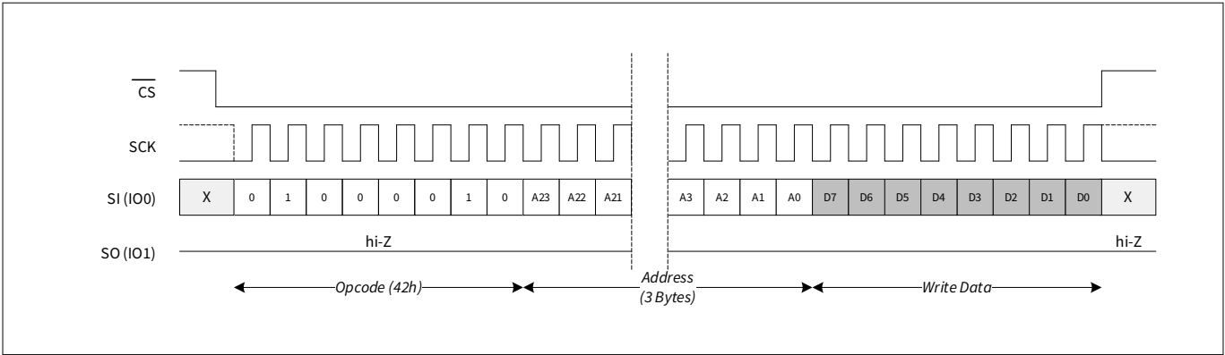
Figure 68 Special sector write (SSWR) in SPI mode (WREN is not shown)
