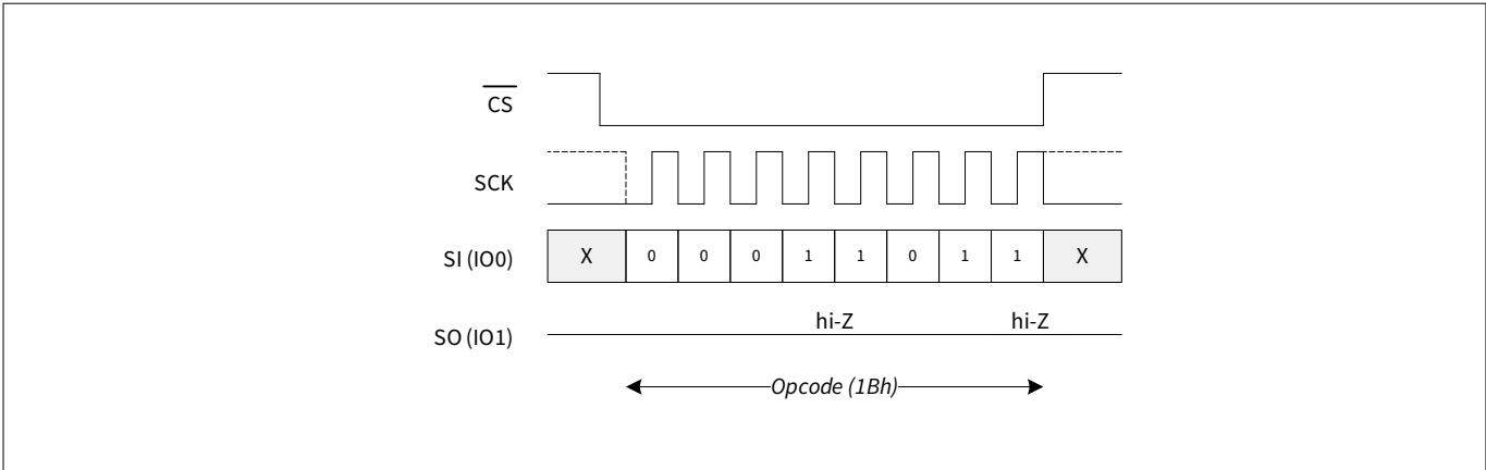
Figure 77 Clear ECC (CLECC) in SPI mode
