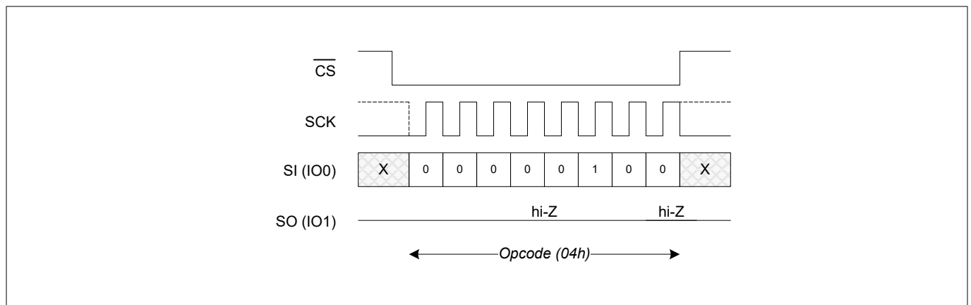
Figure 11 WRDI bus configuration in SPI mode
