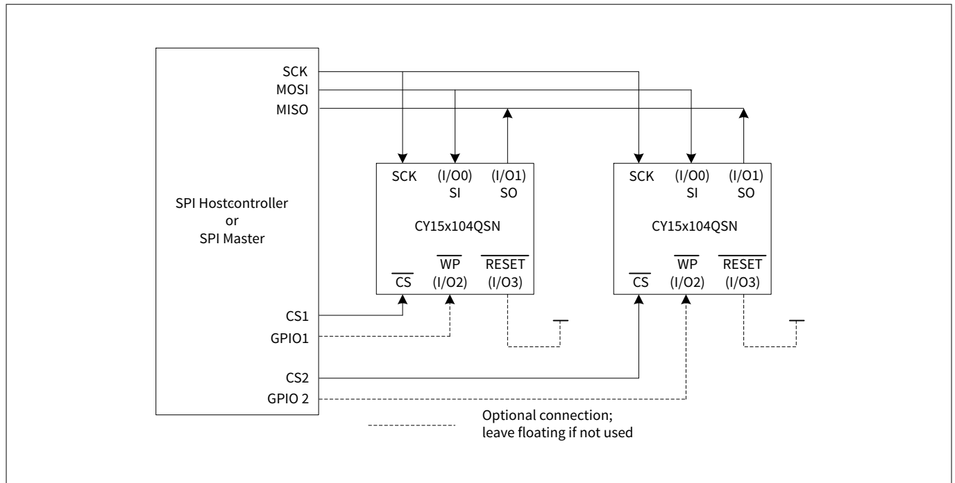
Figure 4 System configuration with SPI port
