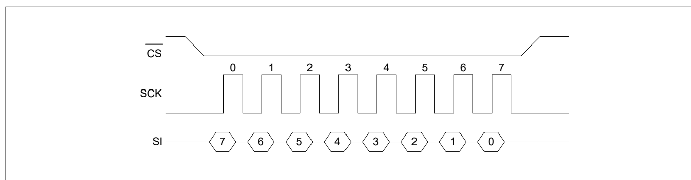
Figure 6 SPI mode 0
