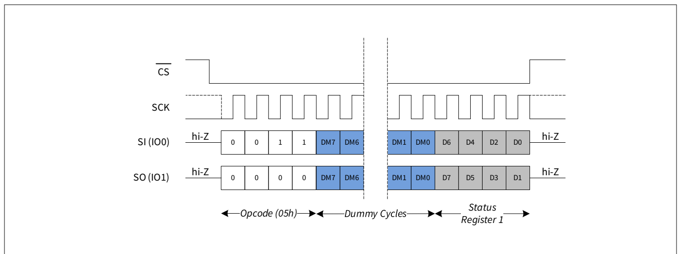
Figure 18 Read SR1 (RDSR1) in DPI mode
