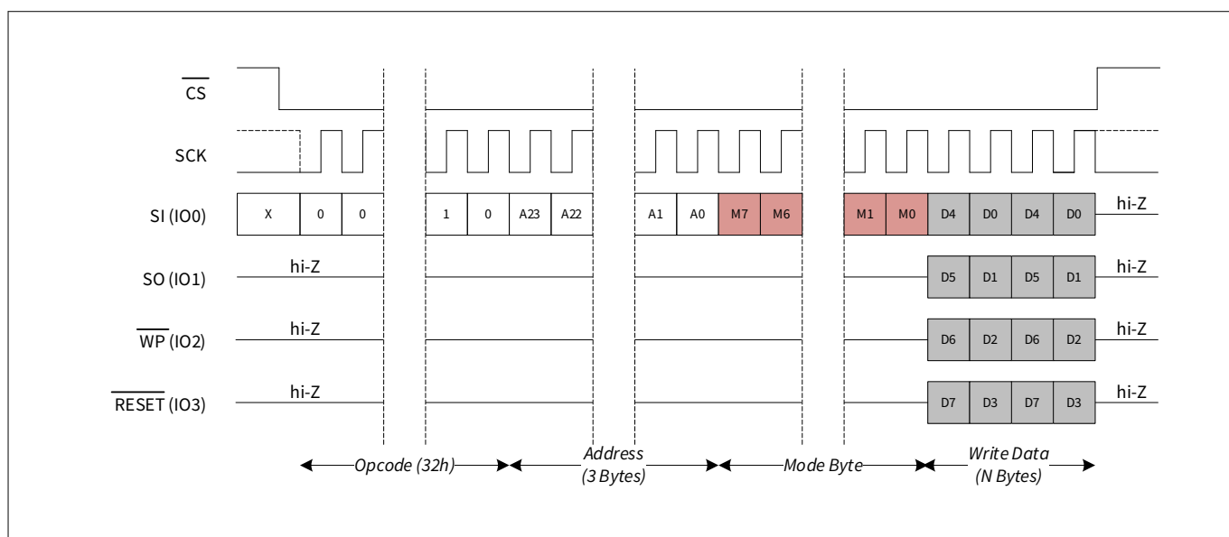
Figure 51 Quad input write (QIW)
