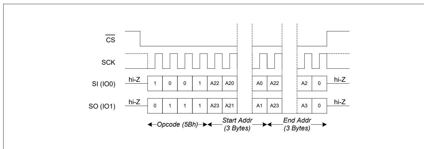
Figure 81 CRC calculation (CRCC) in DPI mode
