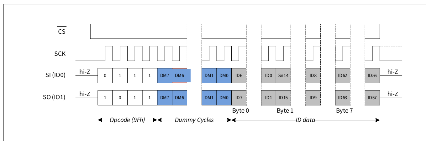
Figure 90 Read device ID (RDID) in DPI mode
