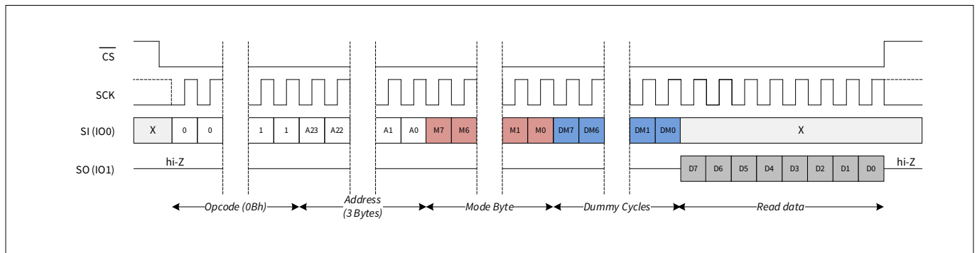
Figure 57 FAST_READ in SPI mode
