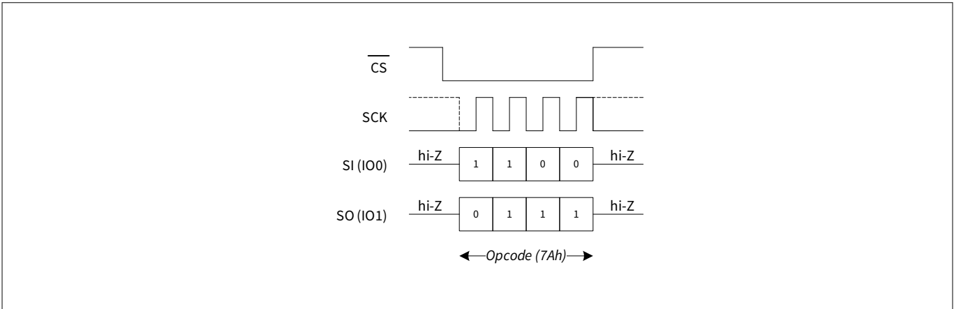
Figure 87 CRC resume (EPCR) in DPI mode
