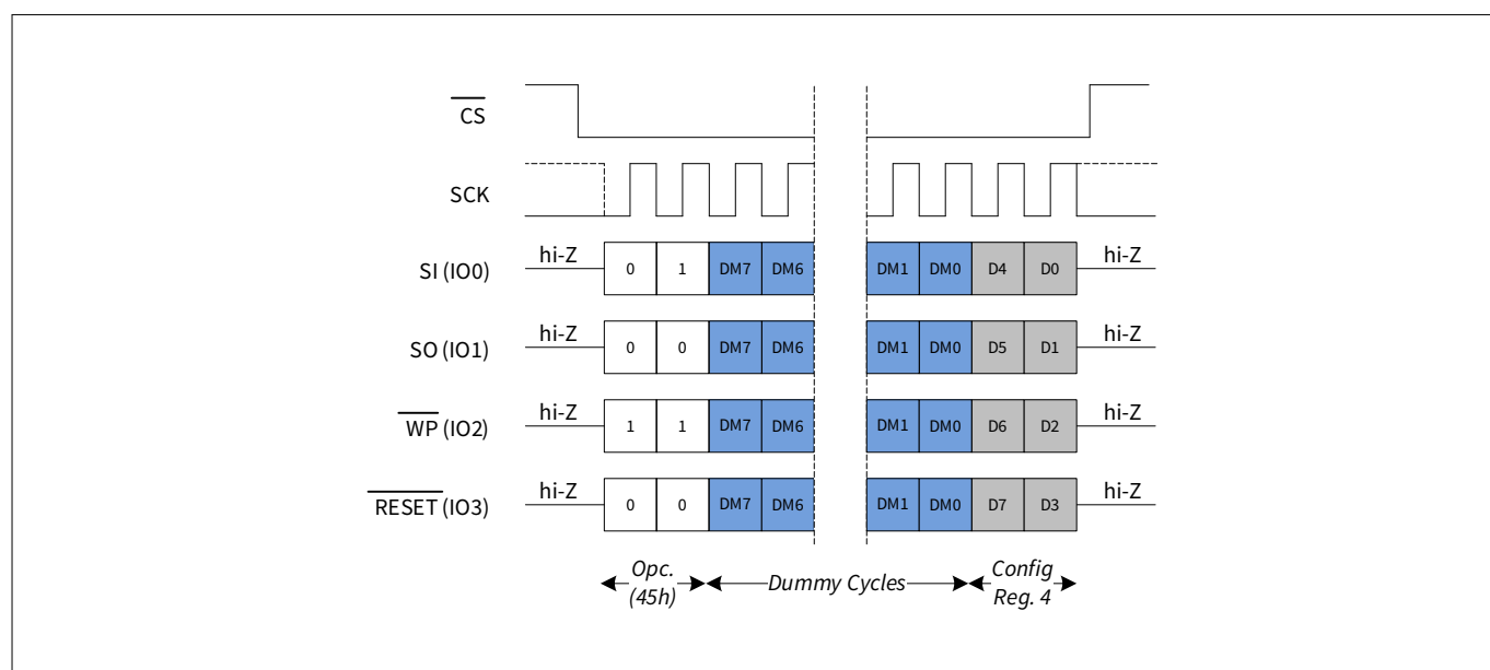
Figure 31 Read CR4 (RDCR4) in QPI mode
