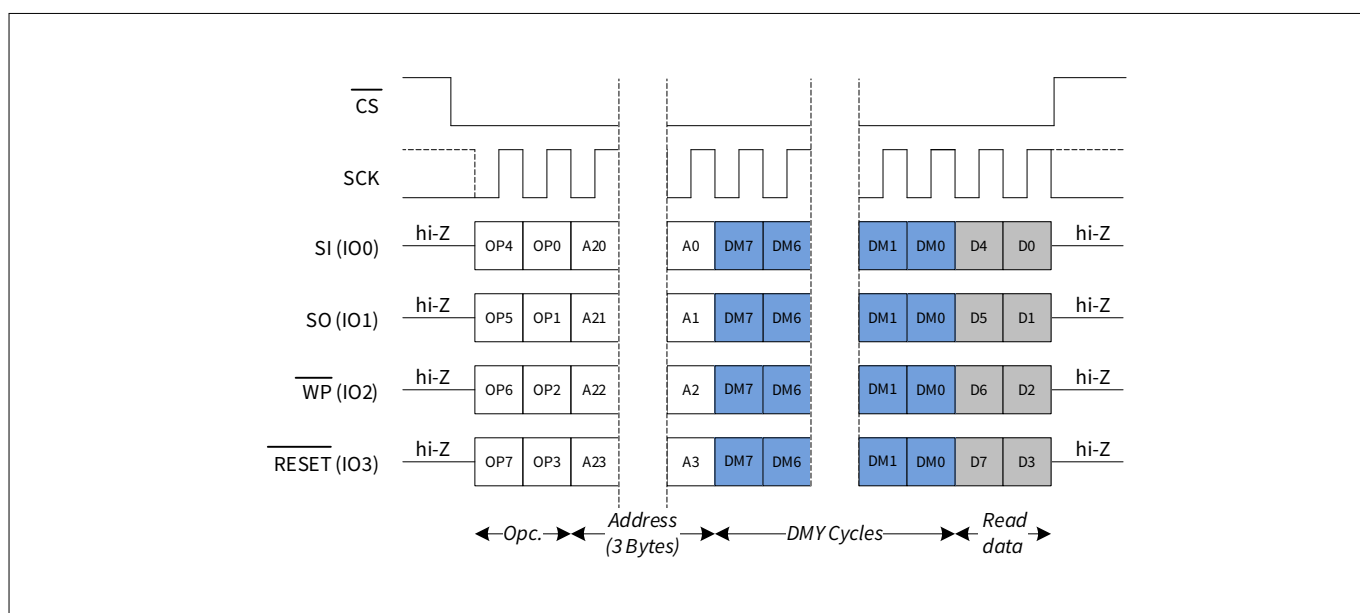
Figure 40 Read any register (RDAR) in QPI mode
