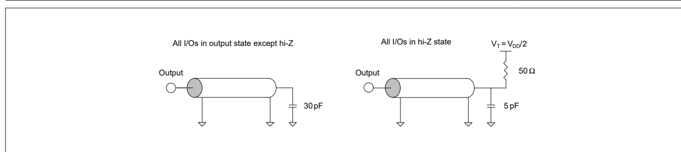
Figure 114 AC test loads
