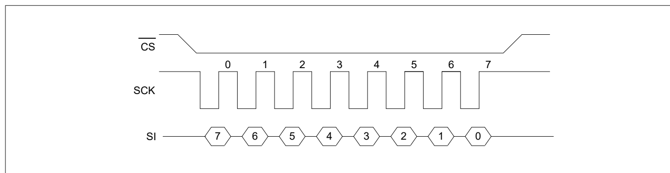
Figure 7 SPI mode 3
