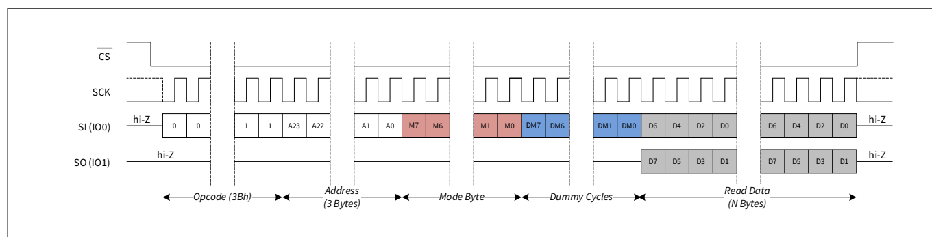
Figure 61 Double output read (DOR)
