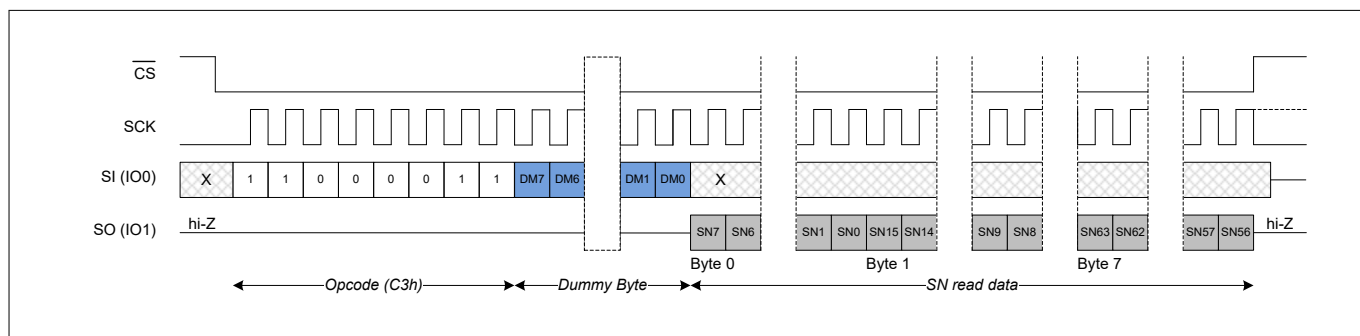
Figure 98 Read serial number (RDSN) in SPI mode
