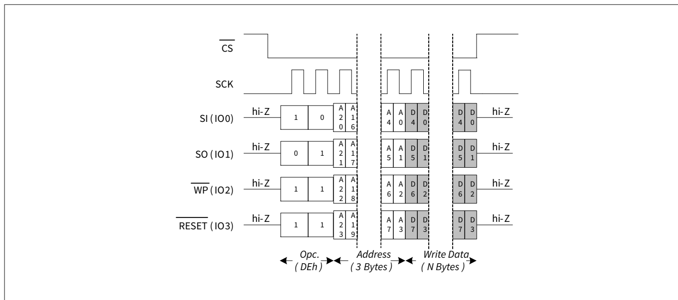
Figure 44 DDR write (DDRWRITE) in QPI mode
