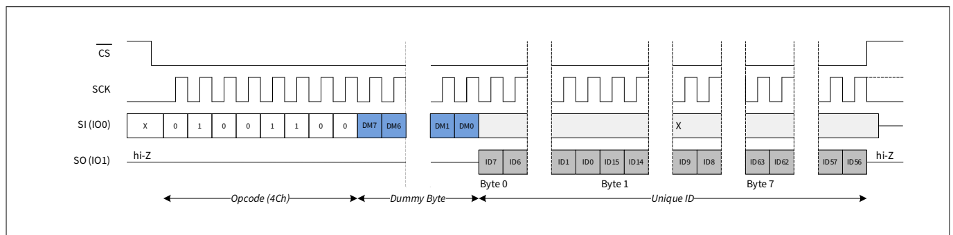
Figure 92 Read unique ID in SPI mode
