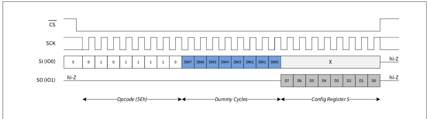
Figure 32 Read CR5 (RDCR5) in SPI mode
