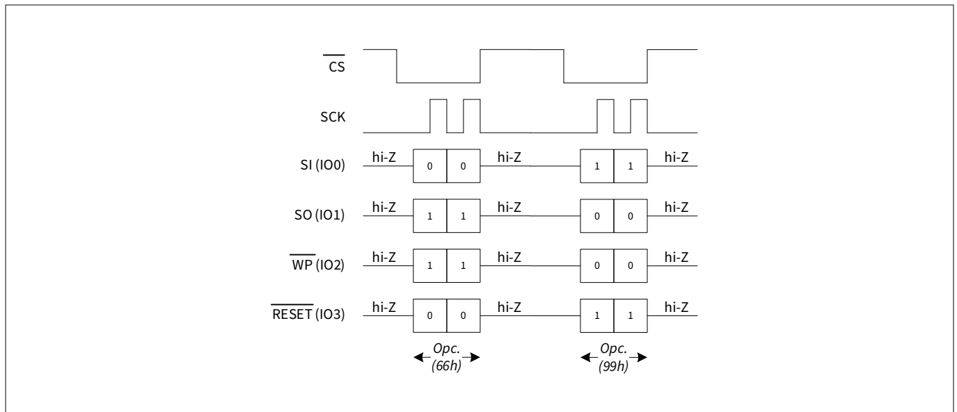
Figure 110 Software reset timing in QPI mode
