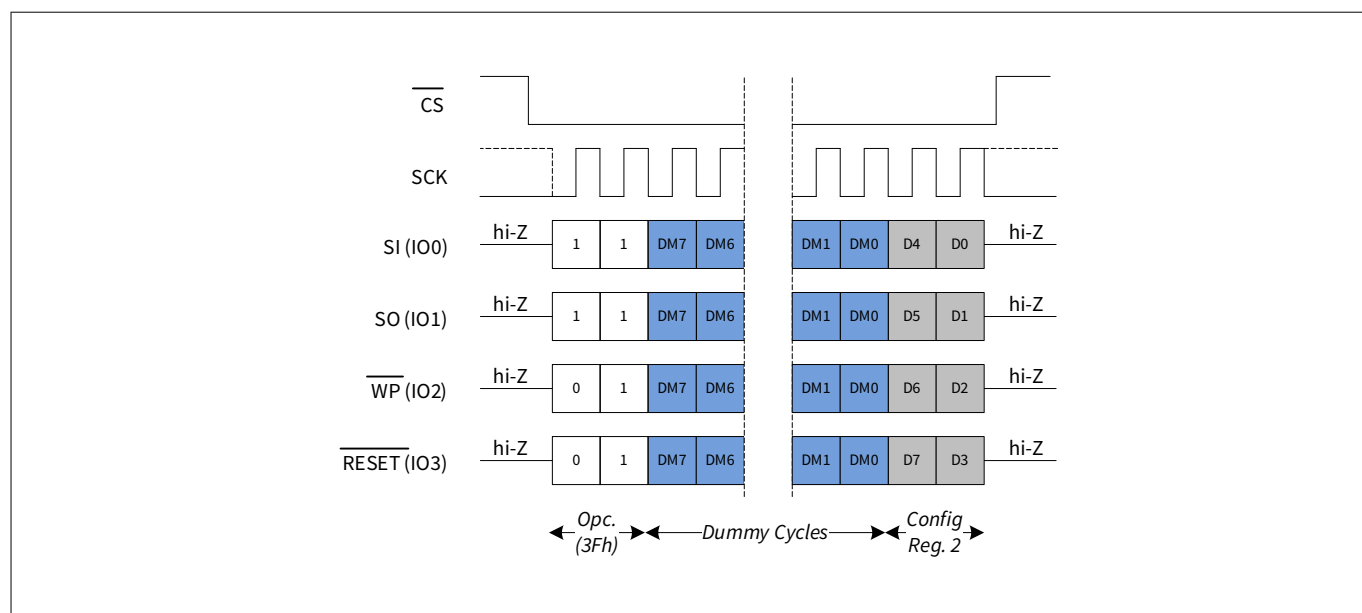
Figure 28 Read CR2 (RDCR2) in QPI mode
