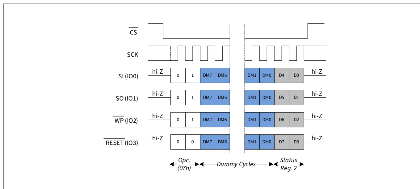
Figure 21 Read SR2 (RDSR2) in DPI mode
