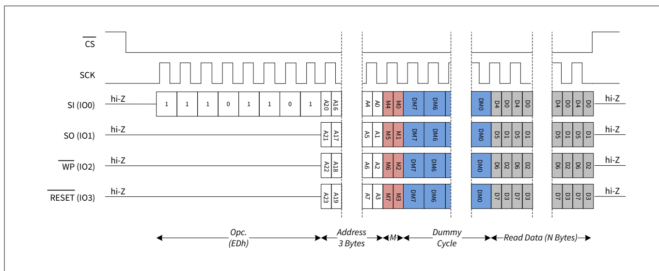
Figure 66 Quad I/O read in DDR (DDRQIOR) – in extended SPI mode
