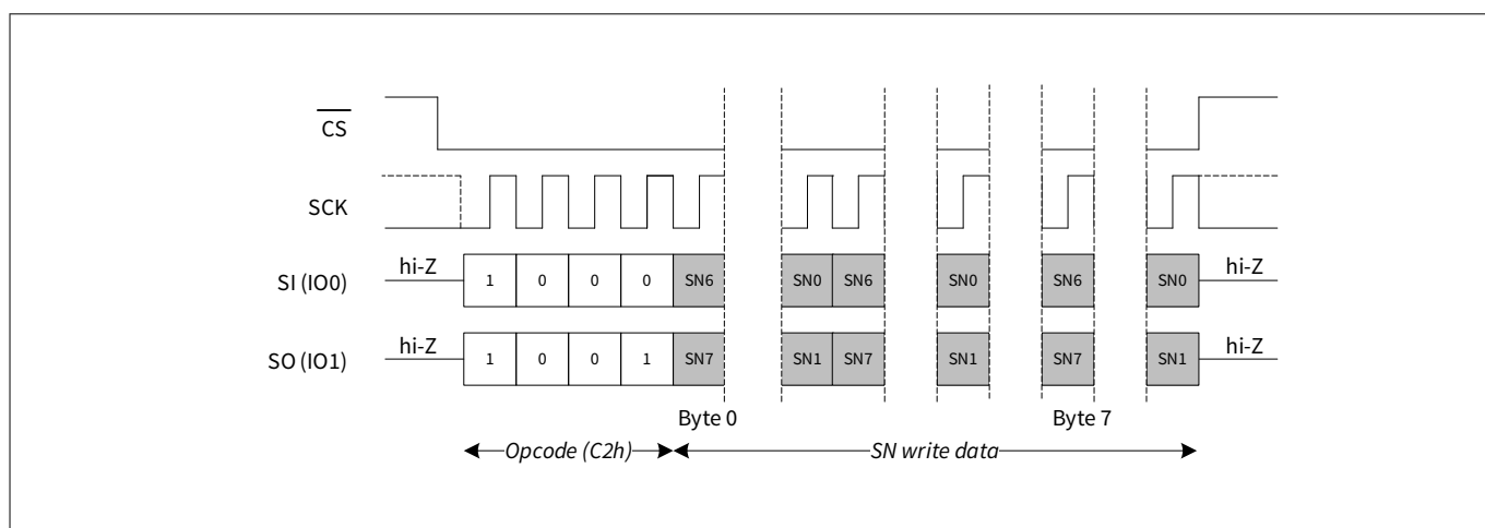
Figure 96 Write serial number in DPI mode (WREN not shown)
