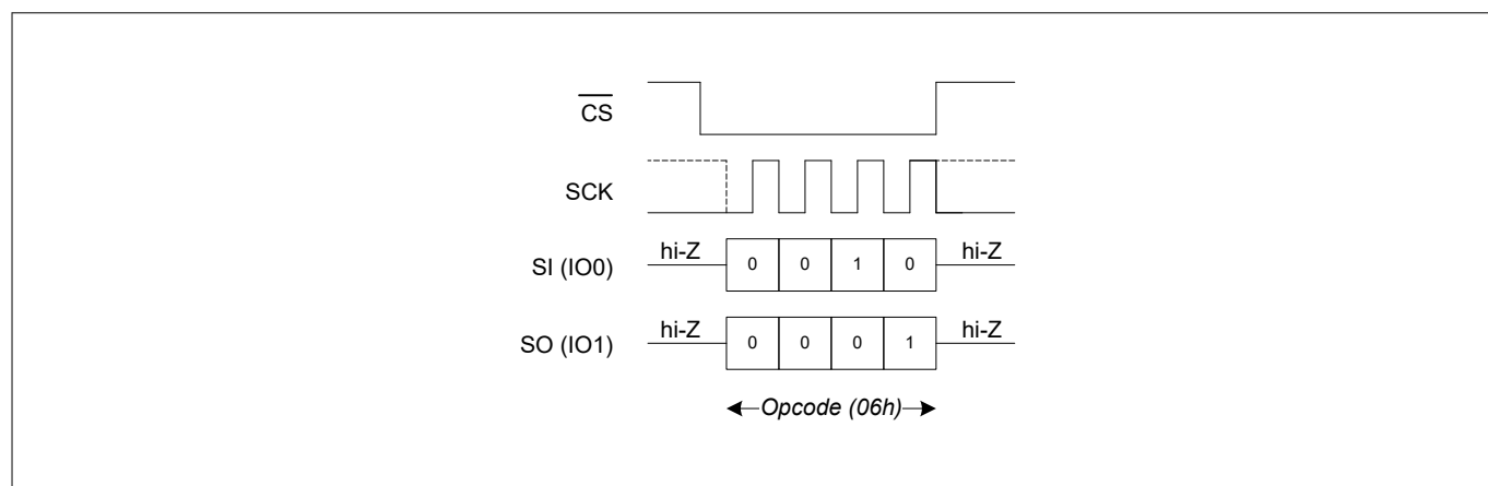
Figure 9 WREN bus configuration in DPI mode
