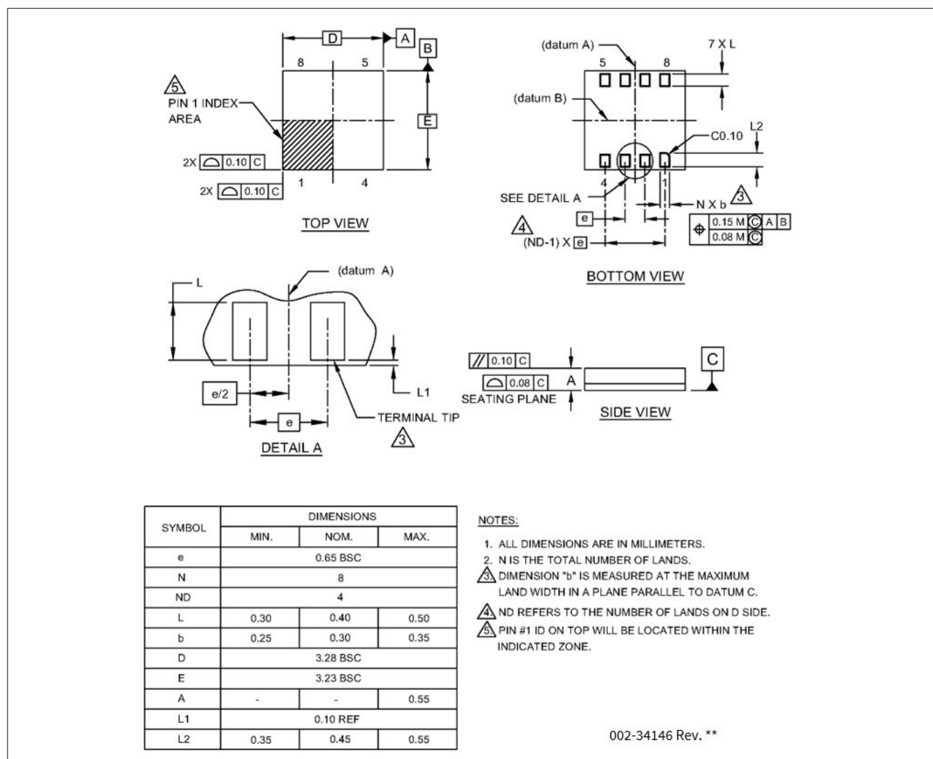
Figure 126 8-pin UFLGA (3.28 × 3.23 × 0.55 mm) BF08A package outline, 002-34146
