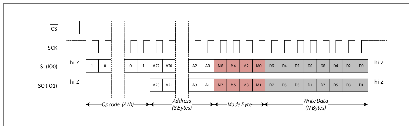
Figure 50 Dual I/O write (DIOW)
