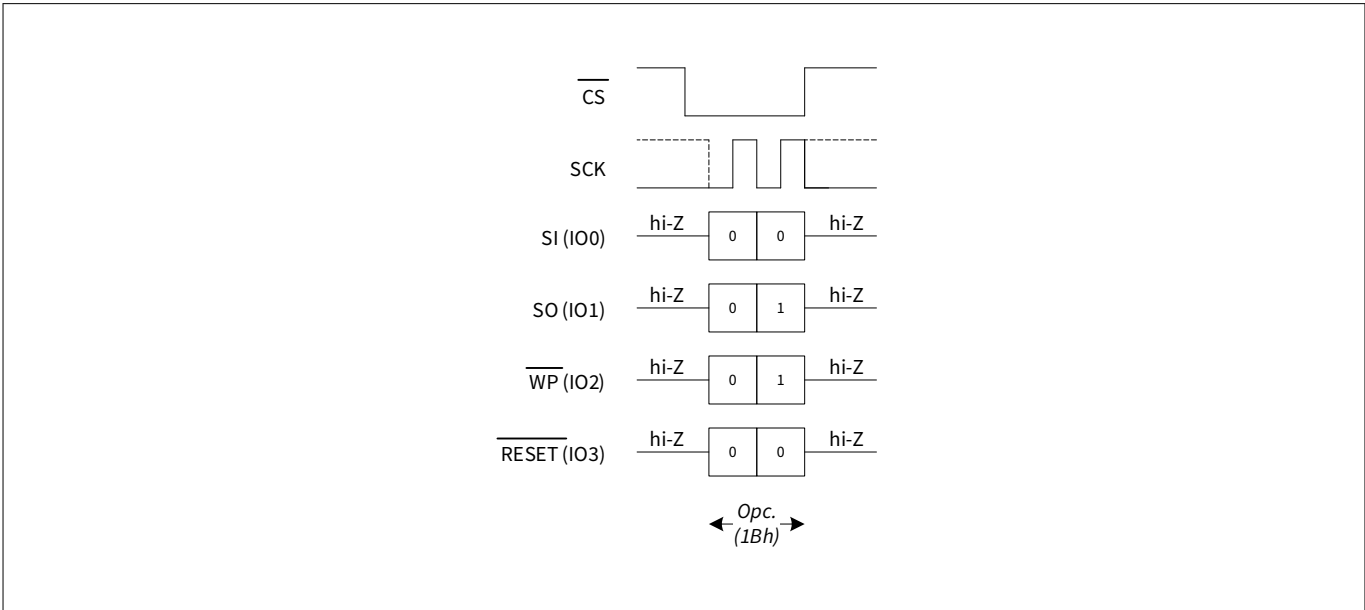
Figure 79 Clear ECC (CLECC) in QPI mode
