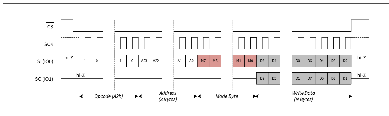
Figure 49 Dual input write (DIW)
