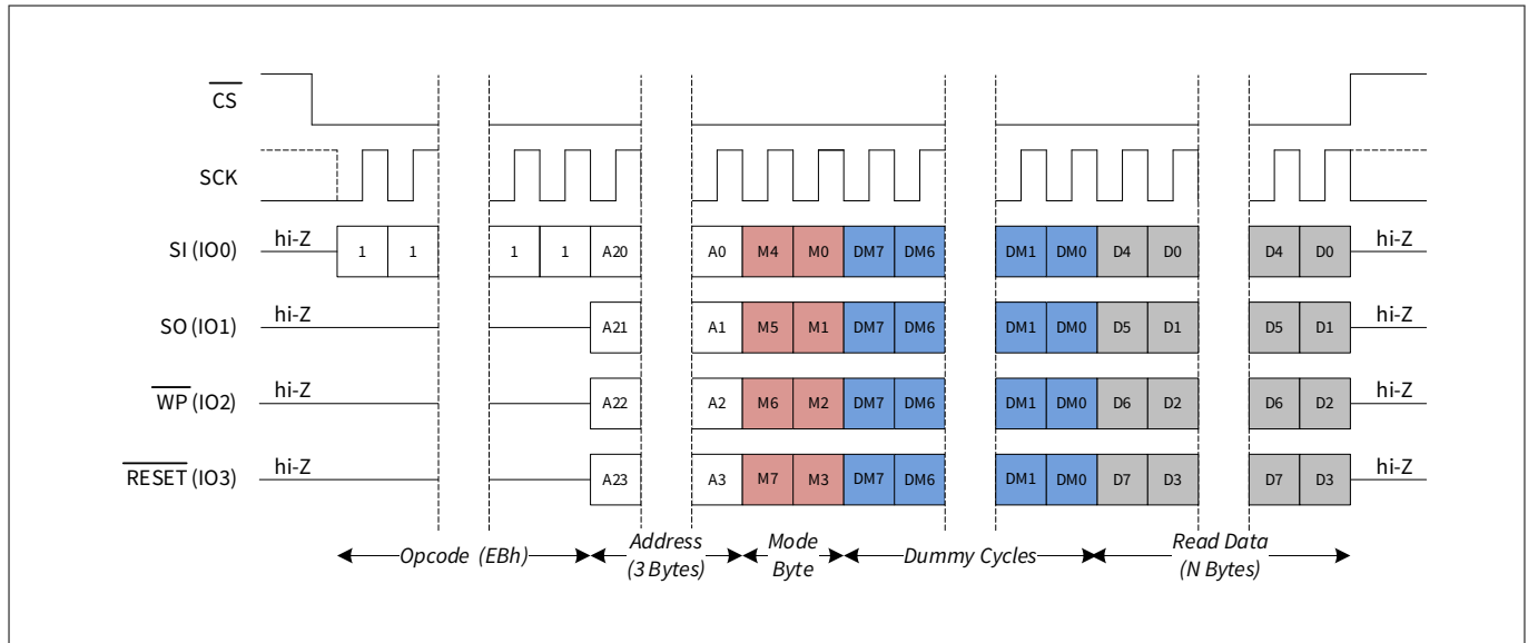
Figure 64 Quad I/O read (QIOR) in extended SPI mode
