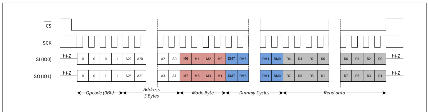
Figure 58 FAST_READ in DPI mode
