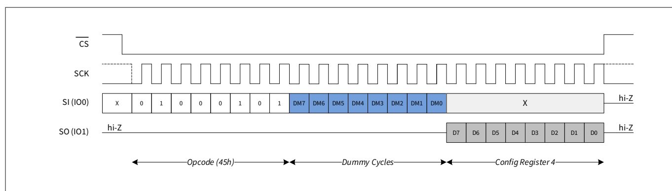
Figure 29 Read CR4 (RDCR4) in SPI mode
