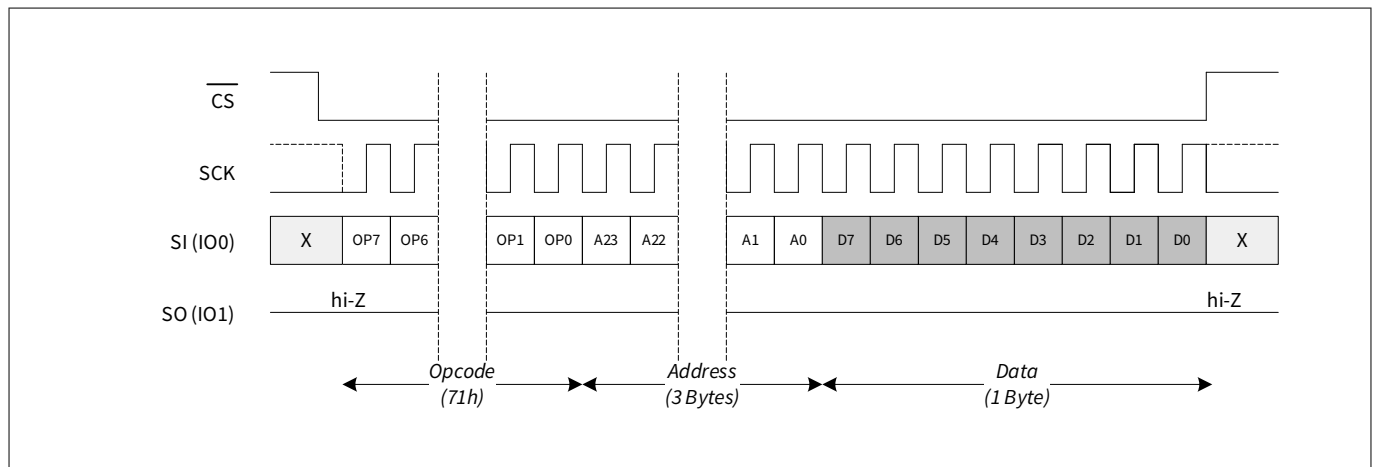
Figure 35 Write any register (WRAR) in SPI mode
