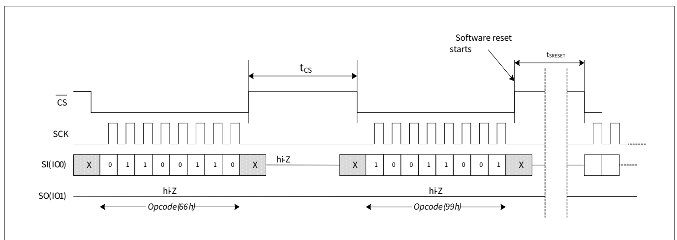
Figure 108 Software reset timing in SPI mode
