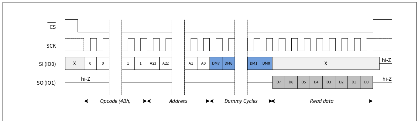
Figure 71 Special sector read (SSRD) in SPI mode
