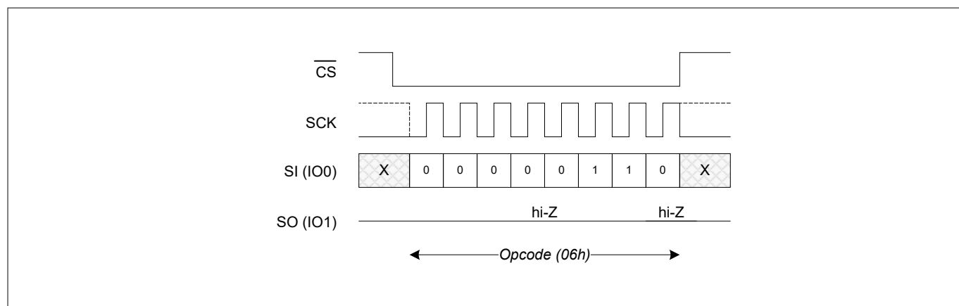
Figure 8 WREN bus configuration in SPI mode
