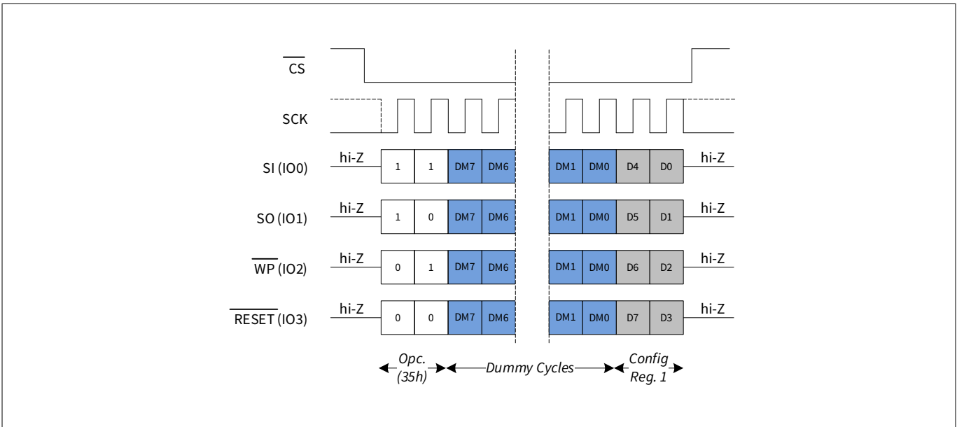
Figure 25 Read CR1 (RDCR1) in QPI mode
