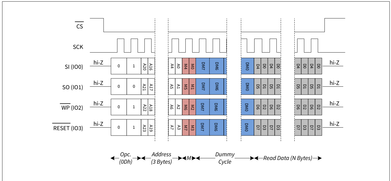
Figure 60 DDRFR in QPI mode
