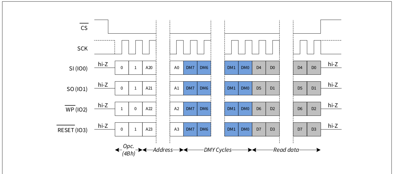
Figure 73 Special sector read (SSRD) in QPI mode
