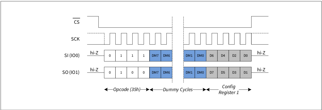
Figure 24 Read CR1 (RDCR1) in DPI mode
