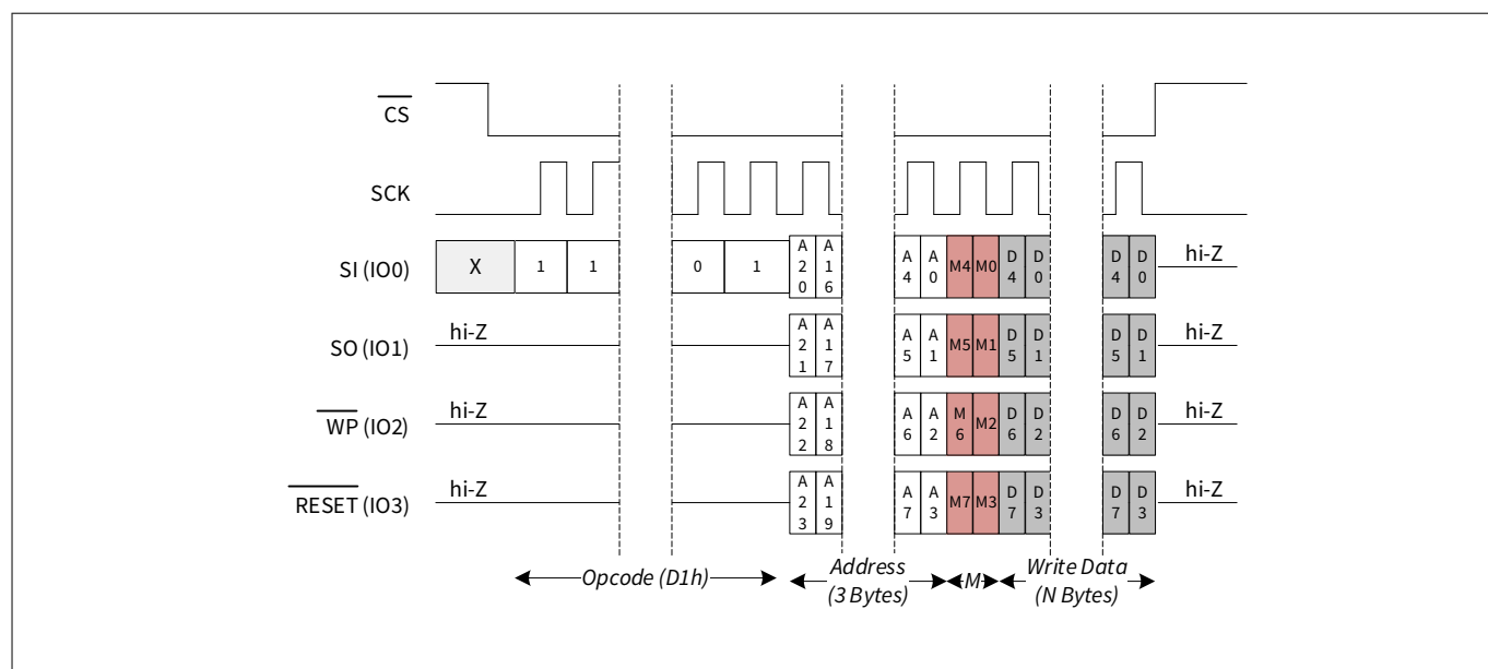
Figure 53 Quad I/O write (QIOW)
