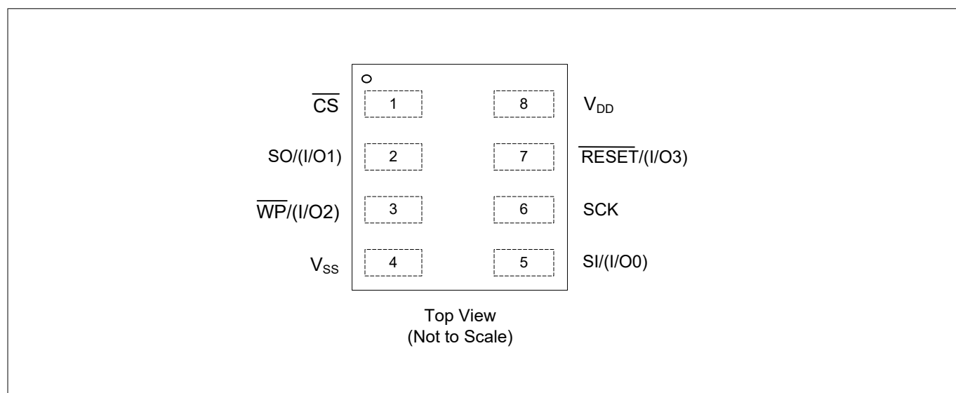
Figure 3 8-pin GQFN/UFLGA pinout
