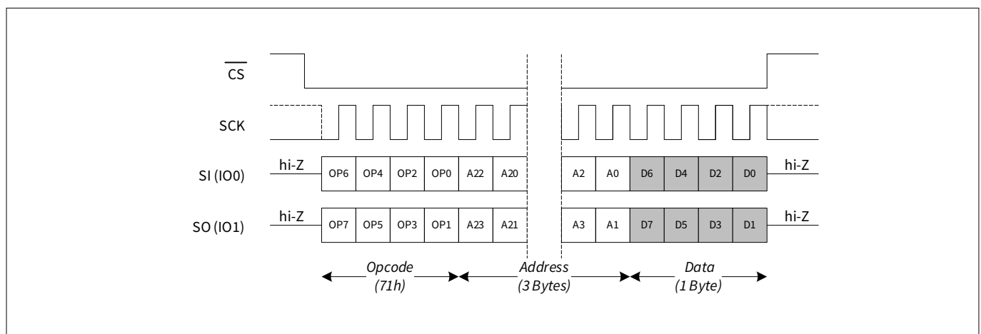
Figure 36 Write any register (WRAR) in DPI mode
