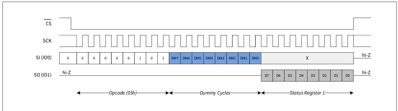
Figure 17 Read SR1 (RDSR1) in SPI mode
