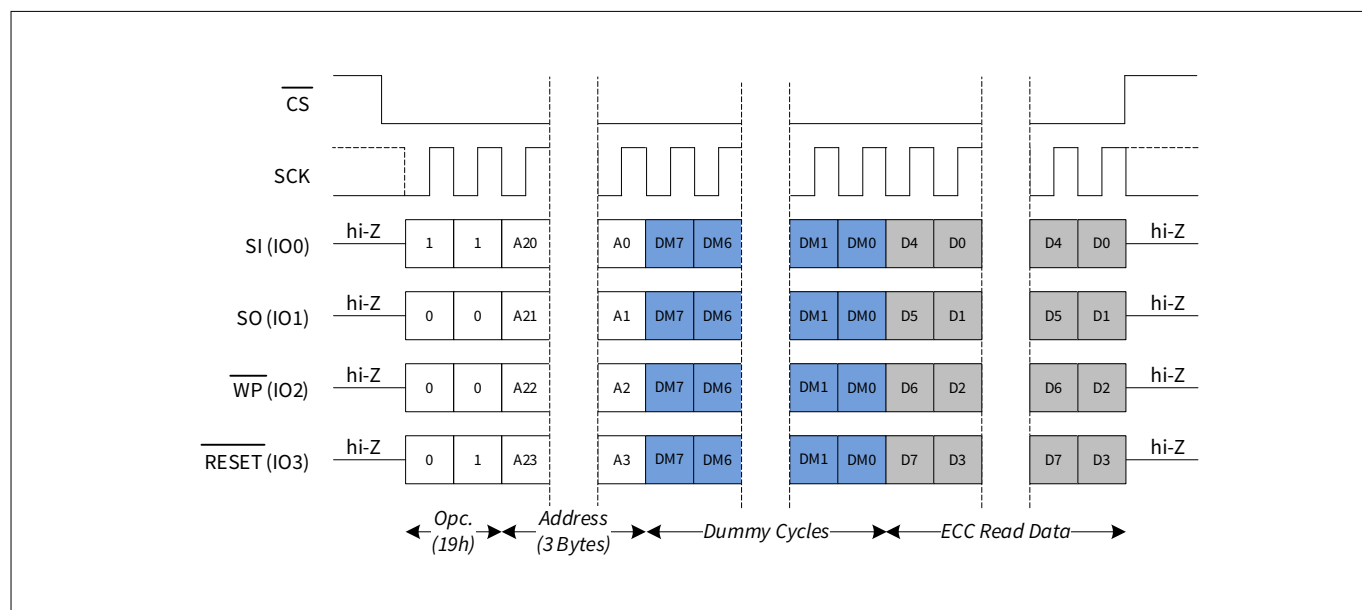
Figure 76 ECC read (ECCRD) in QPI mode
