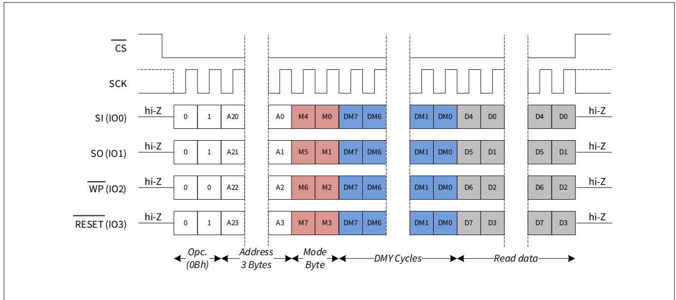
Figure 59 FAST_READ in QPI mode
