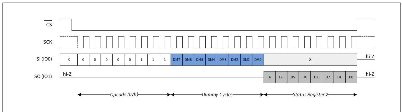
Figure 20 Read SR2 (RDSR2) in SPI mode
