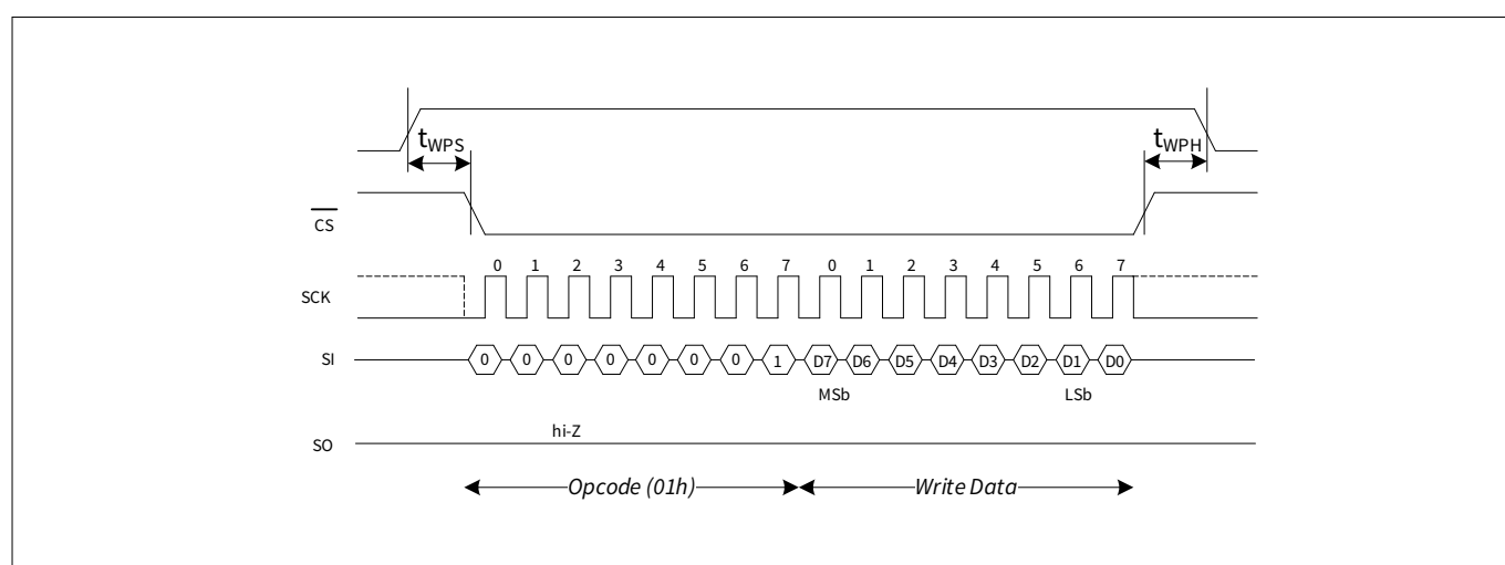
Figure 121 Write protect setup and hold timing
