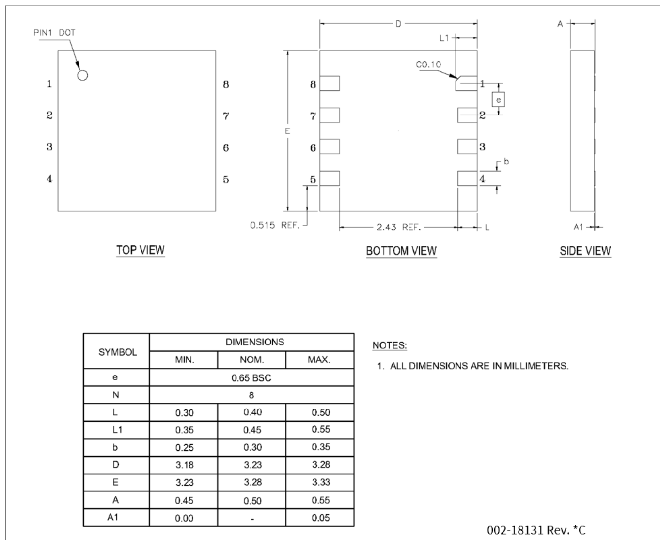
Figure 125 8-pin GQFN (3.23 × 3.28 × 0.55 mm) LP08A package outline, (PG-VQFN-8), 002-18131
