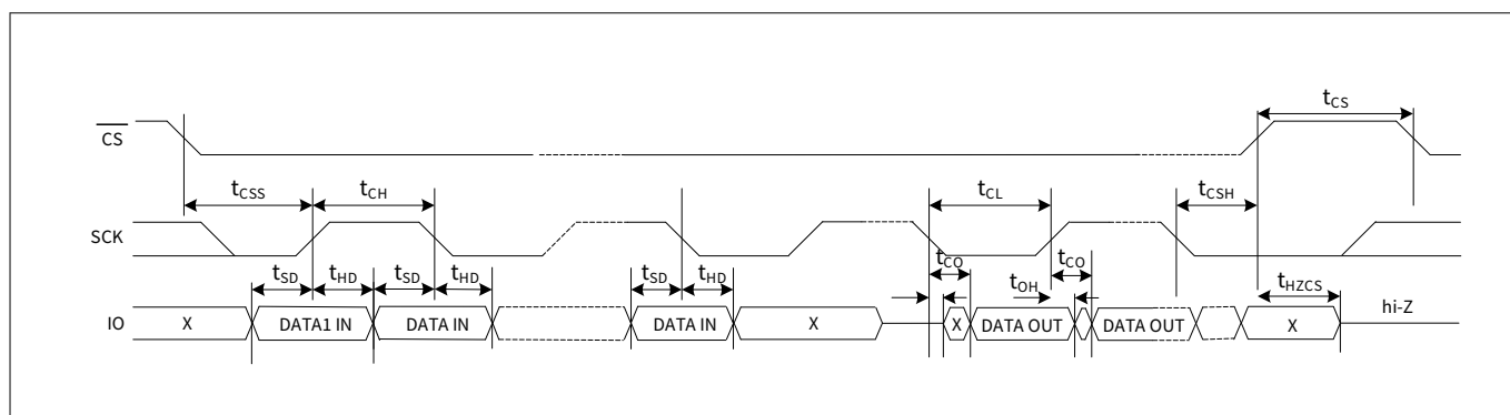
Figure 120 SPI switching timing - multiple I/O, DDR 2)
