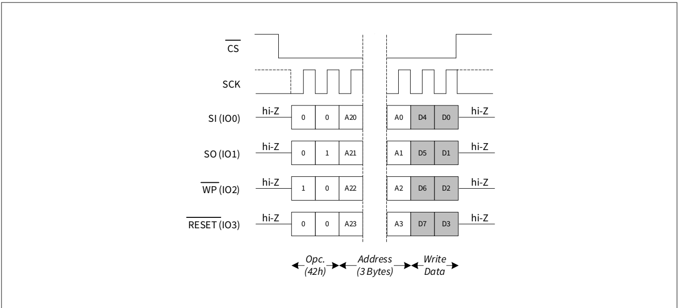
Figure 70 Special sector write (SSWR) in QPI mode (WREN is not shown)
