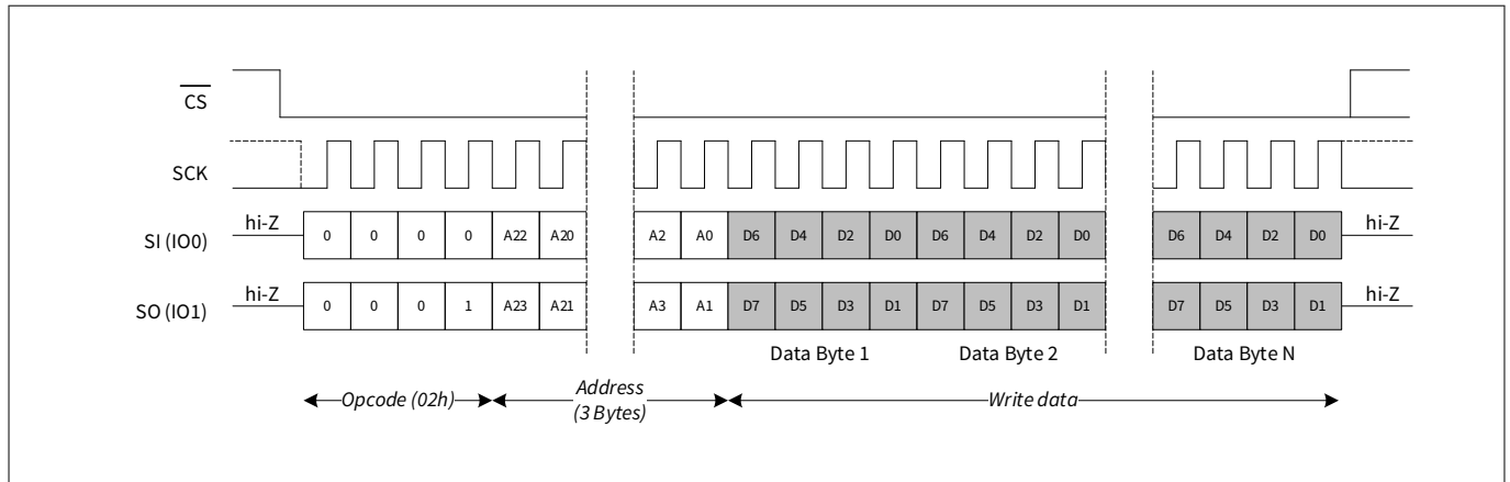
Figure 42 Memory write (WRITE) in DPI mode
