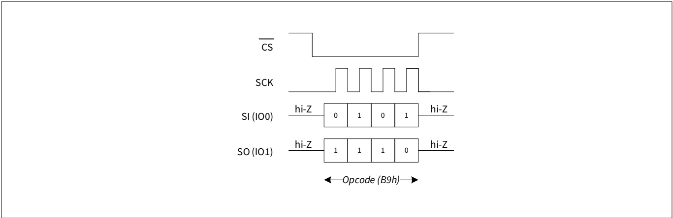
Figure 102 Deep power-down mode operation in DPI mode
