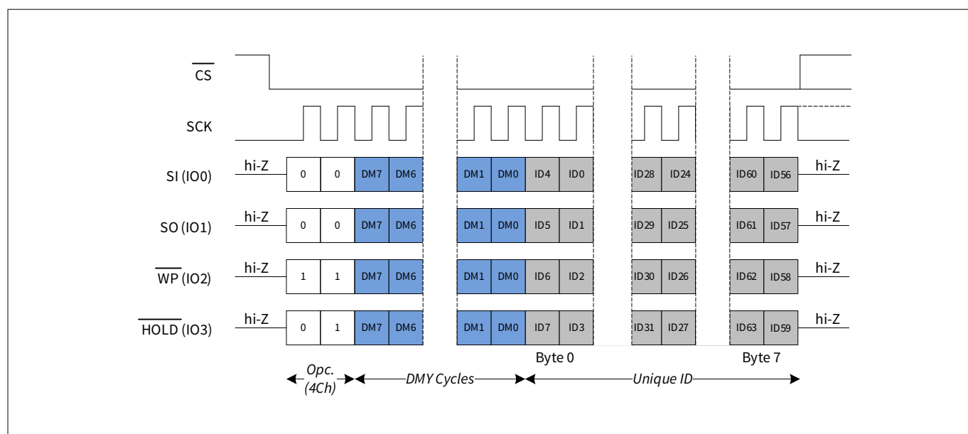
Figure 94 Read unique ID in QPI mode
