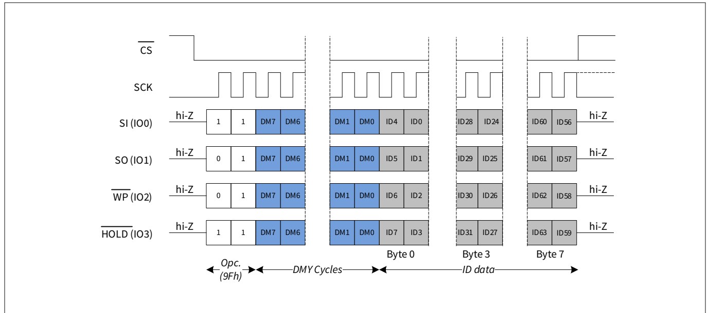
Figure 91 Read device ID (RDID) in QPI mode
