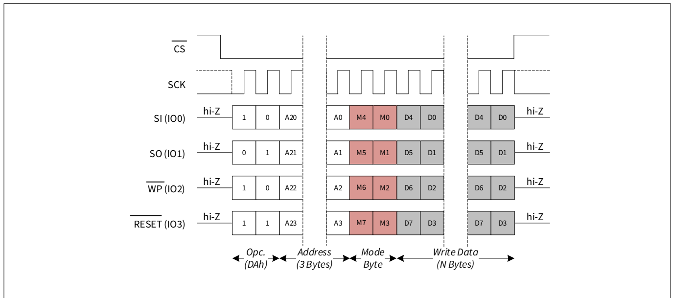
Figure 47 Fast write (FAST_WRITE) in QPI mode
