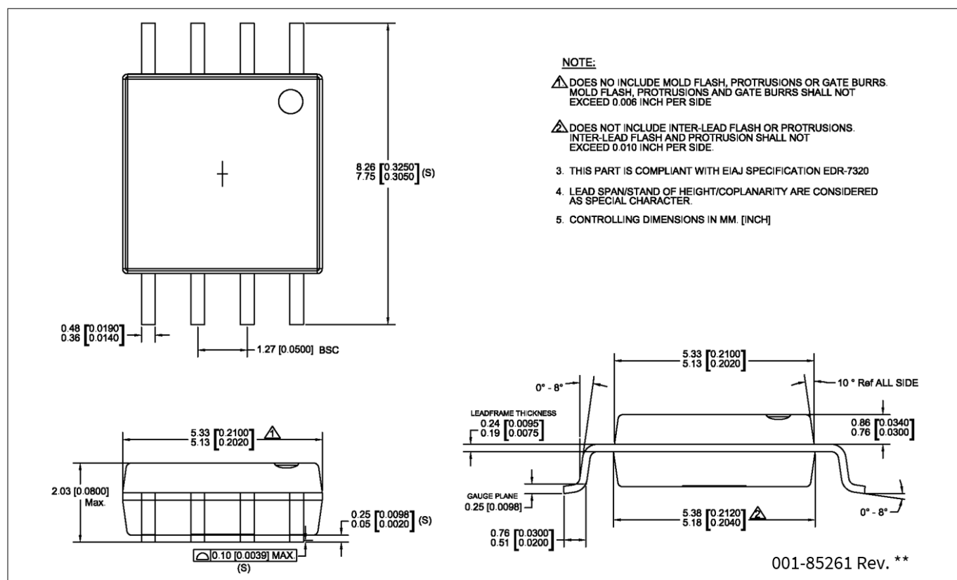
Figure 124 8-pin SOIC (208 Mils) SZ820 package outline, (PG-DSO-8), 001-85261
