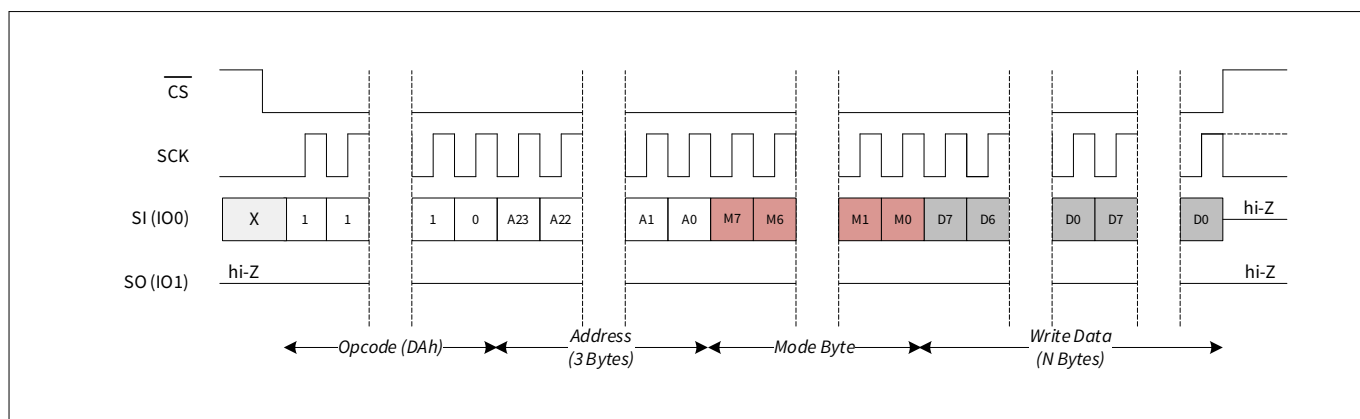
Figure 45 Fast write (FAST_WRITE) in SPI mode
