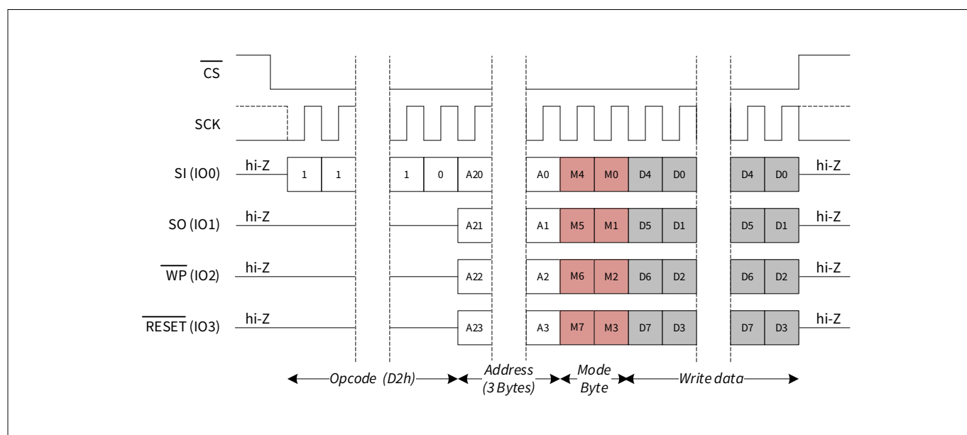
Figure 52 Quad I/O write (QIOW)
