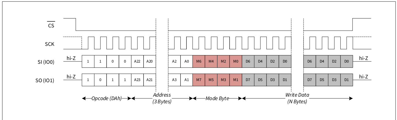
Figure 46 Fast write (FAST_WRITE) in DPI mode
