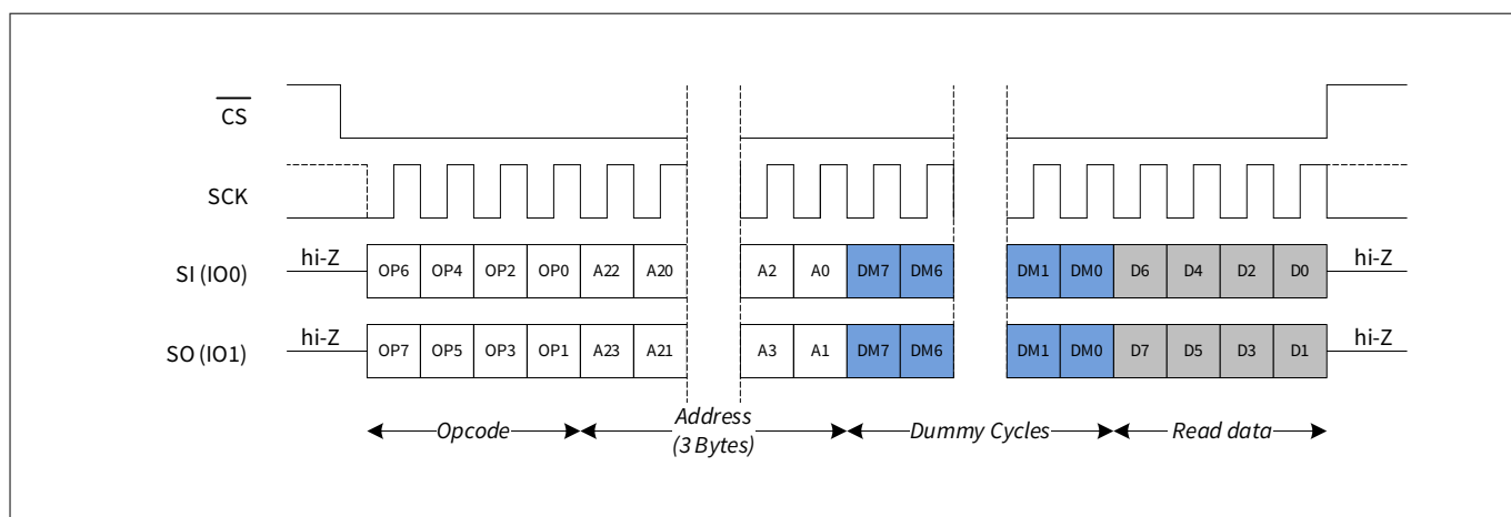
Figure 39 Read any register (RDAR) in DPI mode
