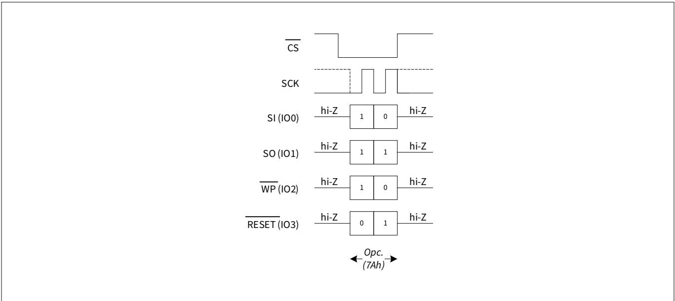
Figure 88 CRC resume (EPCR) in QPI mode
