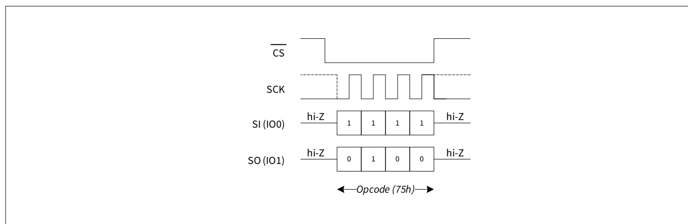
Figure 84 CRC suspend (EPCS) in DPI mode
