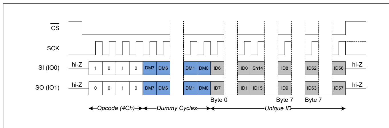
Figure 93 Read unique ID in DPI mode
