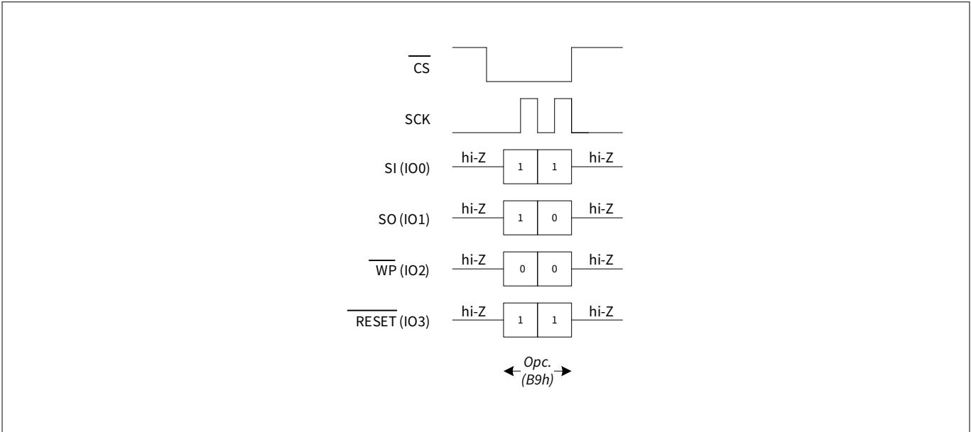
Figure 103 Deep power-down mode operation in QPI mode
