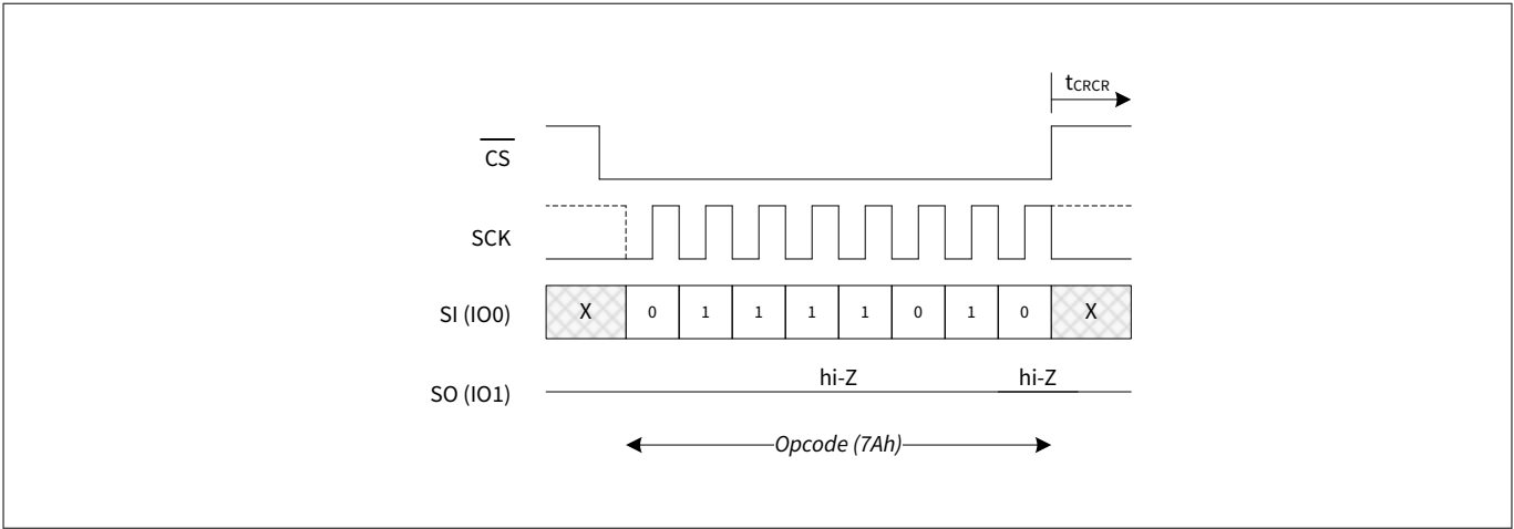
Figure 86 CRC resume (EPCR) in SPI mode
