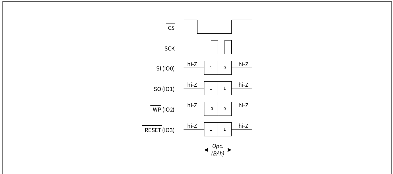
Figure 107 Hibernate mode operation in QPI mode
