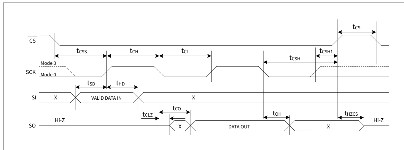
Figure 116 SPI switching timing - single IO, SDR (mode 0 and mode 3)
