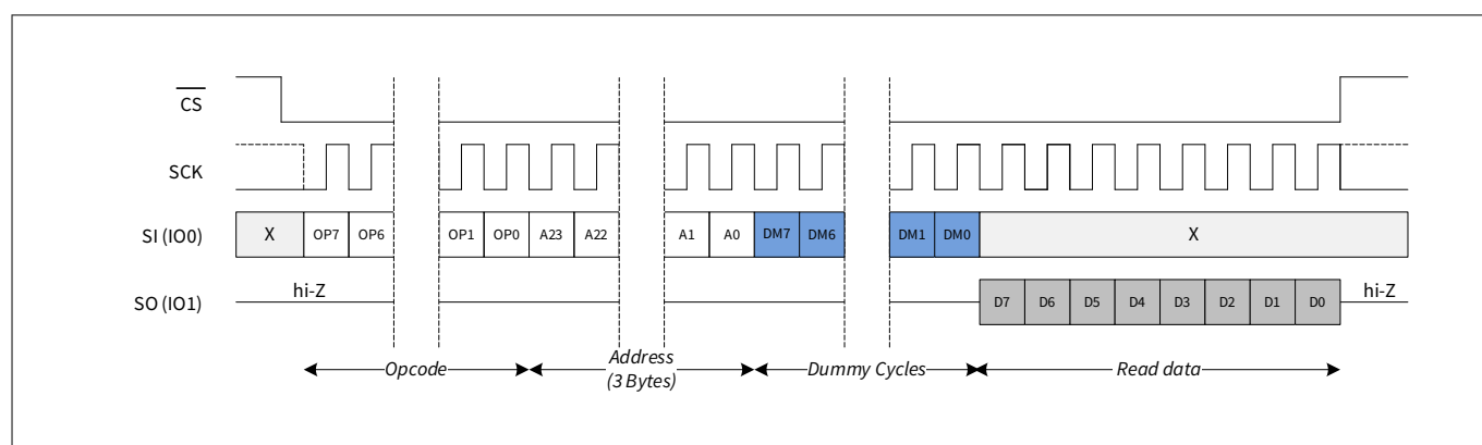
Figure 38 Read any register (RDAR) in SPI mode
