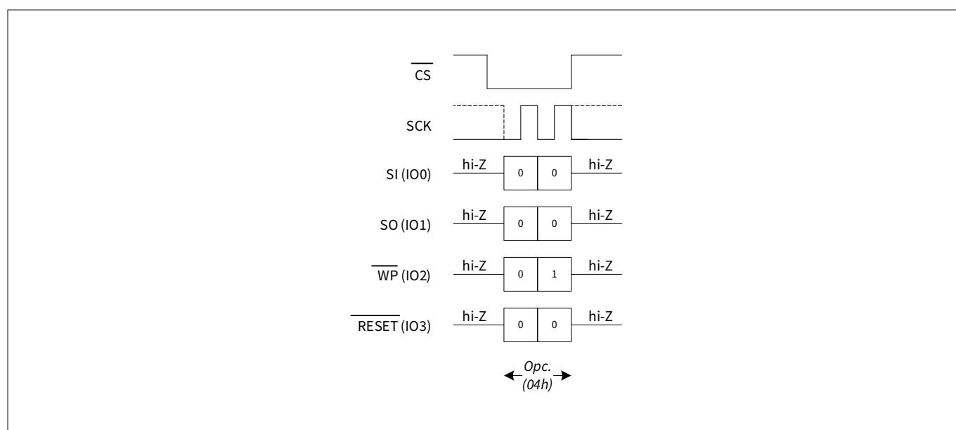
Figure 13 WRDI bus configuration in QPI mode
