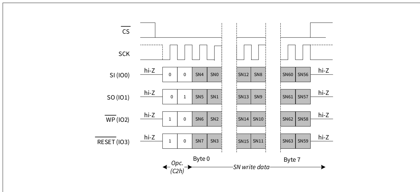
Figure 97 Write serial number in QPI mode (WREN not shown)
