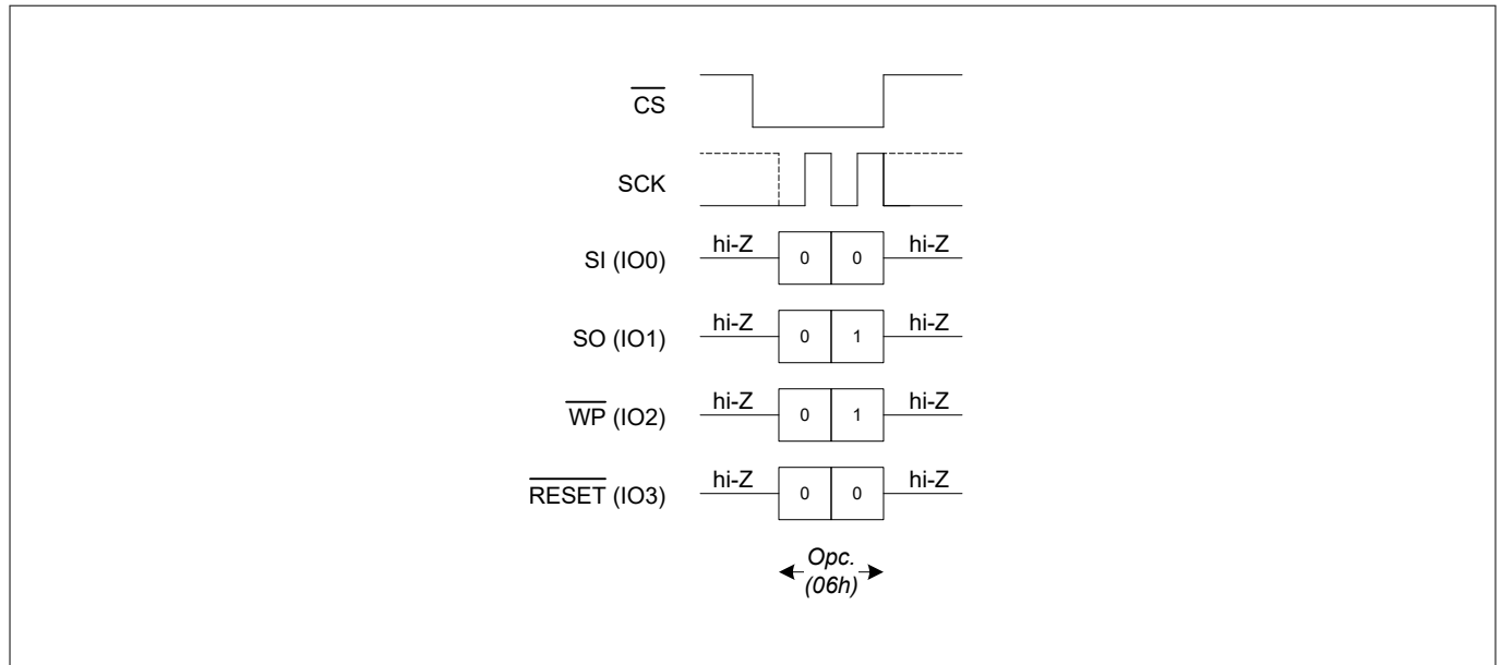
Figure 10 WREN bus configuration in QPI mode
