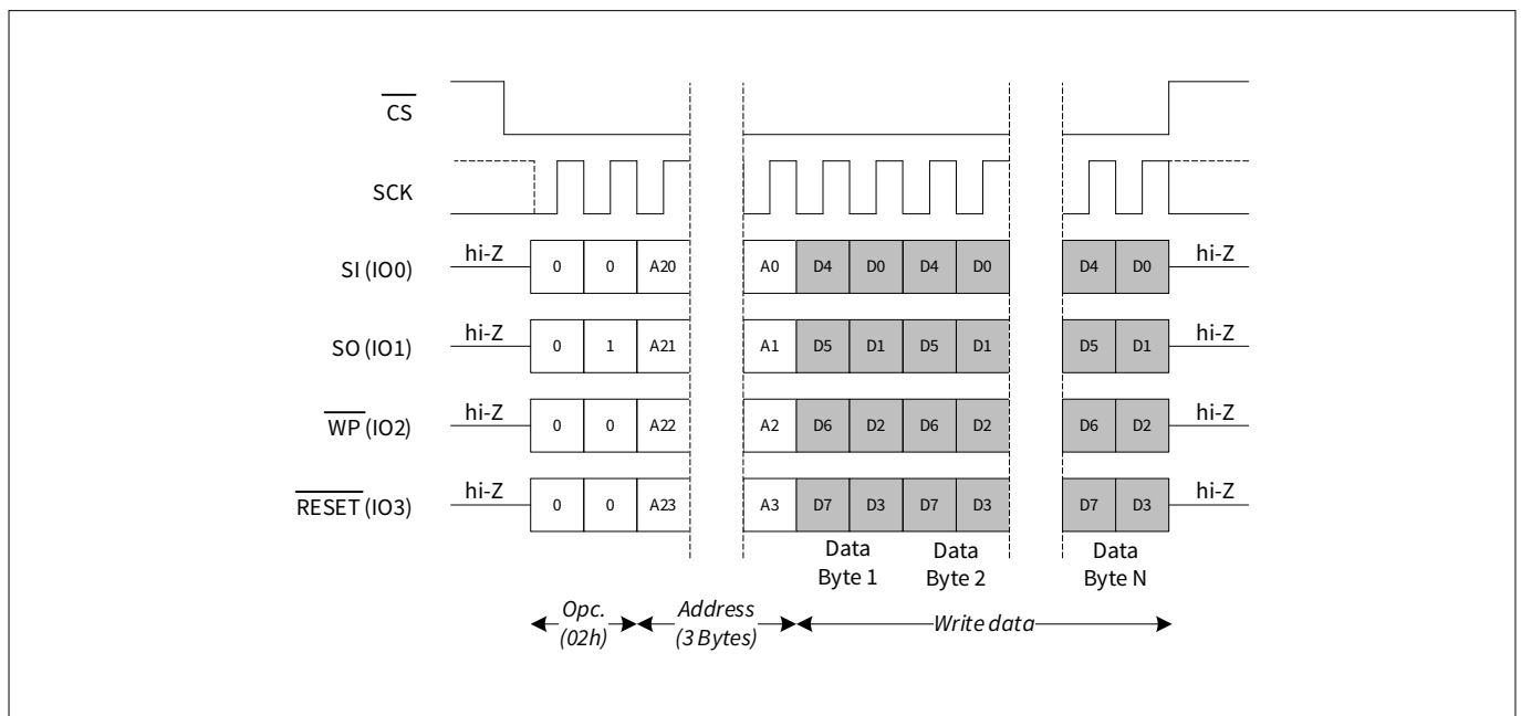
Figure 43 Memory write (WRITE) in QPI mode
