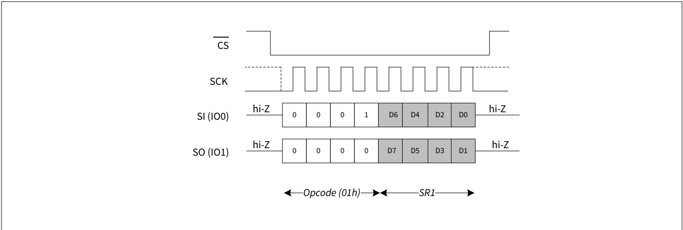
Figure 15 WRSR in DPI mode (WREN not shown)
