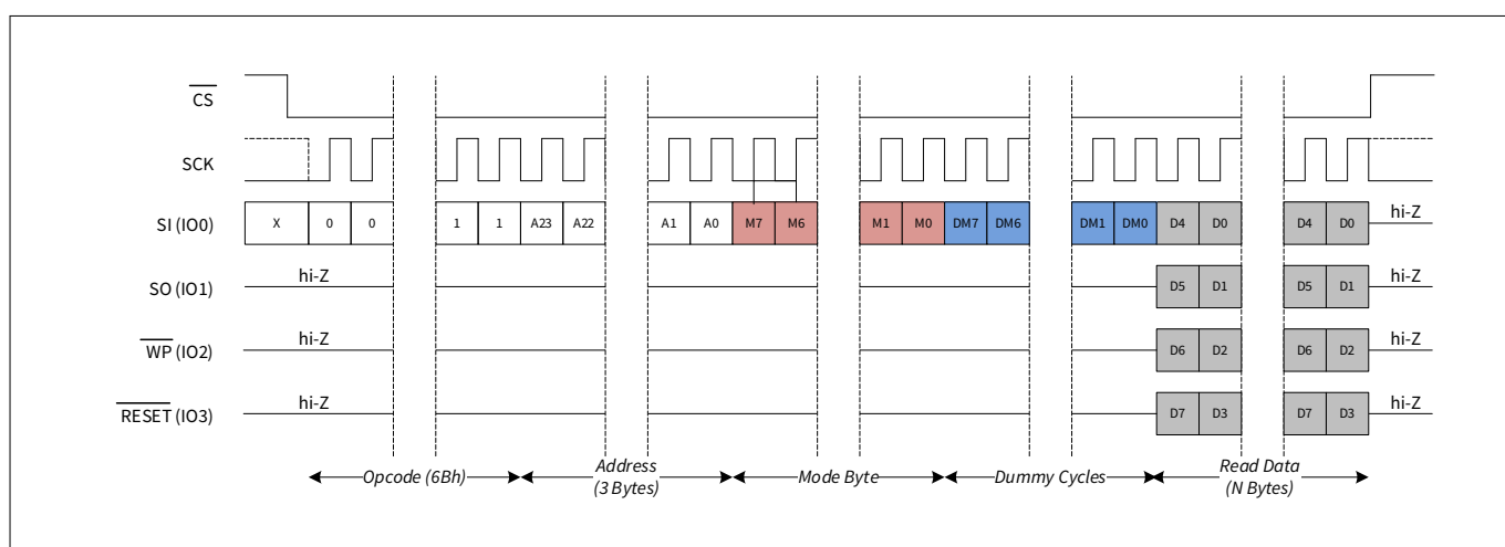
Figure 63 Quad output read (QOR)
