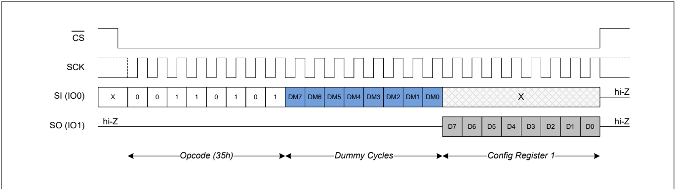
Figure 23 Read CR1 (RDCR1) in SPI mode
