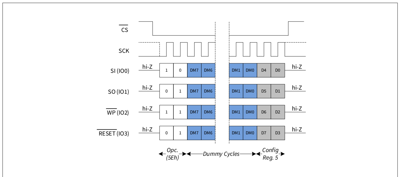
Figure 34 Read CR5 (RDCR5) in QPI mode
