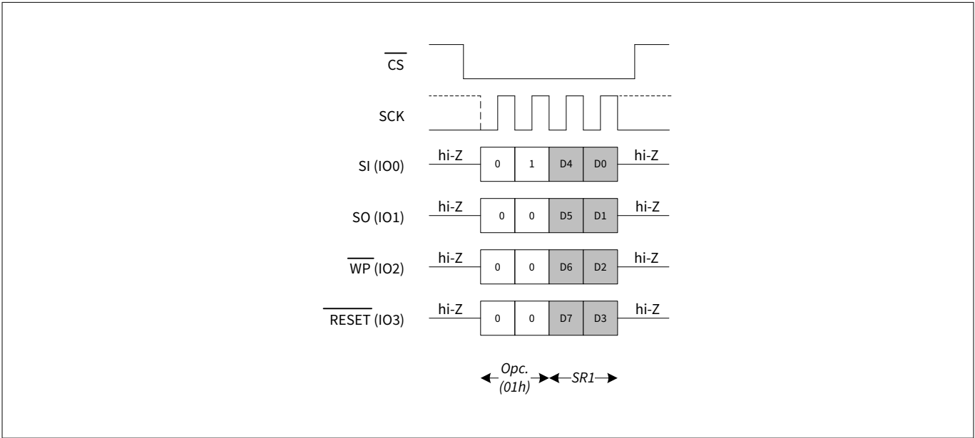
Figure 16 WRSR in QPI mode (WREN not shown)
