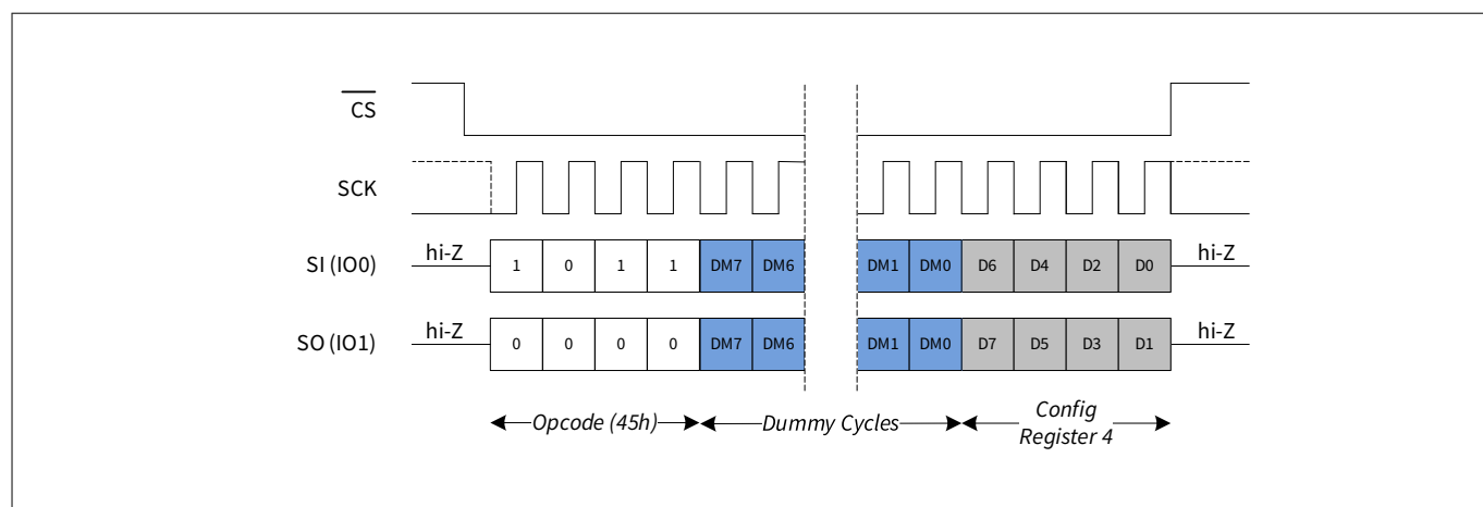
Figure 30 Read CR4 (RDCR4) in DPI mode
