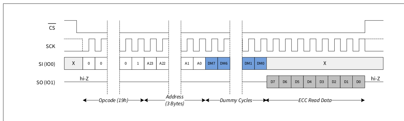
Figure 74 ECC read (ECCRD) in SPI mode
