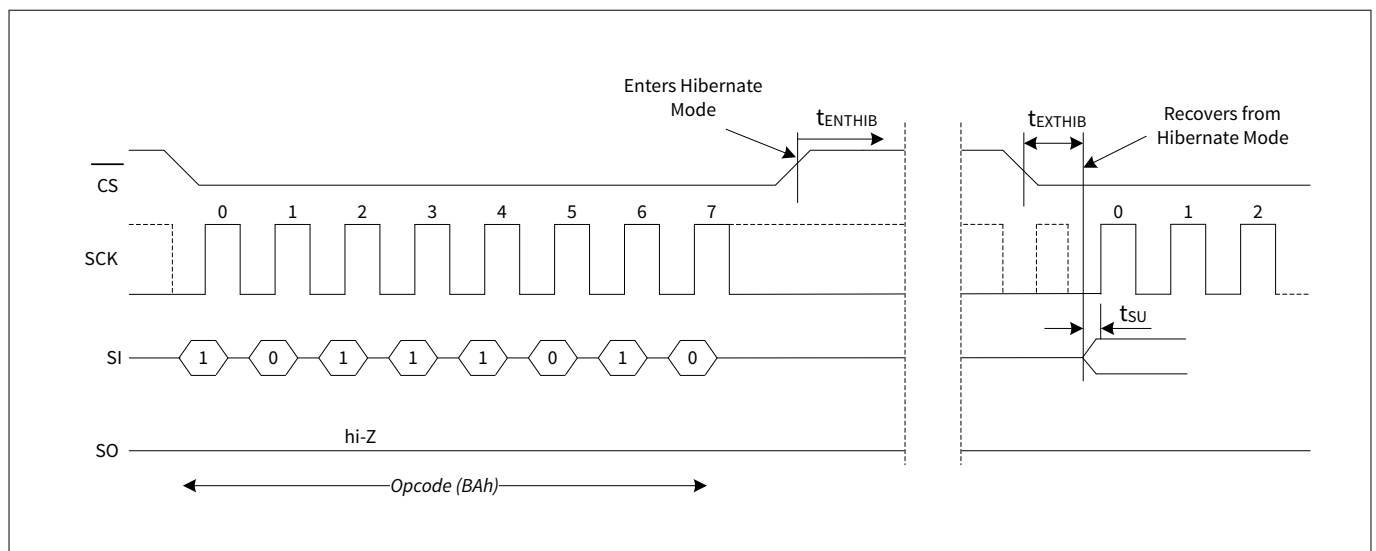
Figure 105 Hibernate mode operation in SPI mode
