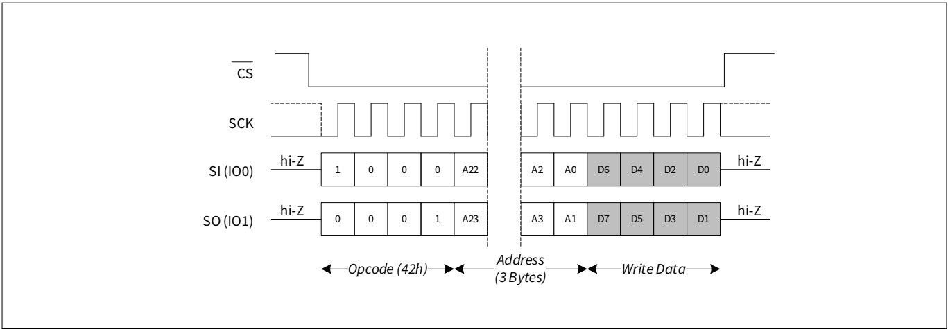
Figure 69 Special sector write (SSWR) in DPI mode (WREN is not shown)
