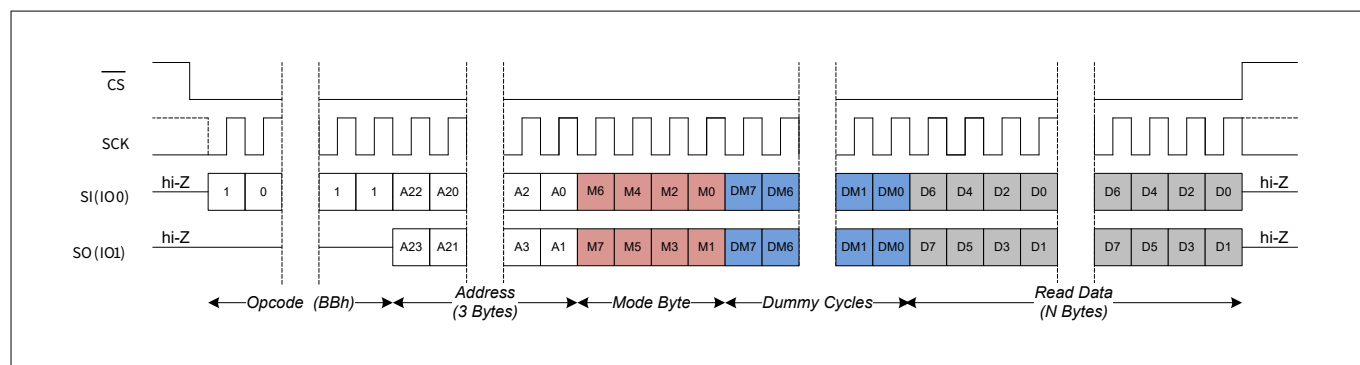
Figure 62 Double I/O read (DIOR)
