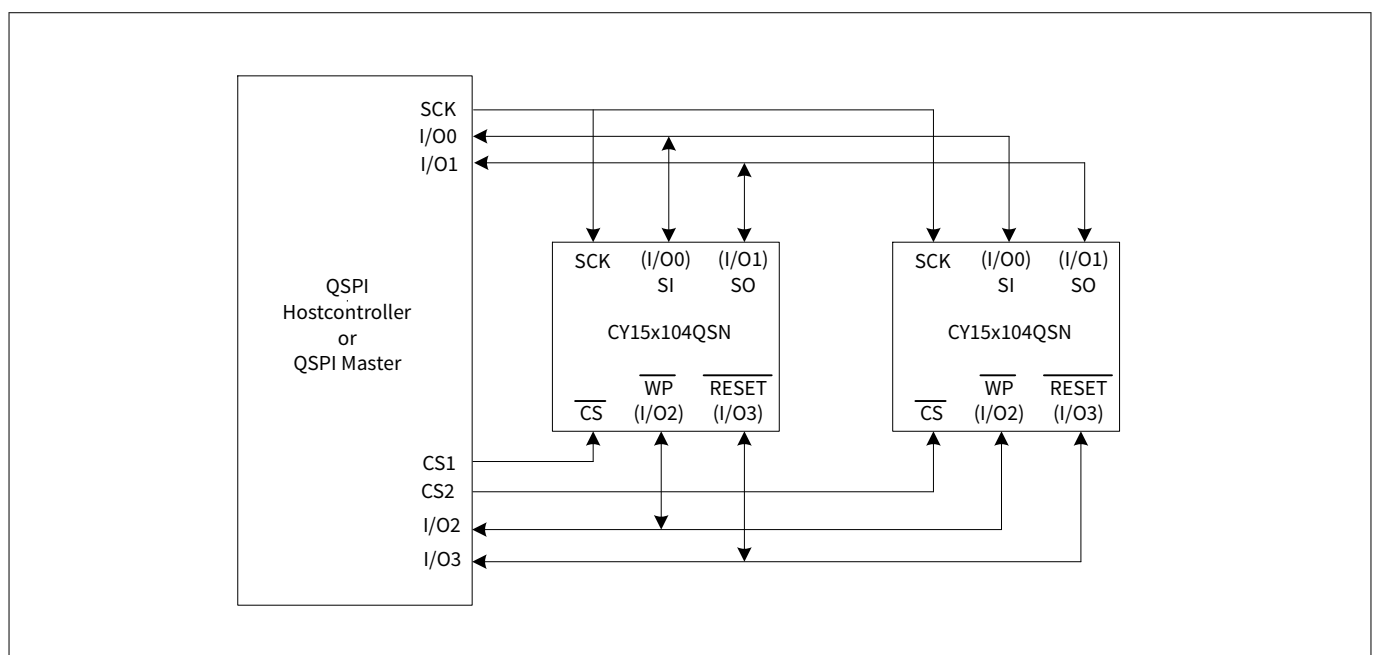
Figure 5 System configuration with QSPI port
