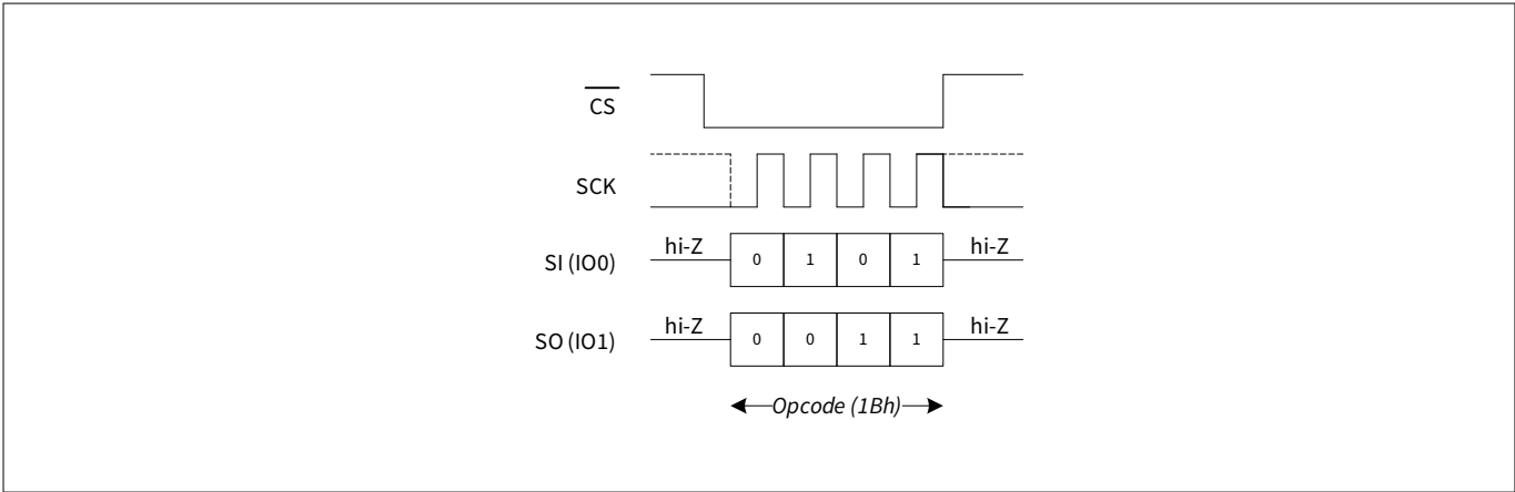
Figure 78 Clear ECC (CLECC) in DPI mode
