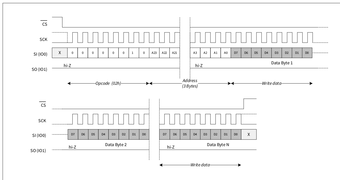
Figure 41 Memory write (WRITE) in SPI mode
