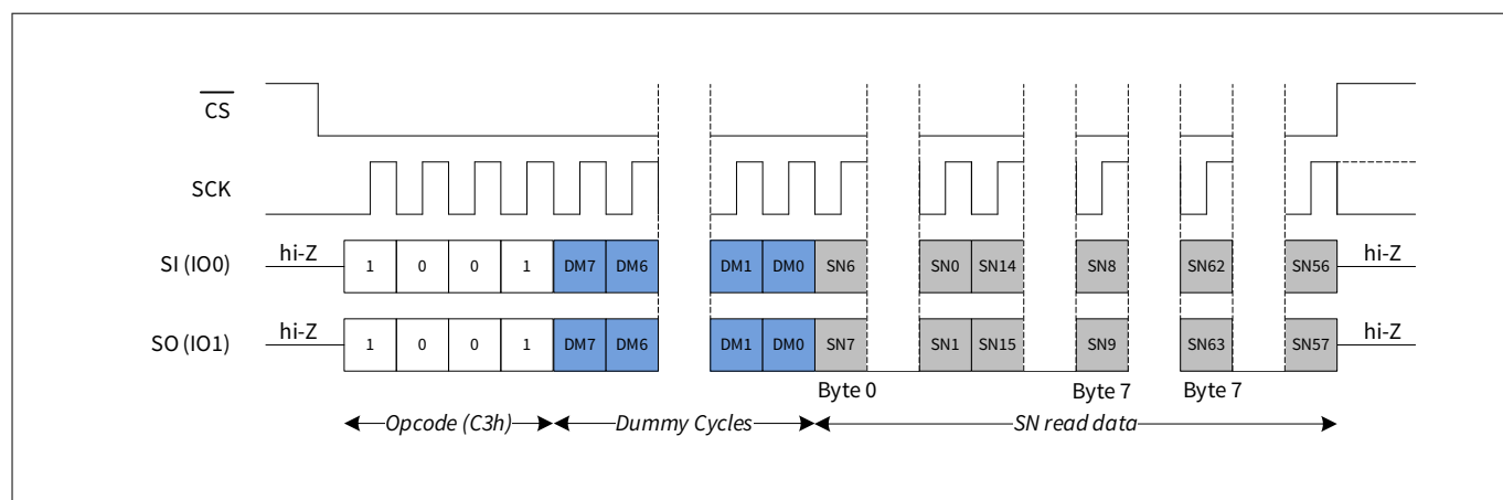
Figure 99 Read serial number (RDSN) in DPI mode
