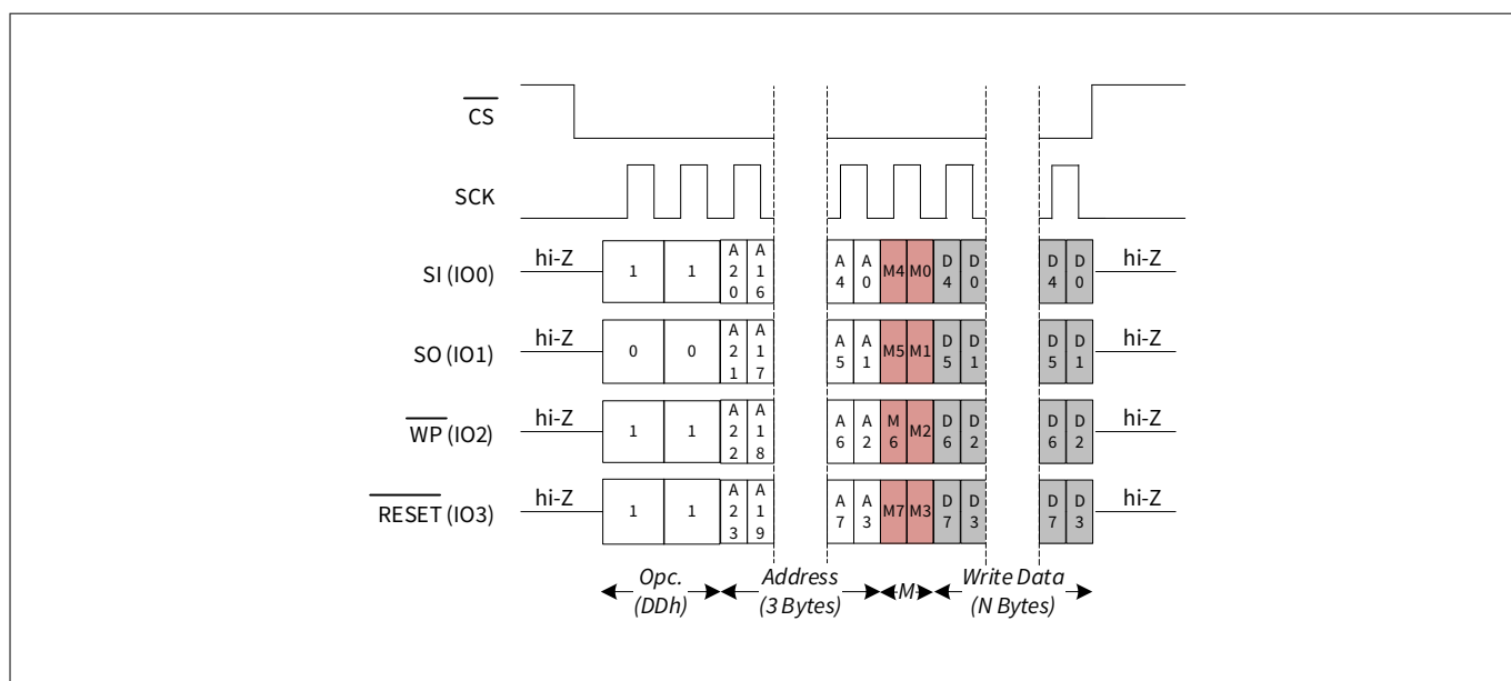
Figure 48 DDR fast write (DDR_FAST_WRITE) in QPI mode
