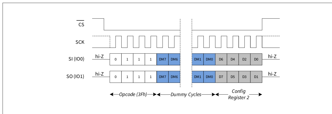
Figure 27 Read CR2 (RDCR2) in DPI mode
