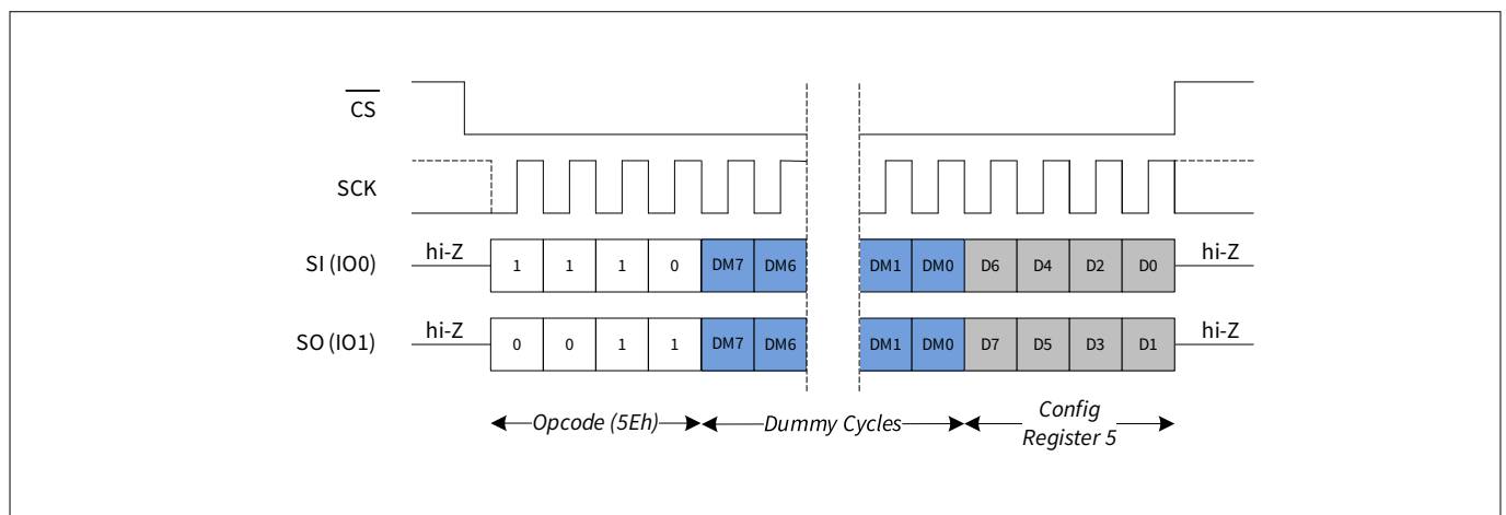
Figure 33 Read CR5 (RDCR5) in DPI mode
