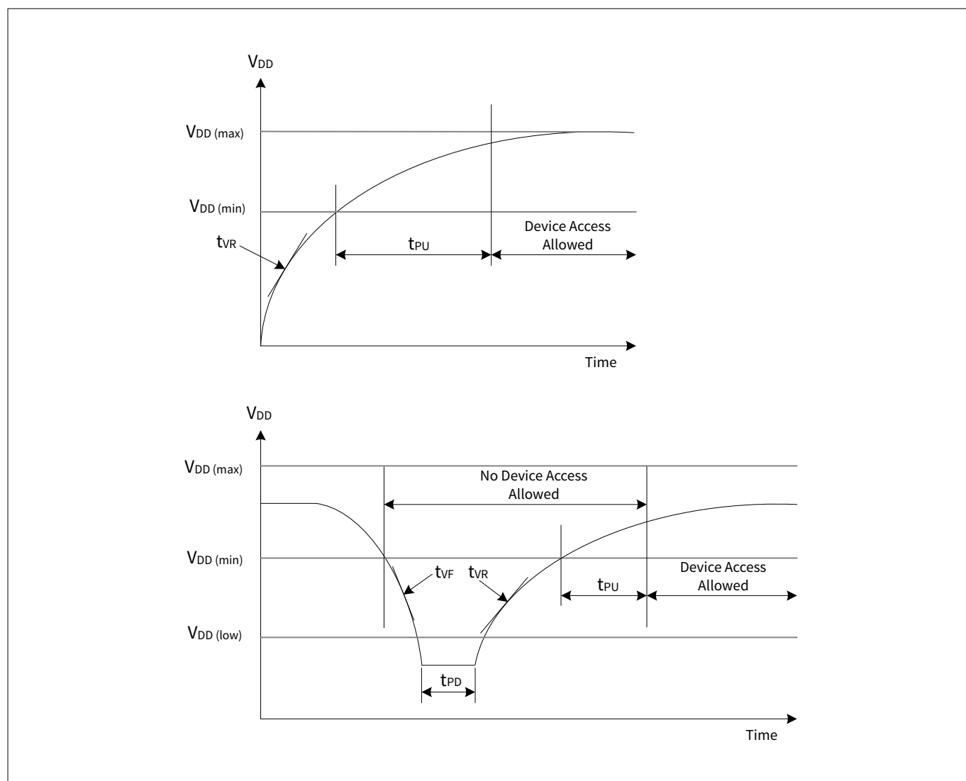
Figure 122 Power cycle timing
