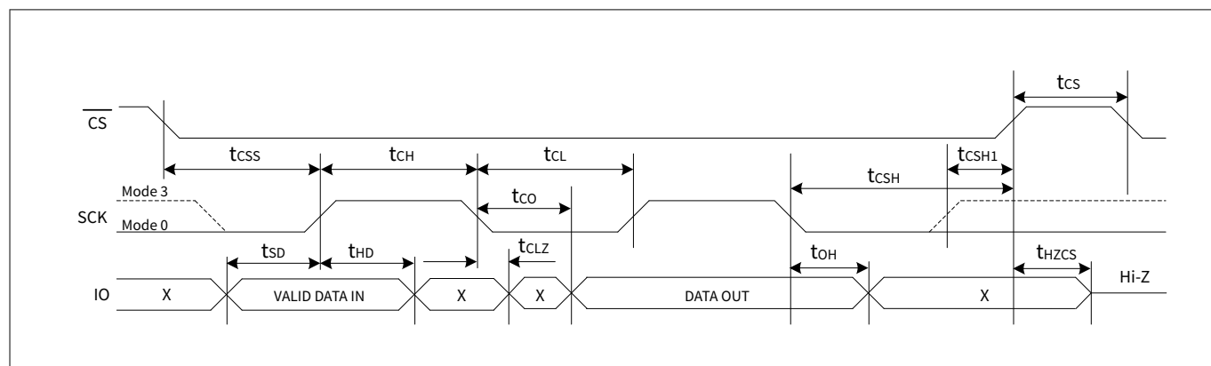
Figure 117 SPI switching timing - multiple I/O, SDR (mode 0 and mode 3)
