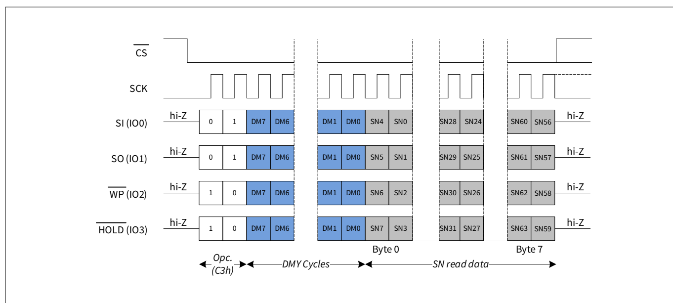
Figure 100 Read serial number (RDSN) in QPI mode
