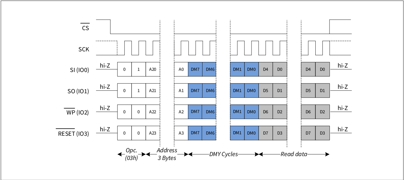
Figure 56 READ in QPI mode
