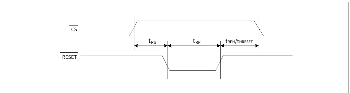
Figure 112 RESET timing - SPI with QUAD clear (CR1[1]='0') and QPI disabled (CR2[6]='0')
