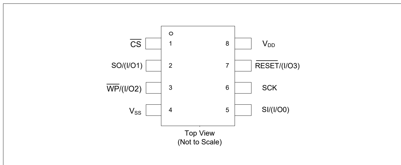
Figure 2 8-pin SOIC pinout
