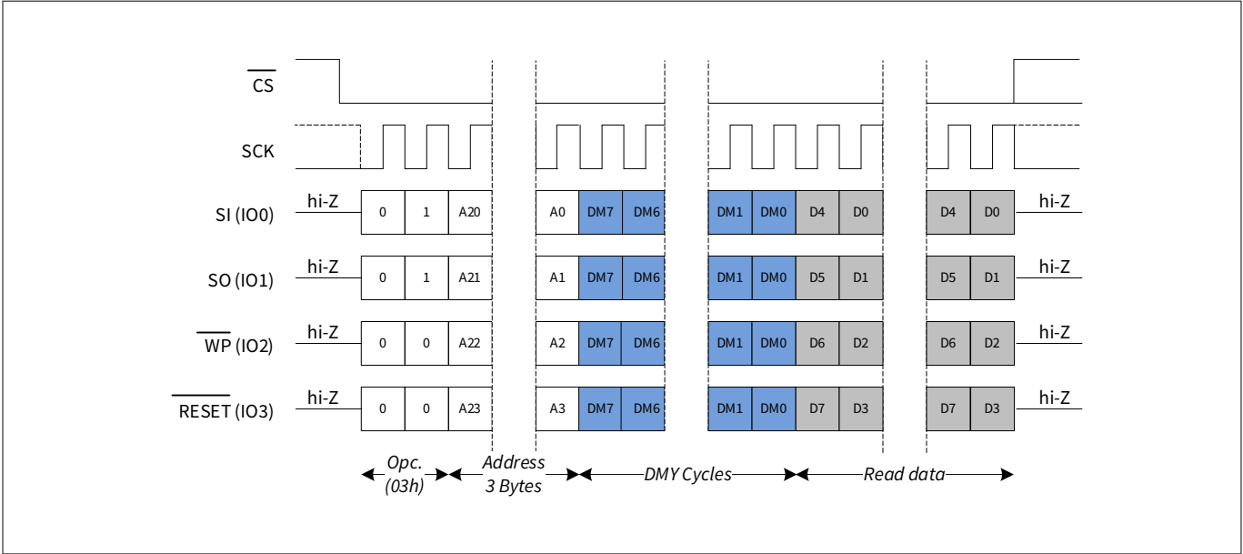
Figure 55 READ in DPI mode
