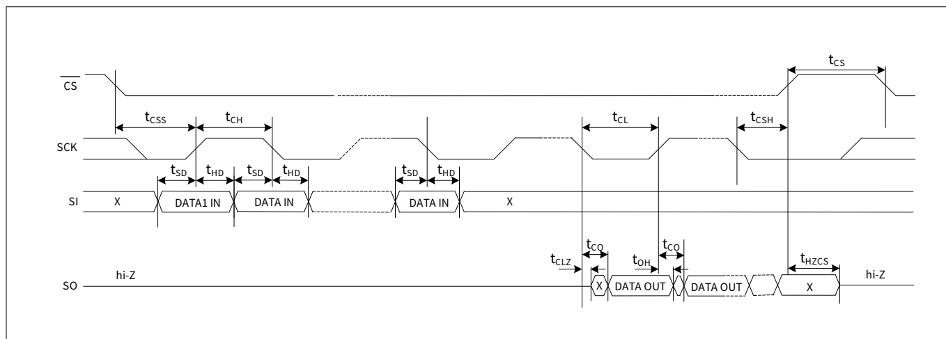
Figure 119 SPI switching timing - single I/O, DDR
