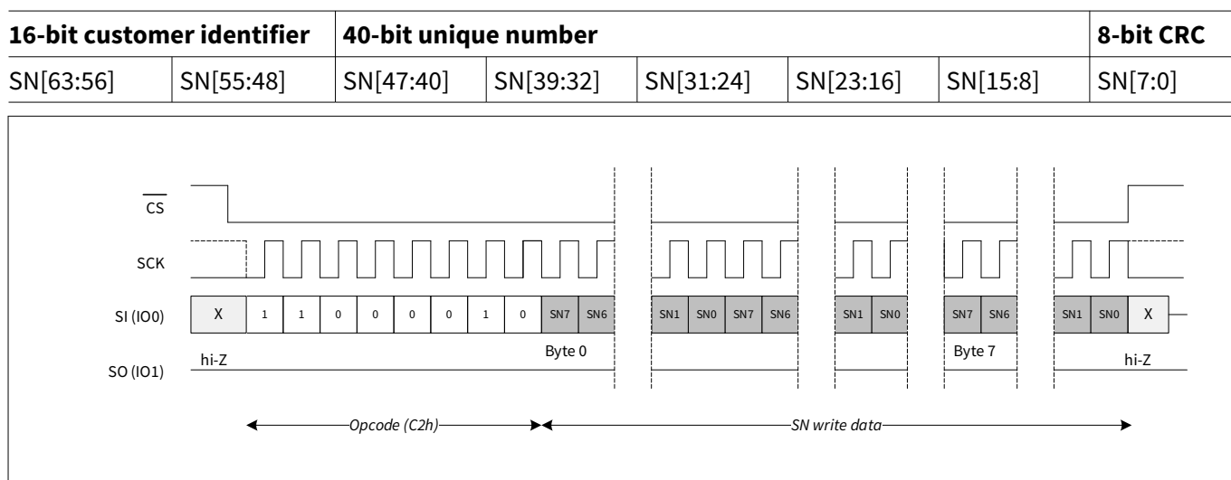
Figure 95 Write serial number in SPI mode (WREN not shown)
