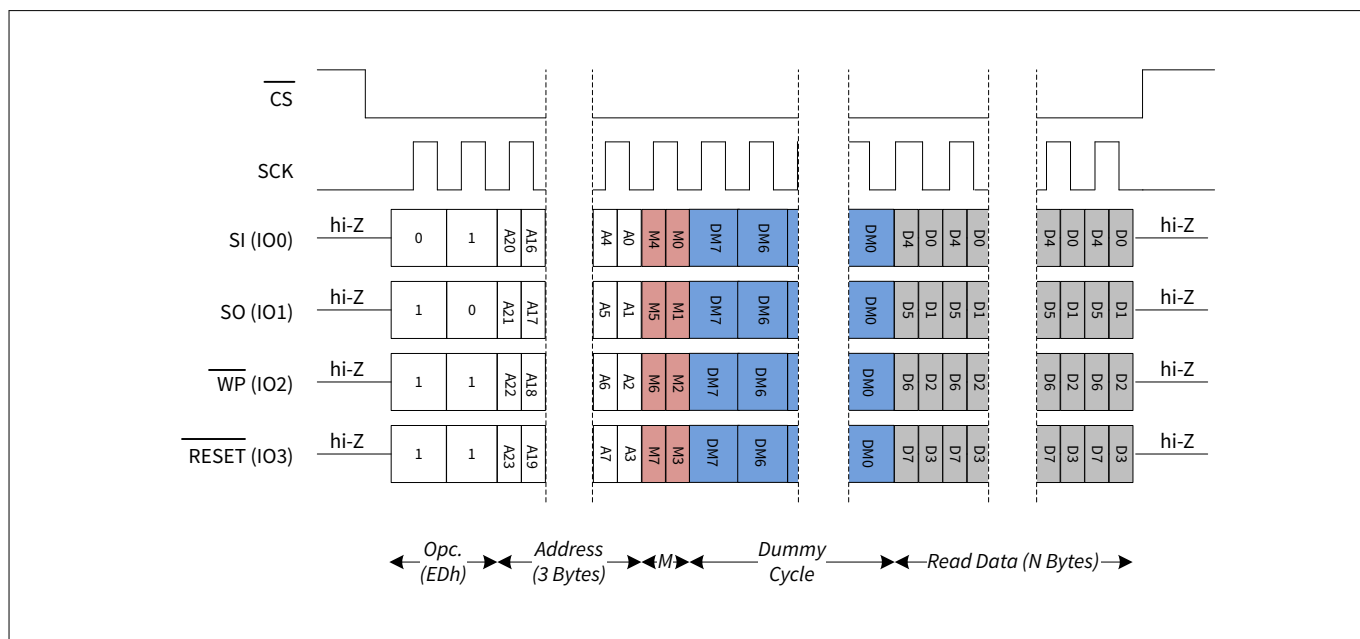
Figure 67 Quad I/O read in DDR (DDRQIOR) – in QPI mode
