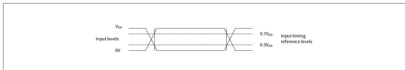
Figure 115 AC timing input voltage reference levels
