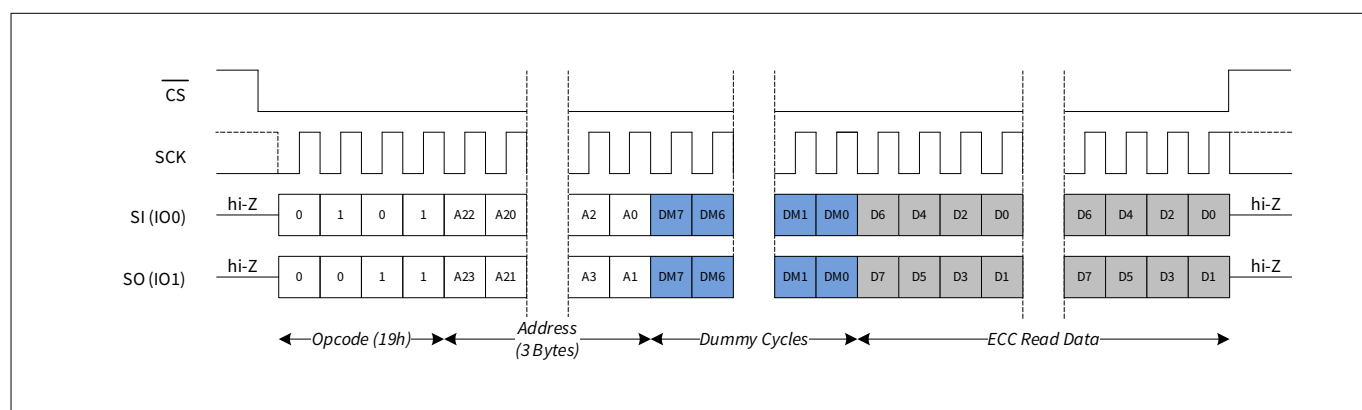
Figure 75 ECC read (ECCRD) in DPI mode
