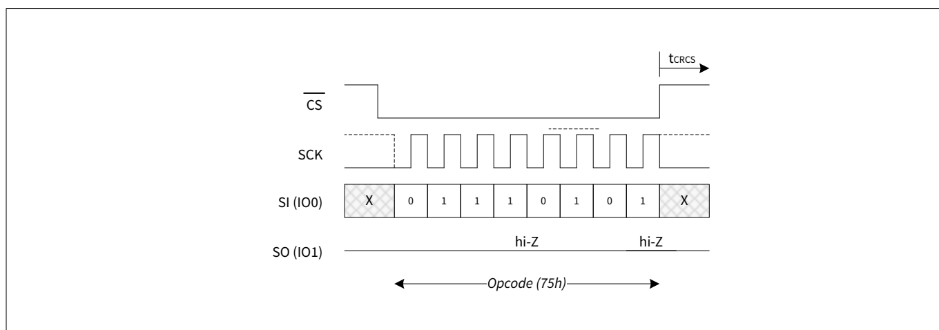
Figure 83 CRC suspend (EPCS) in SPI mode
