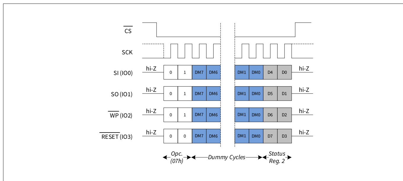
Figure 22 Read SR2 (RDSR2) in QPI mode
