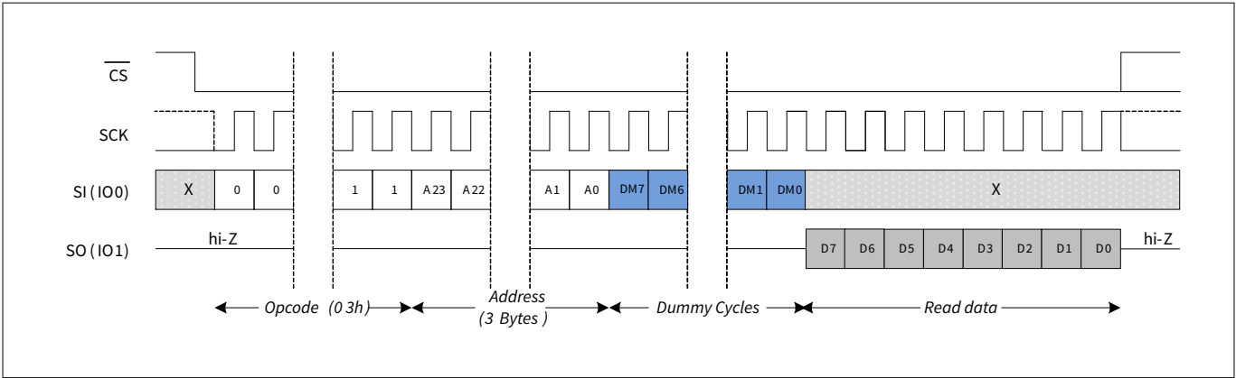
Figure 54 READ in SPI mode
