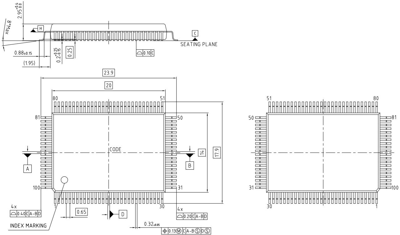
Figure 5. 100-lead QFP (20.00 × 14.00 × 3.35 mm) PQH100 package outline, Z8B00248915
