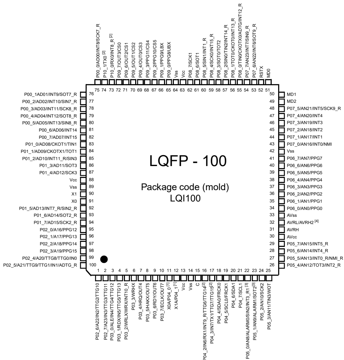
Figure 3. Pin assignment of CY96(F)34x (LQI100)
