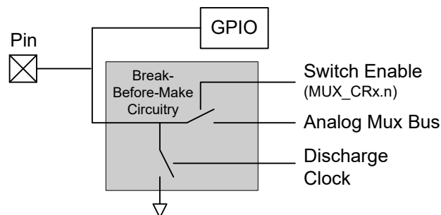
Figure 13-2. I/O Pin Configuration
