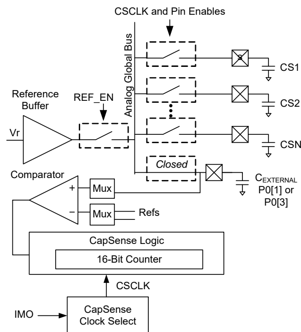
Figure 12-8. Negative Charge Integration Block Diagram
