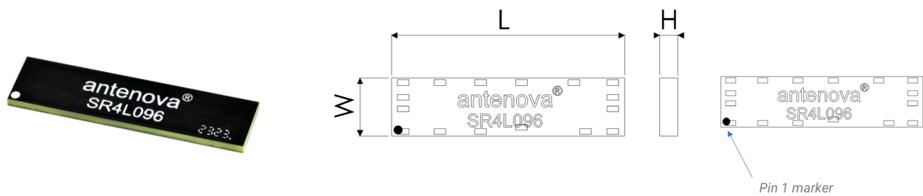
Top view
