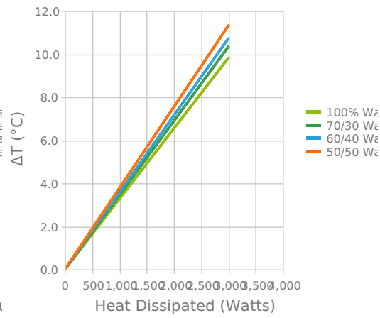
WL2000 Fluid Inlet/Outlet Temperature Differ @ Nominal Flow 4.4 L/min
