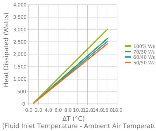
WL2000 Heat Dissipation 2000 Watt Requirement
