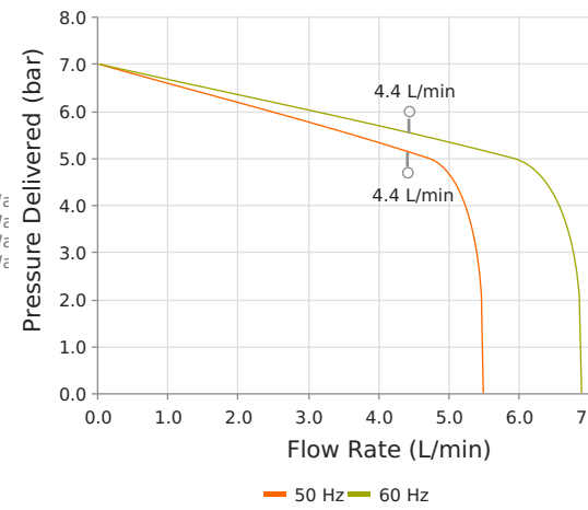
WL2000 - Pump Curve
