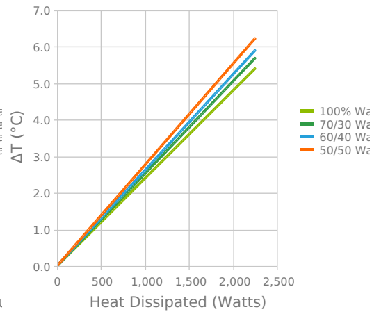
WL1500 Fluid Inlet/Outlet Temperature Differ @ Nominal Flow 6 L/min
