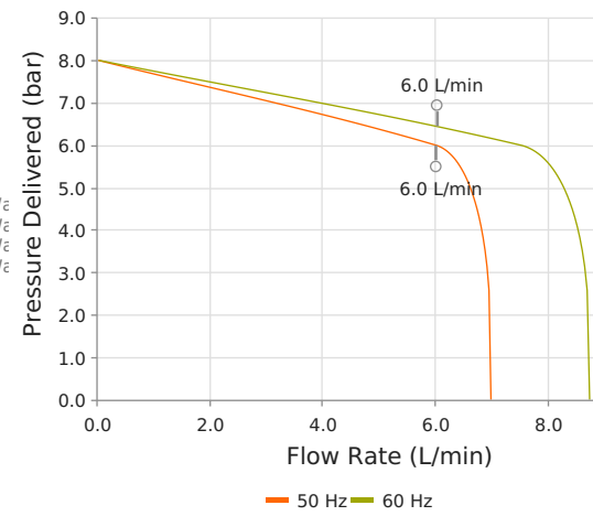
WL1500 - Pump Curve
