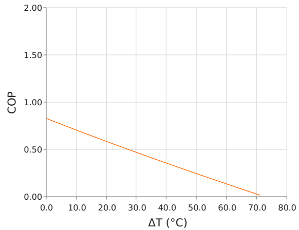
Coefficient of Performance ( COP = Q_c/P_{in} ) T_{hot} = 35\text{ }^{\circ}\text{C} | operating = 2.2 Amps
