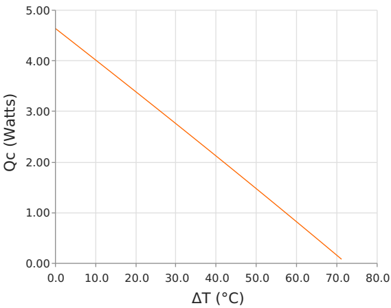
Heat Pumped at Cold Side ( Q_c ) T_{hot} = 35\text{ }^{\circ}\text{C} | operating = 2.2 Amps
