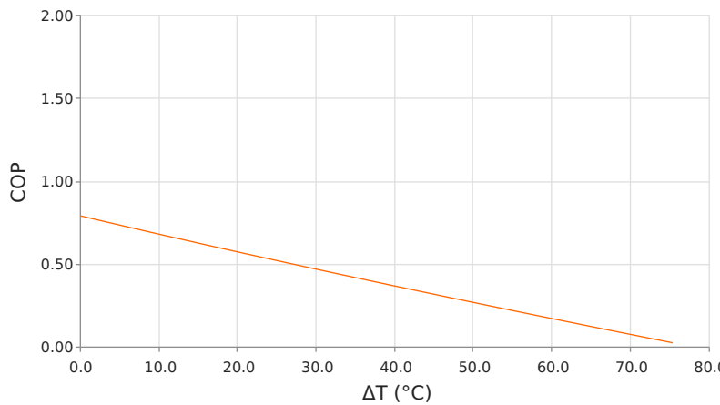
Coefficient of Performance (COP = Q_c/P_{in} ) T_{hot} = 50\text{ }^{\circ}\text{C} | I_{operating} = 10.5\text{ Amps}
