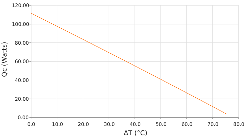
Heat Pumped at Cold Side ( Q_c ) T_{hot} = 50\text{ }^{\circ}\text{C} | I_{operating} = 10.5\text{ Amps}
