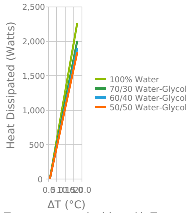
WL1500 Heat Dissipation 1500 Watt Requirement
