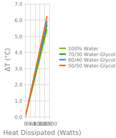
WL1500 Fluid Inlet/Outlet Temperature Difference (ΔT) @ Nominal Flow 6 L/min
