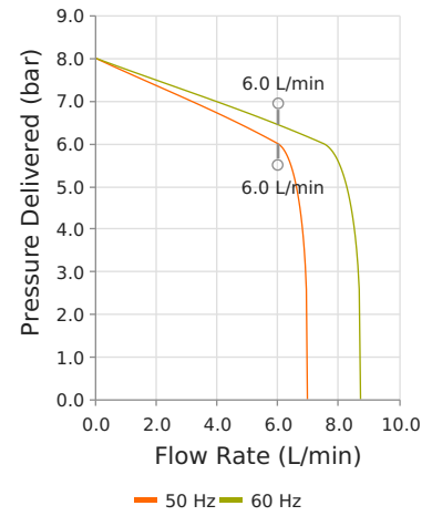
WL1500 - Pump Curve
