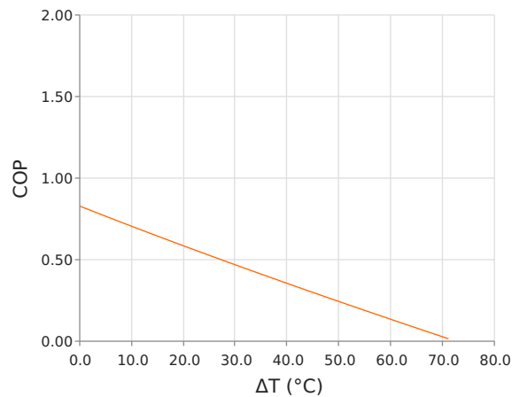
Coefficient of Performance ( COP = Q_c/P_{in} ) T_{hot} = 35\text{ }^{\circ}\text{C} | operating = 3.4 Amps
