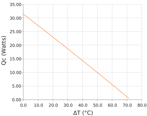
Heat Pumped at Cold Side ( Q_c ) T_{hot} = 35\text{ }^{\circ}\text{C} | operating = 3.4 Amps
