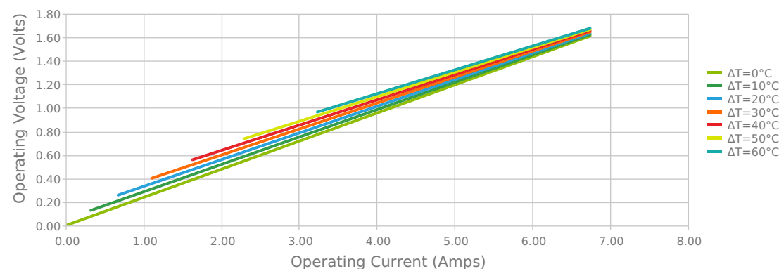
Current vs Voltage (I vs V) T_{hot} = 27\text{ °C}
