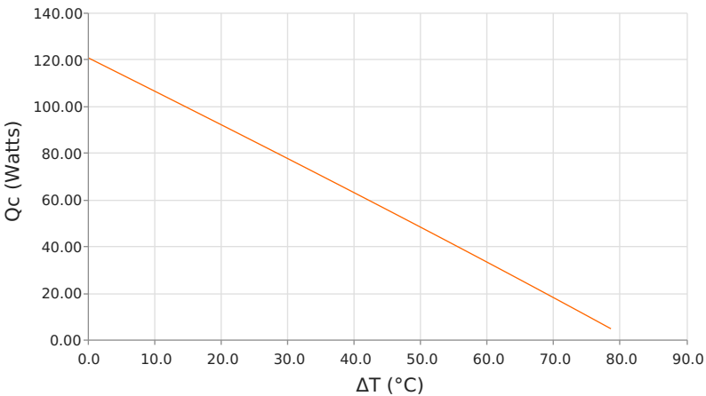
Heat Pumped at Cold Side ( Q_c ) T_{hot} = 50\text{ }^{\circ}\text{C} | operating = 10.7 Amps
