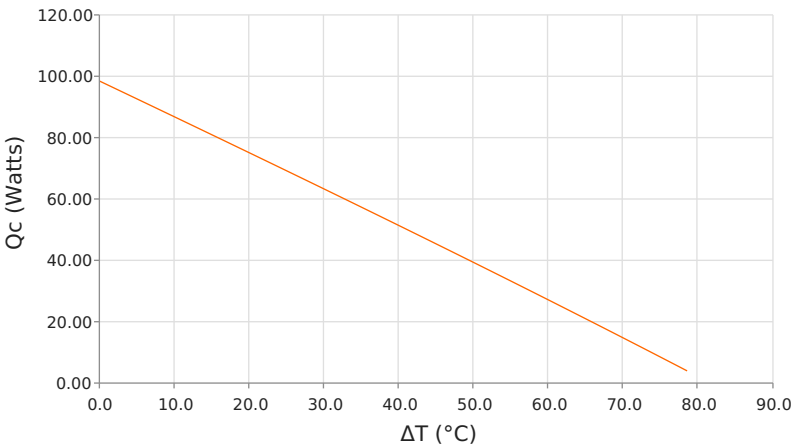
Heat Pumped at Cold Side ( Q_c ) T_{hot} = 50\text{ }^{\circ}\text{C} | operating = 9.5 Amps
