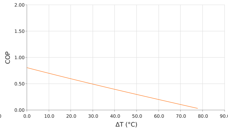
Coefficient of Performance (COP = Q_c/P_{in} ) T_{hot} = 50^\circ\text{C} | operating = 1 Amps
