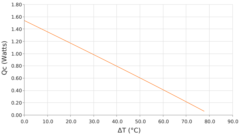
Heat Pumped at Cold Side ( Q_c ) T_{hot} = 50^\circ\text{C} | operating = 1 Amps
