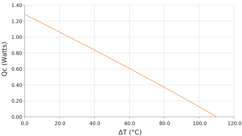
Heat Pumped at Cold Side ( Q_c ) T_{hot} = 35\text{ }^{\circ}\text{C} | operating = 1.5 Amps
