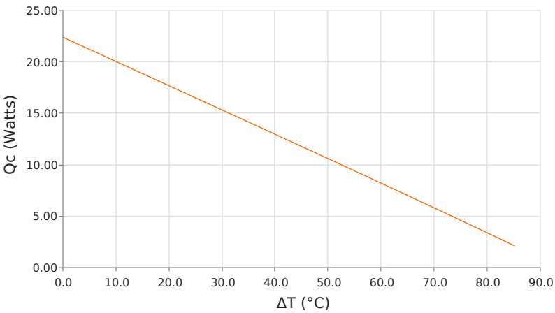
Heat Pumped at Cold Side ( Q_c ) T_{hot} = 85\text{ }^{\circ}\text{C} | operating = 7.5 Amps
