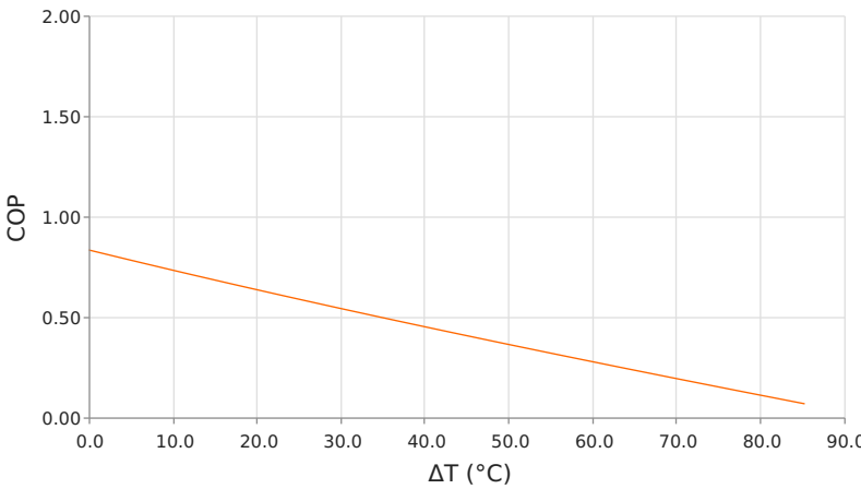
Coefficient of Performance (COP = Q_c/P_{in} ) T_{hot} = 85\text{ }^{\circ}\text{C} | operating = 7.5 Amps
