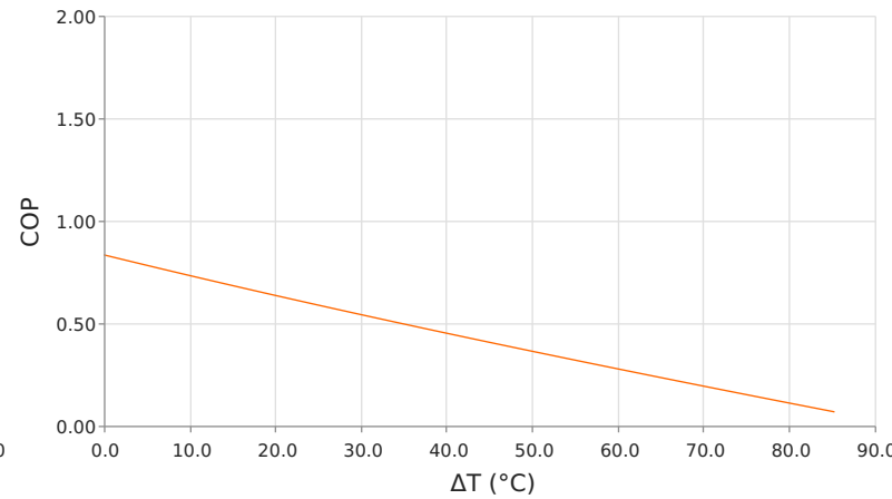
Coefficient of Performance (COP = Q_c/P_{in} ) T_{hot} = 85^\circ\text{C} | operating = 4.2 Amps
