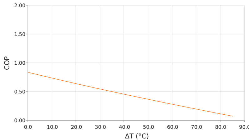
Coefficient of Performance (COP = Q_c/P_{in} ) T_{hot} = 85\text{ }^{\circ}\text{C} | I_{operating} = 11.9\text{ Amps}
