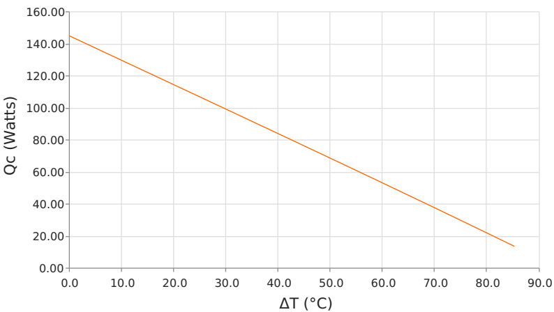
Heat Pumped at Cold Side ( Q_c ) T_{hot} = 85\text{ }^{\circ}\text{C} | I_{operating} = 11.9\text{ Amps}
