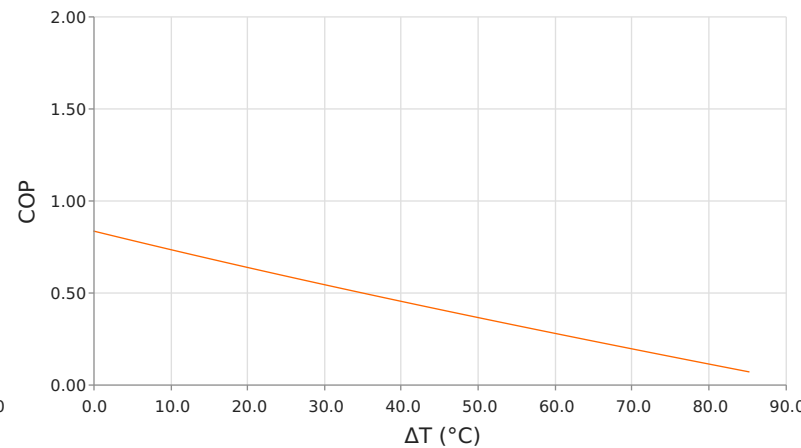
Coefficient of Performance (COP = Q_c/P_{in} ) T_{hot} = 85^\circ\text{C} | operating = 9.1 Amps
