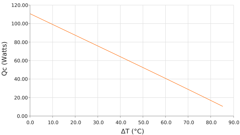
Heat Pumped at Cold Side ( Q_c ) T_{hot} = 85^\circ\text{C} | operating = 9.1 Amps
