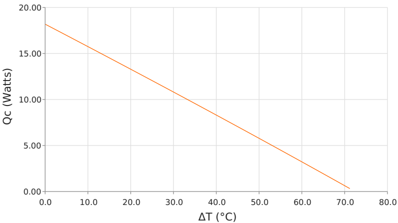
Heat Pumped at Cold Side ( Q_c ) T_{hot} = 35^\circ\text{C} | operating = 7.9 Amps
