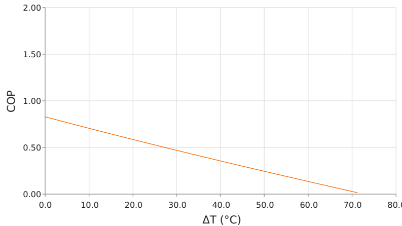
Coefficient of Performance (COP = Q_c/P_{in} ) T_{hot} = 35^\circ\text{C} | operating = 7.9 Amps
