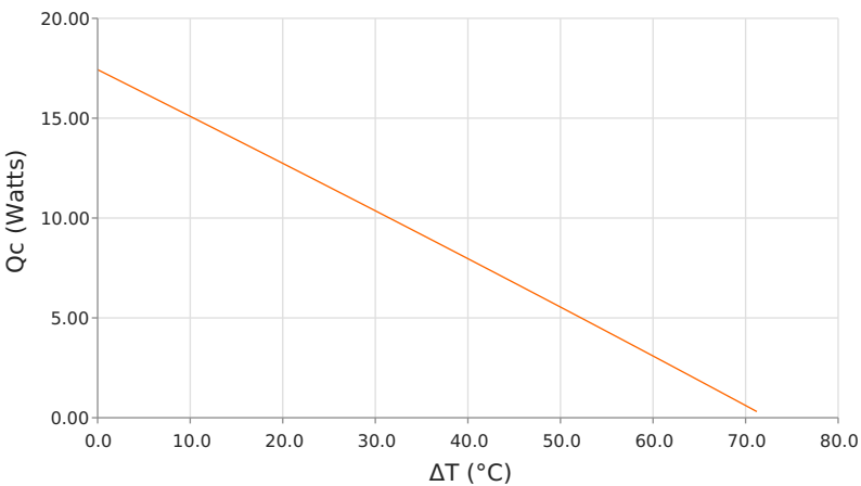
Heat Pumped at Cold Side ( Q_c ) T_{hot} = 35^\circ\text{C} | operating = 3.3 Amps
