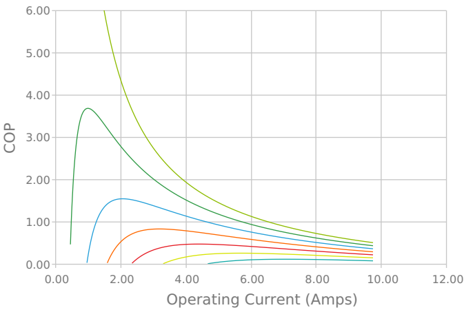
Coefficient of Performance ( COP = Q_c/P_{in} ) T_{hot} = 27^\circ C
