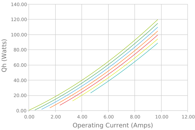
Total Heat Dissipated at Hot Side ( Q_h = Q_c + P_{in} ) T_{hot} = 27^\circ C
