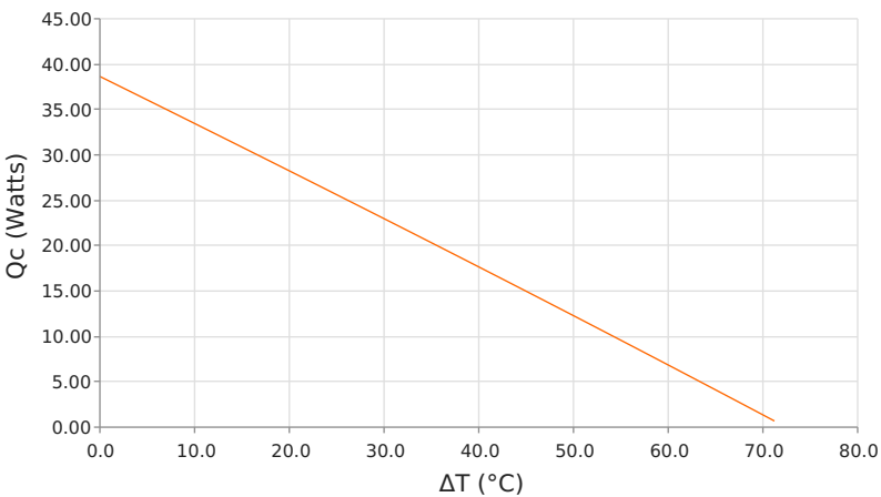
Heat Pumped at Cold Side ( Q_c ) T_{hot} = 35^\circ C | operating = 7.3 Amps
