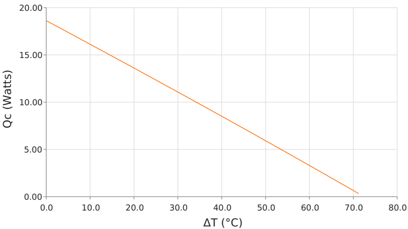
Heat Pumped at Cold Side ( Q_c ) T_{hot} = 35\text{ }^{\circ}\text{C} | operating = 2 Amps
