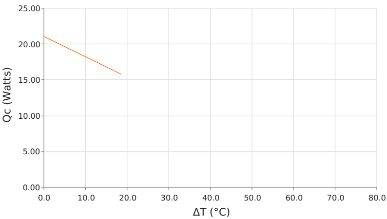
Heat Pumped at Cold Side ( Q_c ) T_{hot} = 35\text{ }^{\circ}\text{C} | operating = 2.2 Amps
